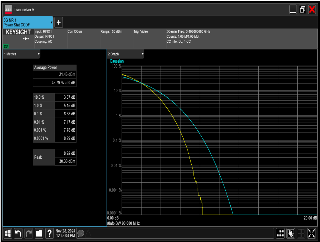
n77(3450-3550) SCS=30kHz DFT_QAM256 BW=90MHz Channel=633000 RB=240@0
