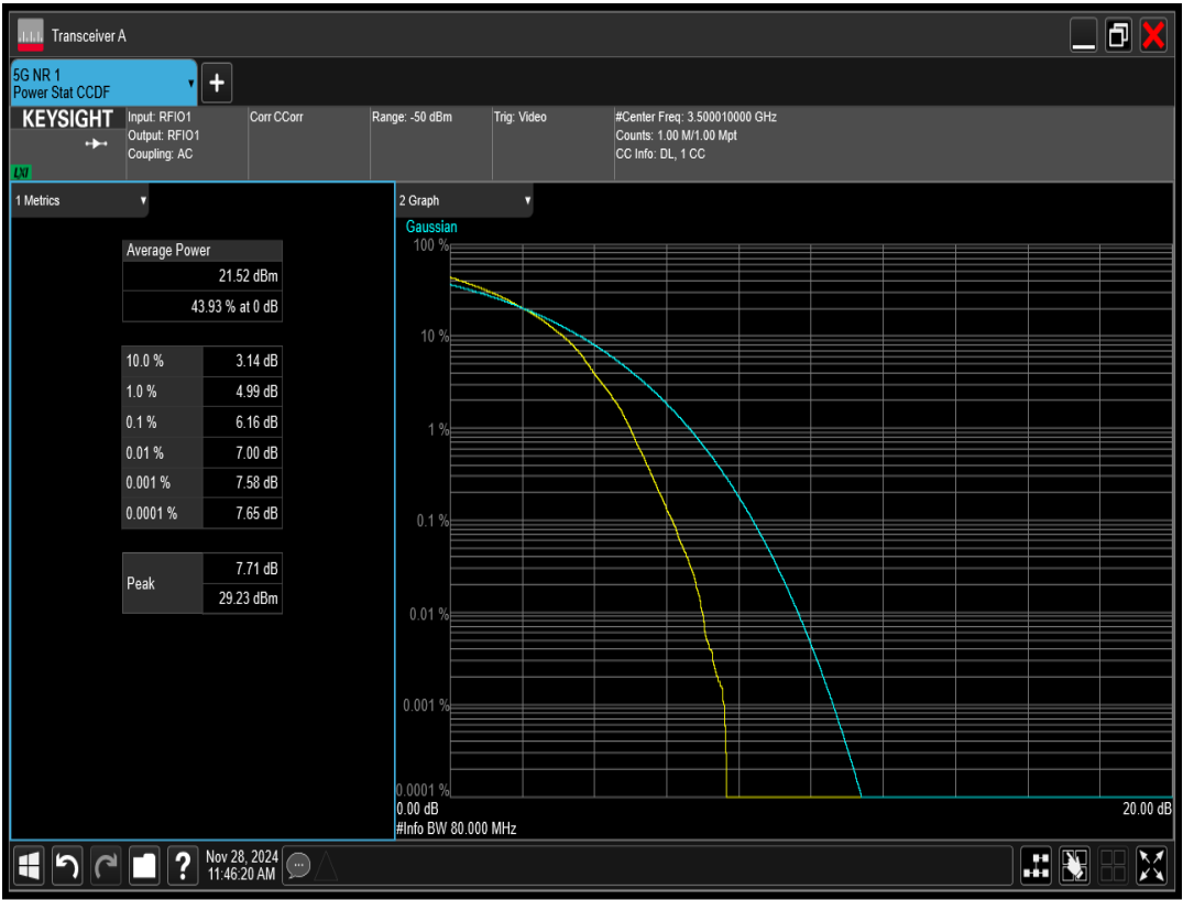
n77(3450-3550) SCS=30kHz DFT_QAM256 BW=80MHz Channel=633334 RB=216@0
