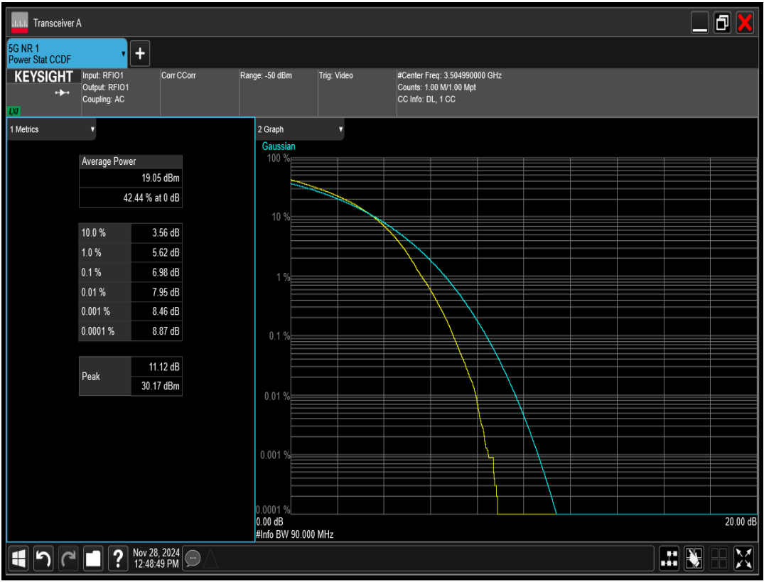
n77(3450-3550) SCS=30kHz DFT_QAM256 BW=90MHz Channel=633666 RB=240@0
