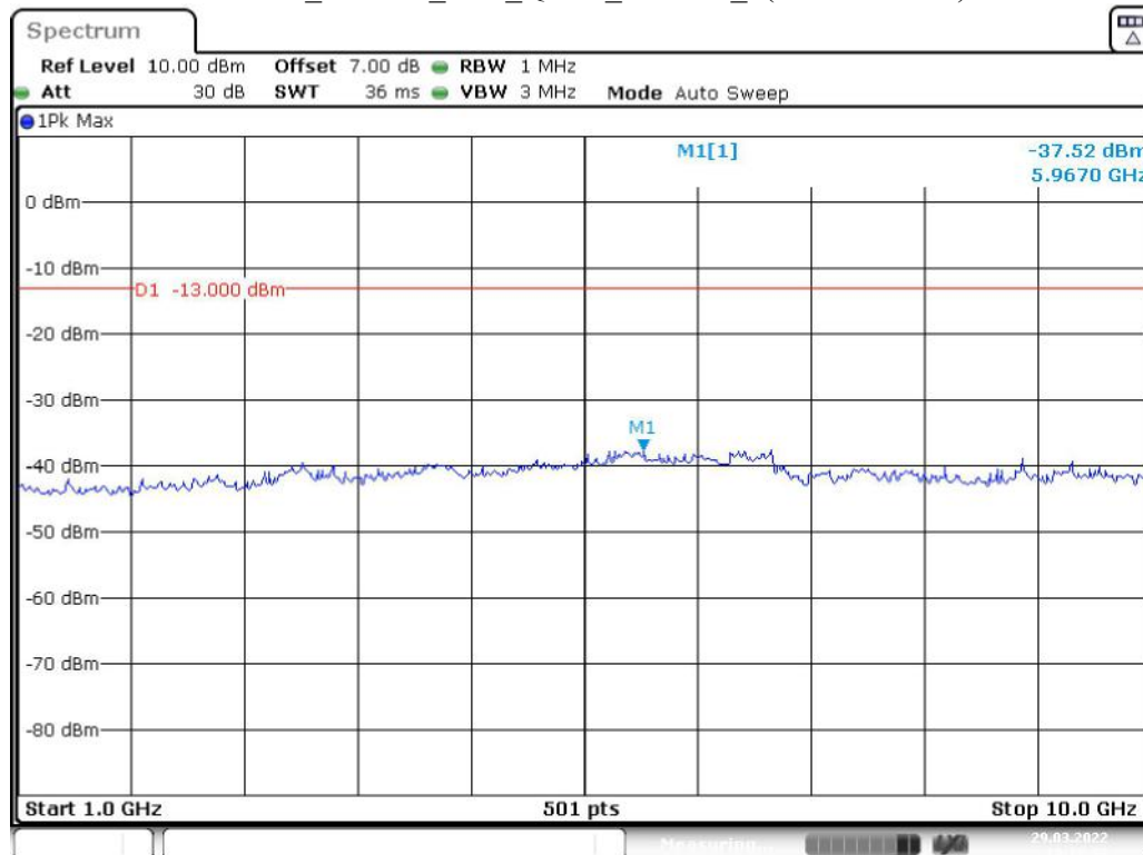
Band 12_10 MHz_Low_QPSK_RB50#0_2(1GHz-10GHz)
