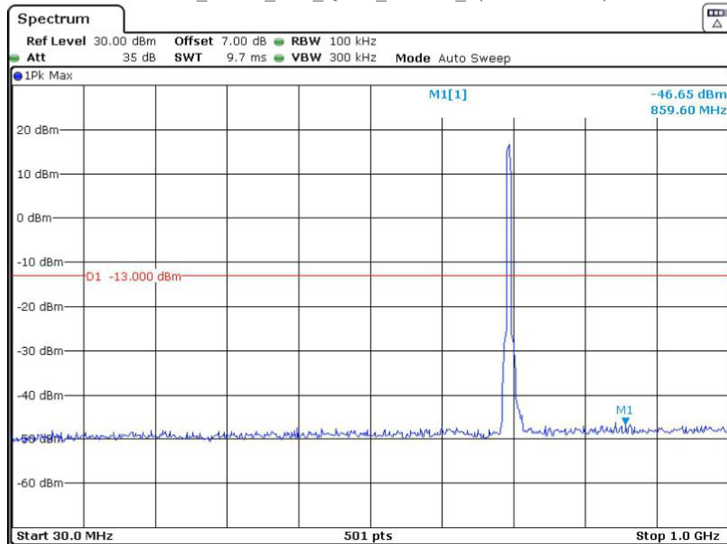
Band 12_5 MHz_Low_QPSK_RB25#0_1(30MHz-1GHz)
