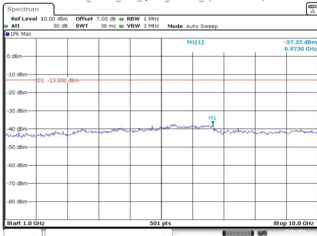
Band 12_5 MHz_Low_QPSK_RB25#0_2(1GHz-10GHz)
