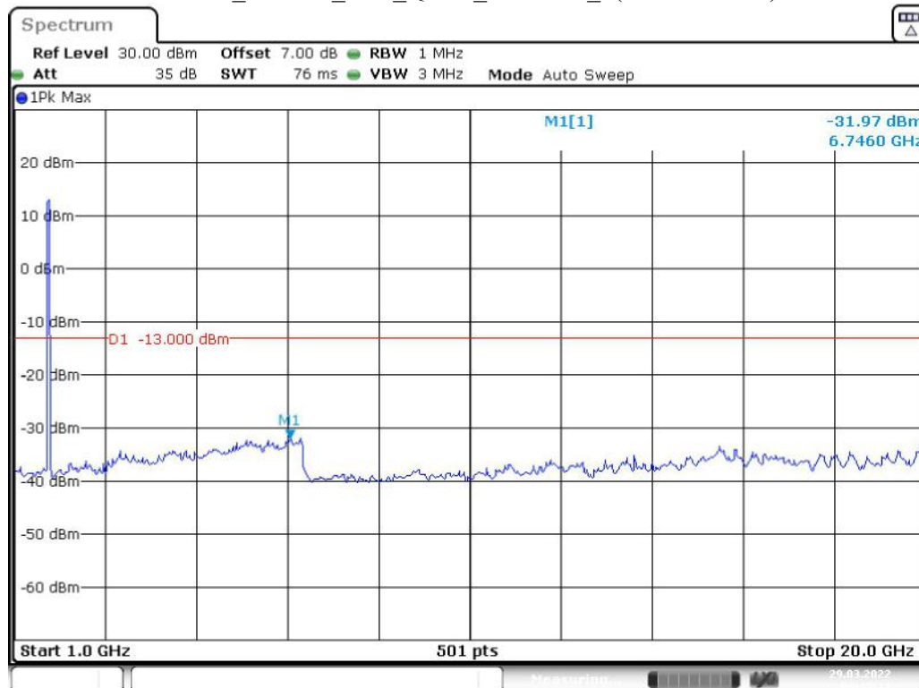
Band 4_20 MHz_Low_QPSK_RB100#0_2(1GHz-20GHz)
