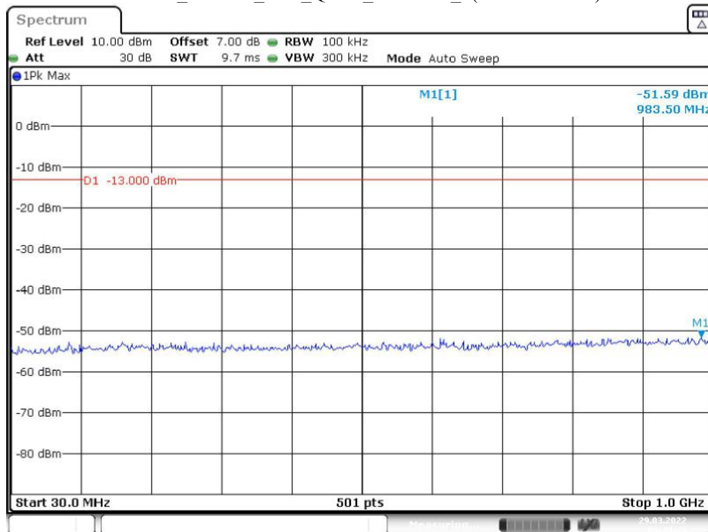
Band 4_20 MHz_Low_QPSK_RB100#0_1(30MHz-1GHz)
