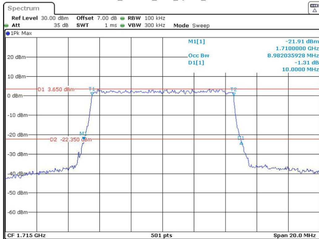
Band 66_10 MHz_Low_QPSK_RB50#0
