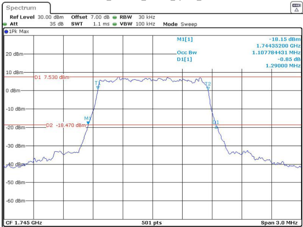
Band 66_1.4 MHz_Middle_QPSK_RB6#0
