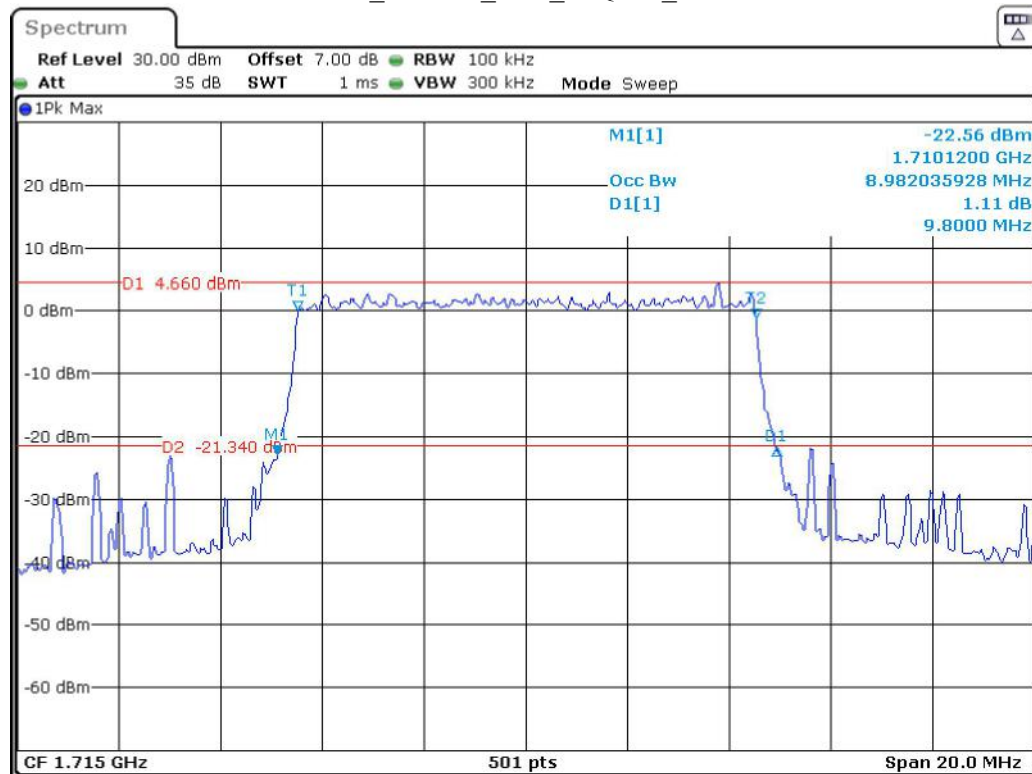
Band 66_10 MHz_Low_16QAM_RB50#0
