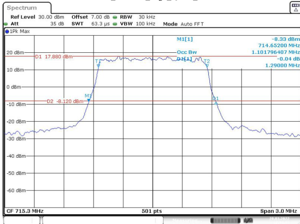
Band 12_1.4 MHz_High_QPSK_RB6#0
