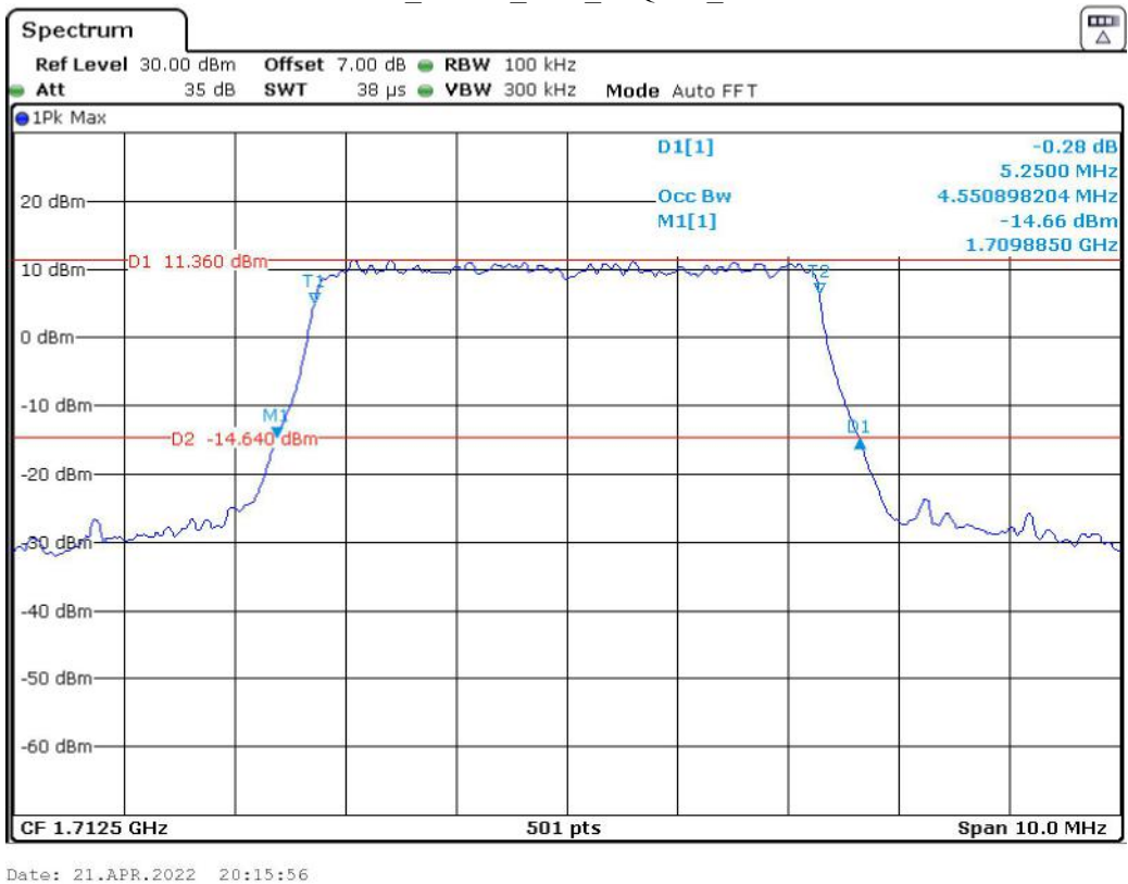
Band 66_5 MHz_Low_16QAM_RB25#0
