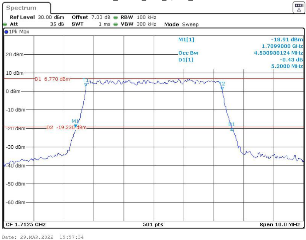
Band 66_5 MHz_Low_QPSK_RB25#0
