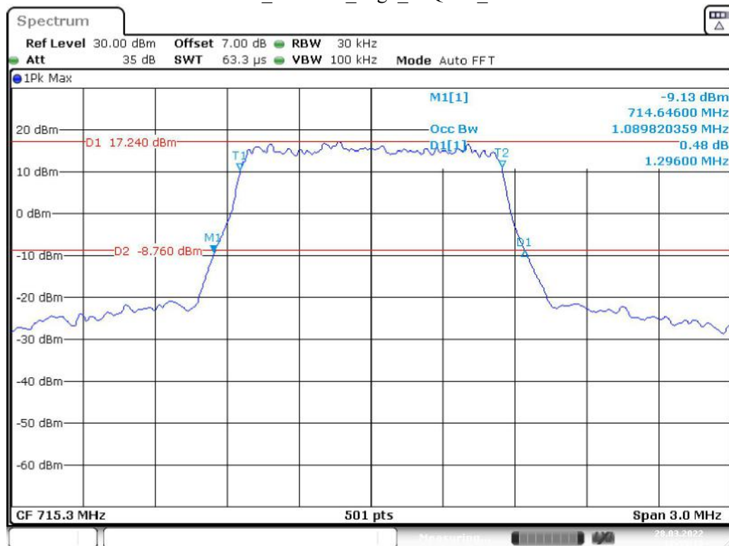
Band 12_1.4 MHz_High_16QAM_RB6#0
