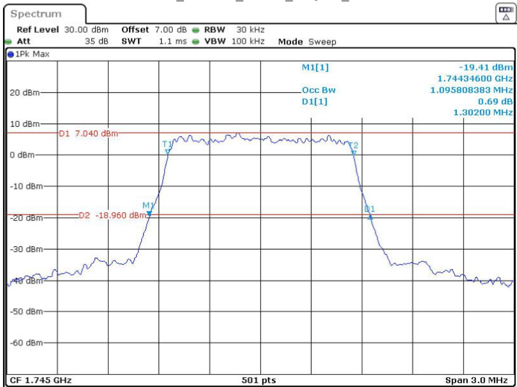
Band 66_1.4 MHz_Middle_16QAM_RB6#0
