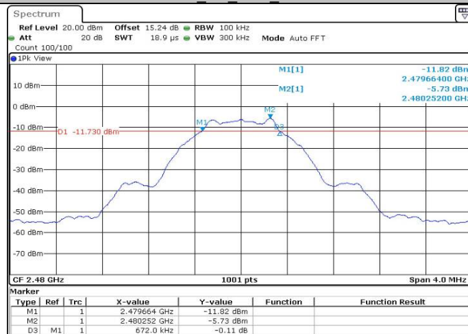
BLE_1M_Ant1_2480
