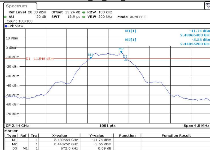
BLE_1M_Ant1_2440
