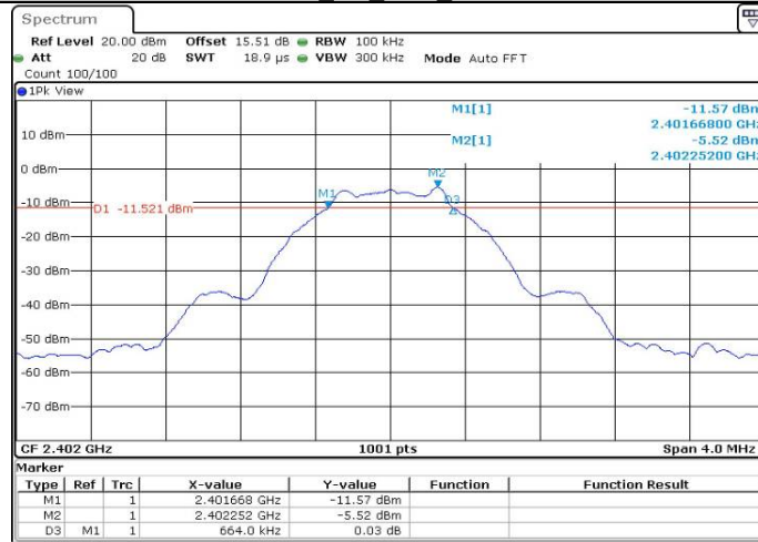
BLE_1M_Ant1_2402
