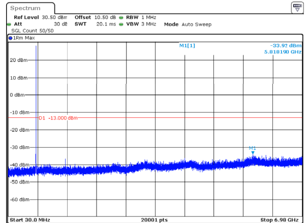
n71_5MHz_15kHz_680.5MHz_DFT-s-OFDM QPSK_RB1@24 -33.92dBm
