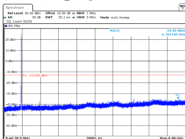
n71_10MHz_15kHz_680.5MHz_DFT-s-OFDM QPSK_RB1@51 -34.82dBm
