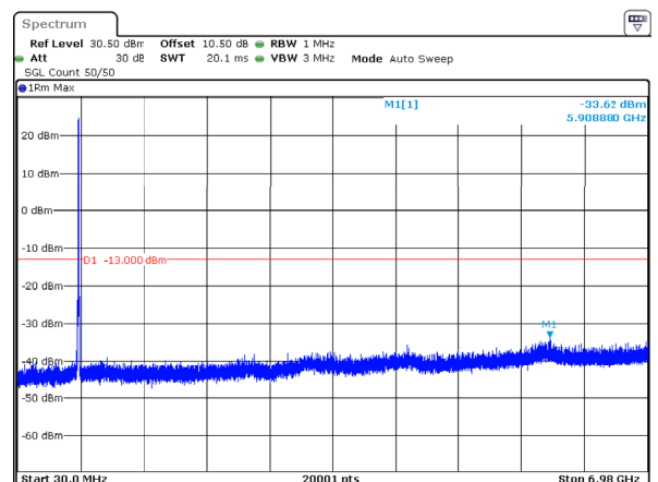
n71_5MHz_15kHz_695.5MHz_DFT-s-OFDM QPSK_RB25@0 -33.62dBm
