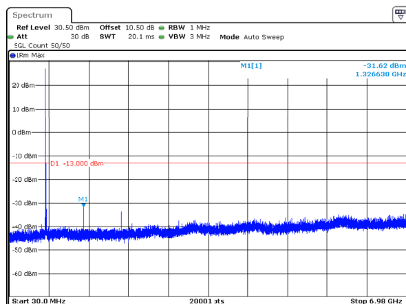
n71_10MHz_15kHz_668MHz_DFT-s-OFDM QPSK_RB1@0 -31.62dBm
