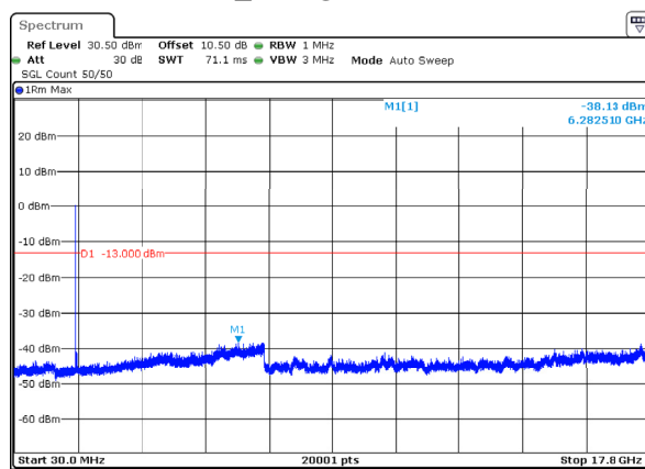
n66_40MHz_15kHz_1745MHz_DFT-s-OFDM QPSK_RB1@0 -38.13dBm
