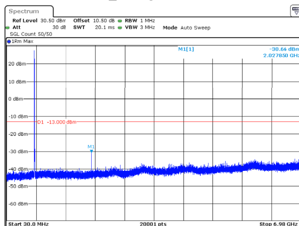
n71_10MHz_15kHz_680.5MHz_DFT-s-OFDM QPSK_RB1@0 -30.66dBm
