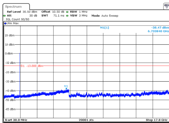
n66_40MHz_15kHz_1730MHz_DFT-s-OFDM QPSK_RB1@0 -38.47dBm
