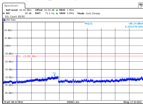
n66_40MHz_15kHz_1730MHz_DFT-s-OFDM QPSK_RB216@0 -38.14dBm
