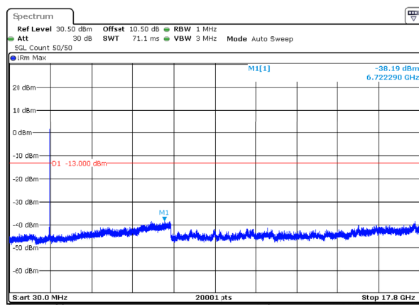
n66_40MHz_15kHz_1745MHz_DFT-s-OFDM QPSK_RB1@215 -38.19dBm
