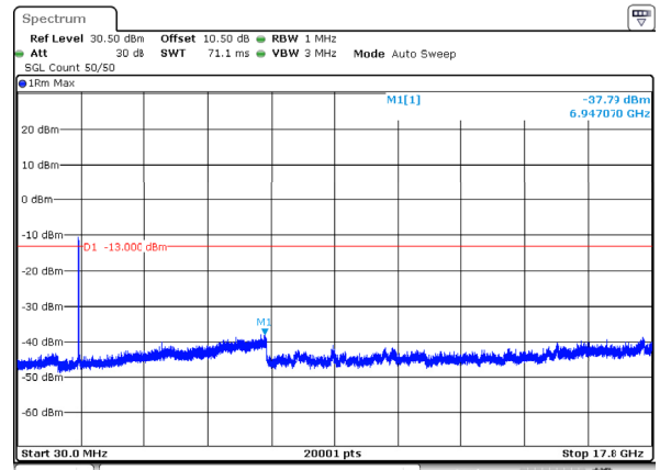
n66_30MHz_15kHz_1725MHz_DFT-s-OFDM QPSK_RB160@0 -37.79dBm
