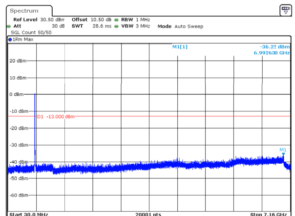
n12_10MHz_15kHz_704MHz_DFT-s-OFDM QPSK_RB50@0 -36.22dBm
