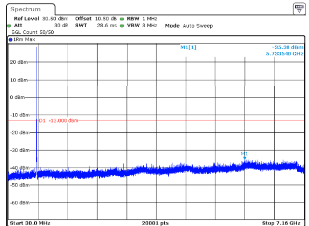
n12_10MHz_15kHz_704MHz_DFT-s-OFDM QPSK_RB1@0 -35.38dBm
