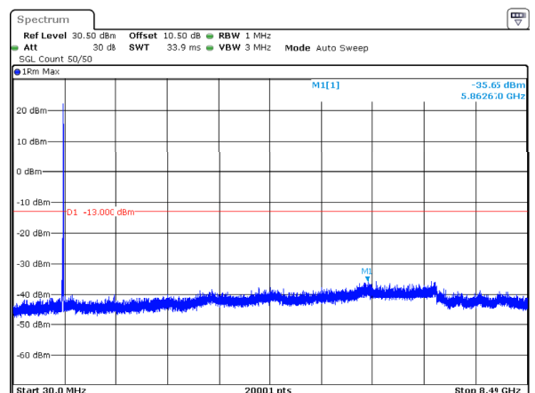
n5_20MHz_15kHz_839MHz_DFT-s-OFDM QPSK_RB1@105 -35.65dBm
