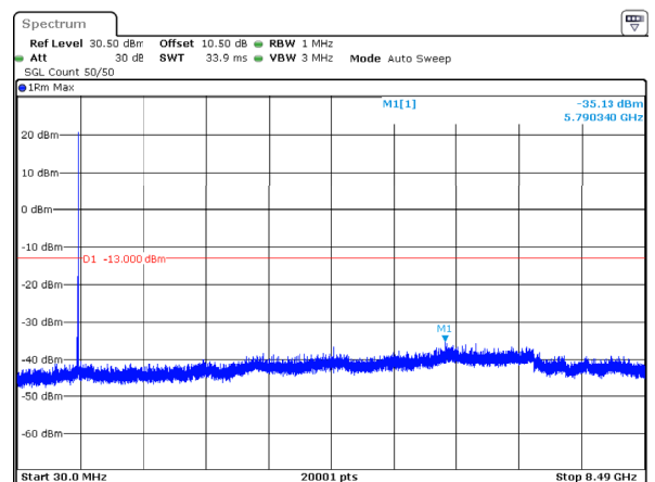
n5_20MHz_15kHz_834MHz_DFT-s-OFDM QPSK_RB1@105 -35.13dBm
