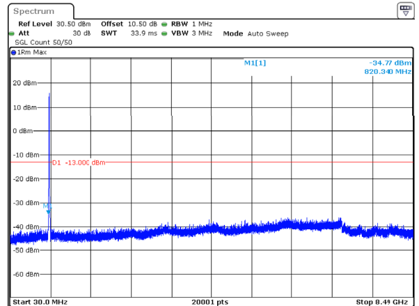
n5_20MHz_15kHz_839MHz_DFT-s-OFDM QPSK_RB100@0 -34.77dBm
