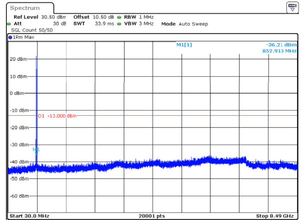
n5_15MHz_15kHz_841.5MHz_DFT-s-OFDM QPSK_RB1@78 -36.21dBm
