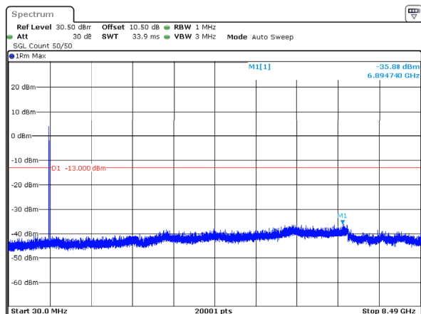
n5_5MHz_15kHz_846.5MHz_DFT-s-OFDM QPSK_RB1@24 -35.88dBm
