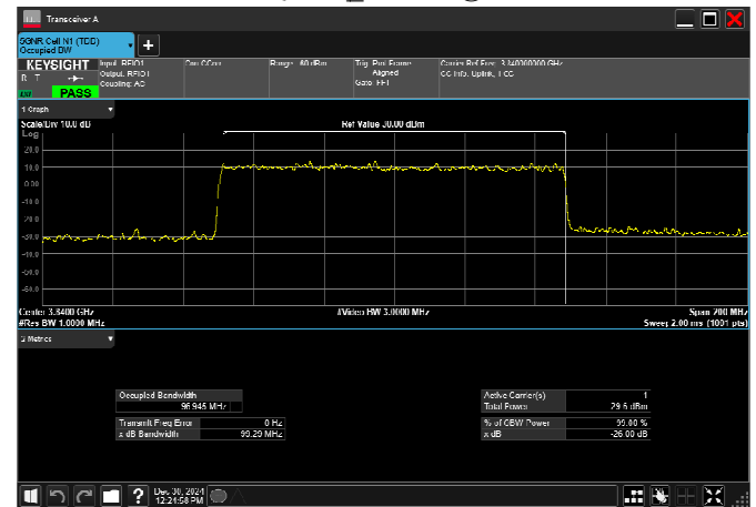
n77_3_100MHz_30kHz_3840MHz_DFT-s-OFDM 64 QAM_RB270@0
