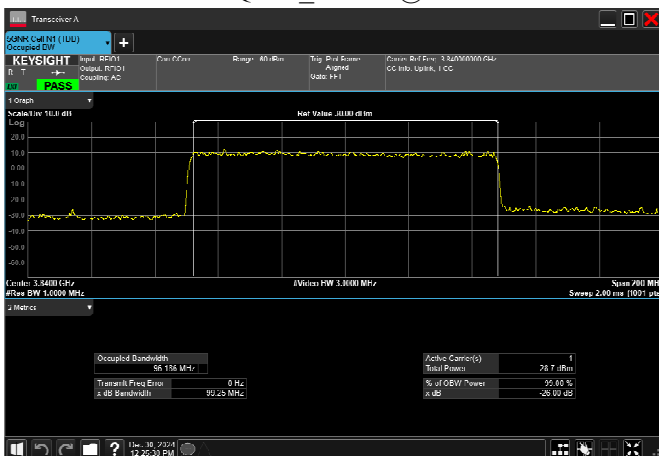
n77_3_100MHz_30kHz_3840MHz_DFT-s-OFDM 16 QAM_RB270@0
