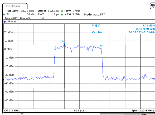
n77_1_40MHz_30kHz_3500MHz_DFT-s-OFDM 256 QAM_RB100@0 Occupied Bandwidth
