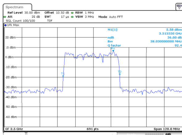
n77_1_40MHz_30kHz_3500MHz_DFT-s-OFDM 256 QAM_RB100@0 26 dB Emission Bandwidth
