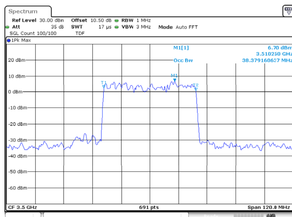
n77_1_40MHz_30kHz_3500MHz_CP-OFDM QPSK_RB106@0 Occupied Bandwidth
