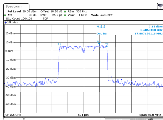
n77_1_20MHz_30kHz_3500MHz_DFT-s-OFDM QPSK_RB50@0 Occupied Bandwidth 26 dB Emission Bandwidth
