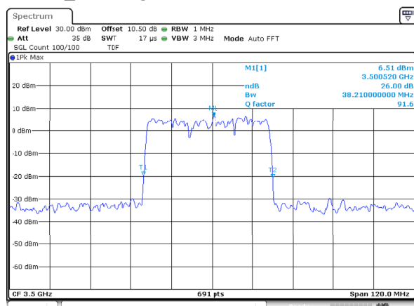
n77_1_40MHz_30kHz_3500MHz_DFT-s-OFDM 64 QAM_RB100@0 26 dB Emission Bandwidth
