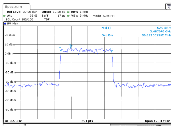
n77_1_40MHz_30kHz_3500MHz_DFT-s-OFDM 64 QAM_RB100@0 Occupied Bandwidth
