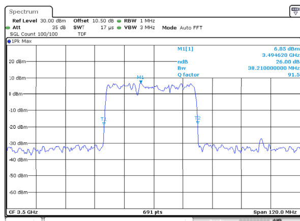
n77_1_40MHz_30kHz_3500MHz_DFT-s-OFDM 16 QAM_RB100@0 26 dB Emission Bandwidth
