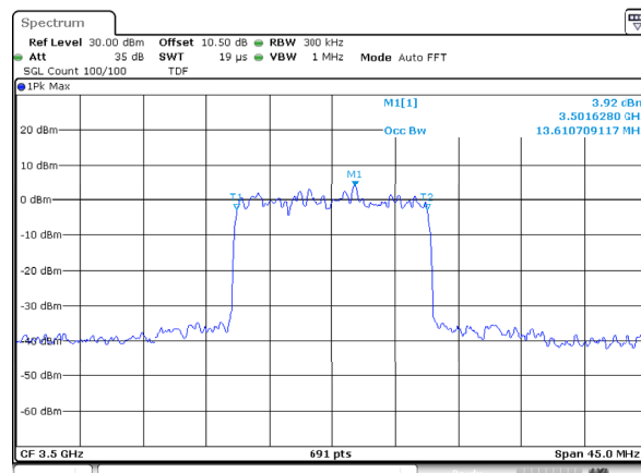
n77_1_15MHz_30kHz_3500MHz_CP-OFDM 256 QAM_RB38@0 Occupied Bandwidth
