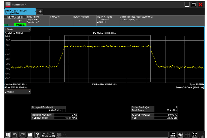
n71_5MHz_15kHz_680.5MHz_CP-OFDM 16 QAM_RB25@0
