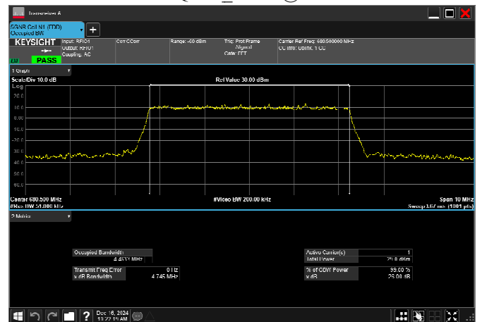
n71_5MHz_15kHz_680.5MHz_DFT-s-OFDM 16 QAM_RB25@0
