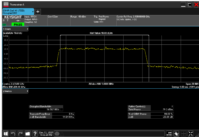
n7_15MHz_15kHz_2535MHz_CP-OFDM QPSK_RB79@0
