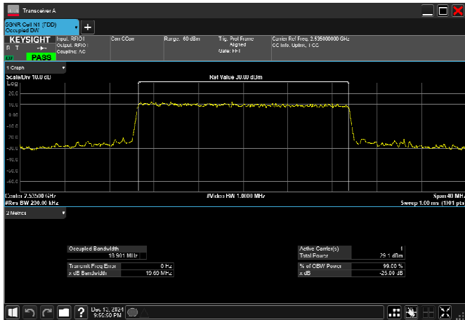
n7_20MHz_15kHz_2535MHz_CP-OFDM 16 QAM_RB106@0
