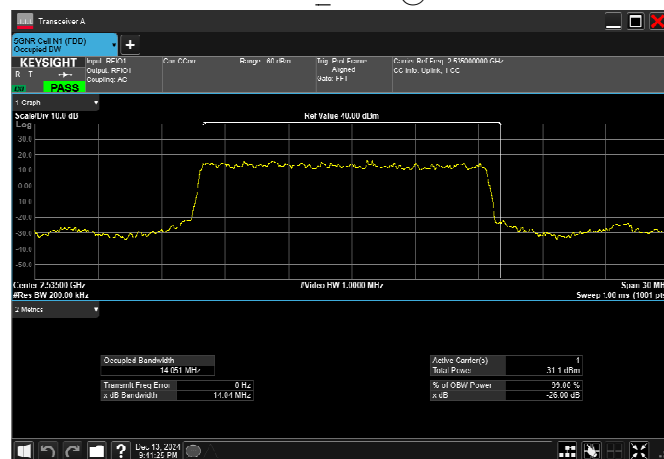
n7_15MHz_15kHz_2535MHz_DFT-s-OFDM 16 QAM RB75@0
