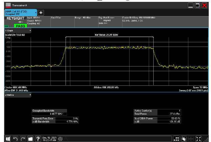
n71_5MHz_15kHz_680.5MHz_CP-OFDM 256 QAM_RB25@0
