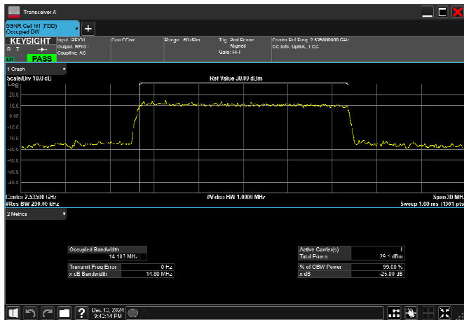
n7_15MHz_15kHz_2535MHz_CP-OFDM 64 QAM_RB79@0
