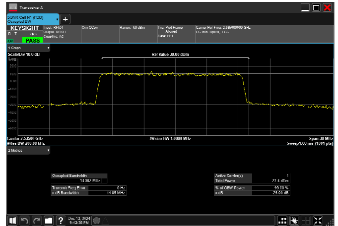
n7_15MHz_15kHz_2535MHz_CP-OFDM 16 QAM_RB79@0
