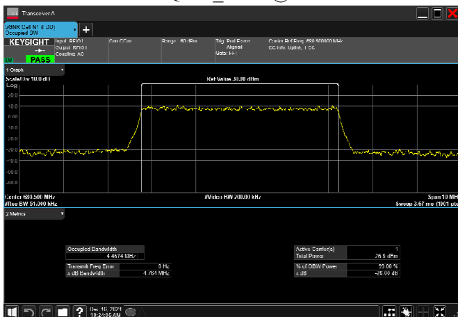
n71_5MHz_15kHz_680.5MHz_CP-OFDM 64 QAM_RB25@0
