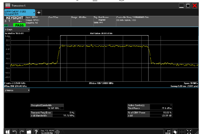
n7_15MHz_15kHz_2535MHz_CP-OFDM 256 QAM_RB79@0
