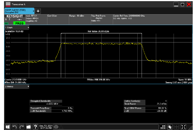
n7_5MHz_15kHz_2535MHz_CP-OFDM 16 QAM_RB25@0
