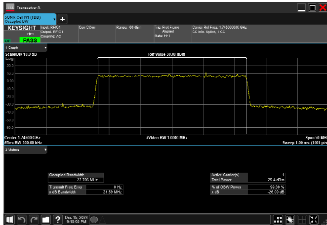
n66_25MHz_15kHz_1745MHz_CP-OFDM 256 QAM_RB133@0
