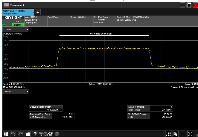
n66_30MHz_15kHz_1745MHz_DFT-s-OFDM QPSK_RB160@0
