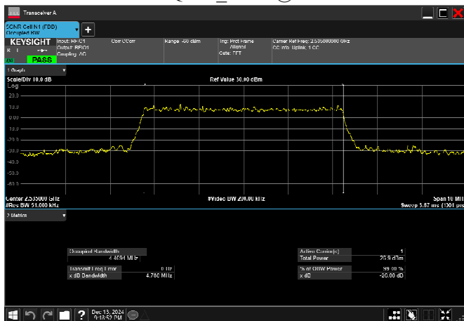
n7_5MHz_15kHz_2535MHz_CP-OFDM 64 QAM_RB25@0
