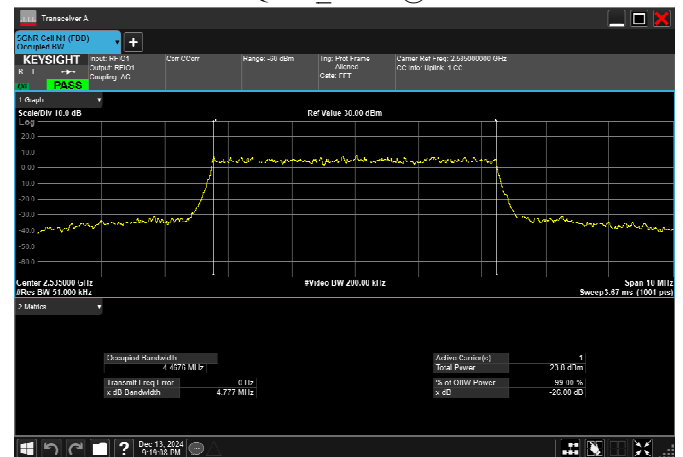
n7_5MHz_15kHz_2535MHz_CP-OFDM 256 QAM_RB25@0
