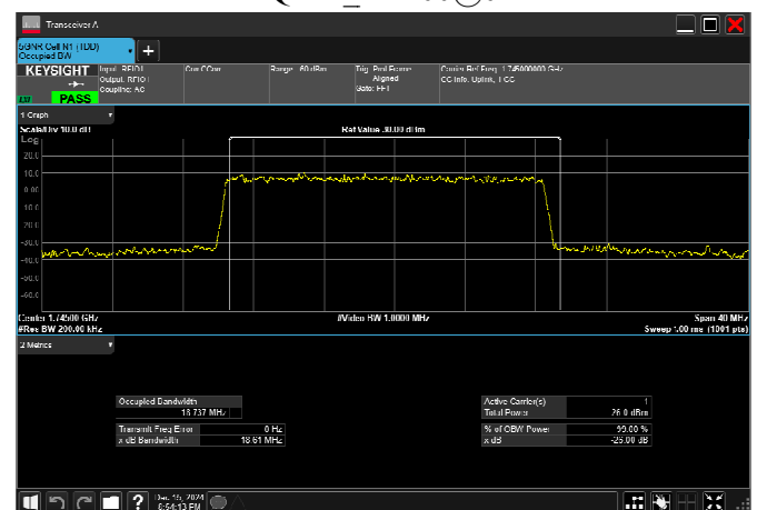
n66_20MHz_15kHz_1745MHz_DFT-s-OFDM 16 QAM_RB100@0
