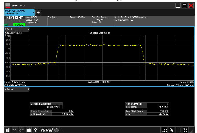
n66_15MHz_15kHz_1745MHz_CP-OFDM QPSK_RB79@0
