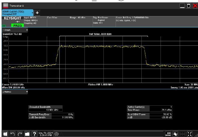
n66_15MHz_15kHz_1745MHz_DFT-s-OFDM 256 QAM_RB75@0
