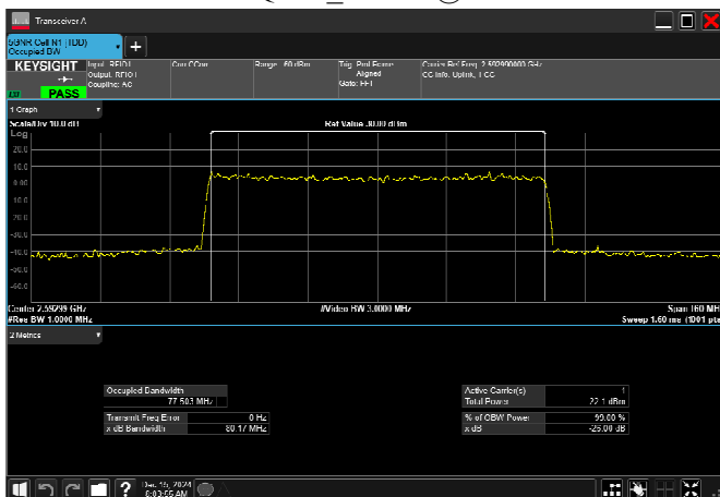
n41_80MHz_30kHz_2592.99MHz_CP-OFDM 64 QAM_RB217@0
