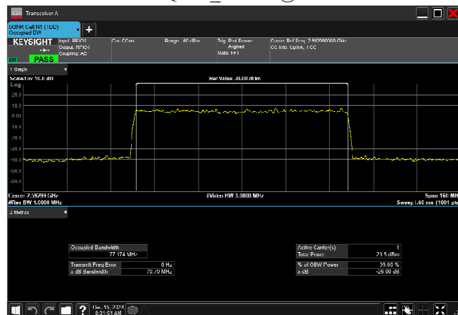
n41_80MHz_30kHz_2592.99MHz_DFT-s-OFDM 16 QAM RB216@0
