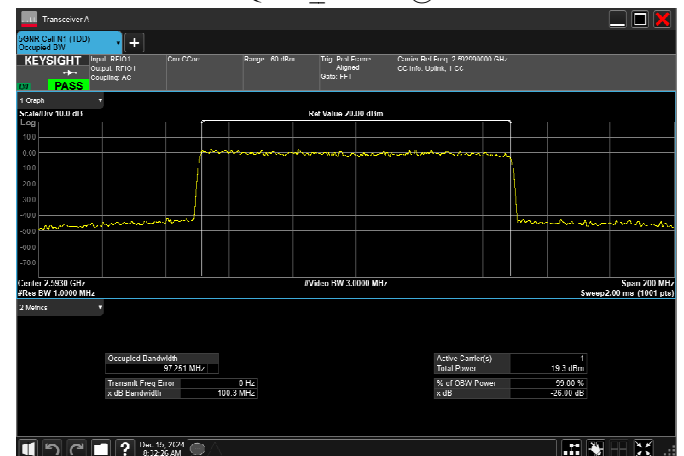
n41_100MHz_30kHz_2592.99MHz_CP-OFDM 256 QAM_RB273@0
