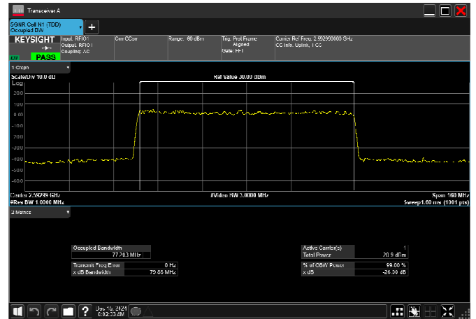
n41_80MHz_30kHz_2592.99MHz_CP-OFDM 16 QAM_RB217@0
