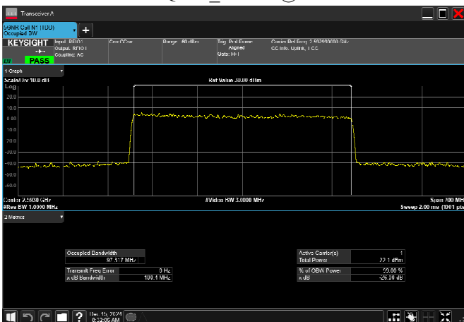
n41_100MHz_30kHz_2592.99MHz_CP-OFDM 64 QAM_RB273@0
