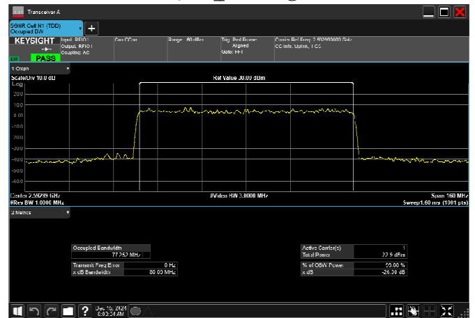
n41_80MHz_30kHz_2592.99MHz_CP-OFDM 256 QAM_RB217@0
