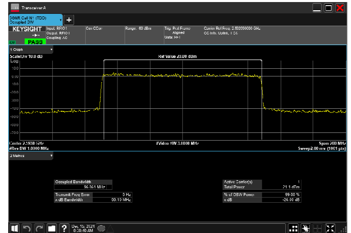
n41_100MHz_30kHz_2592.99MHz_CP-OFDM 16 QAM_RB273@0
