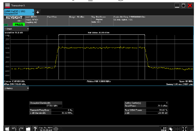
n38_40MHz_30kHz_2595MHz_CP-OFDM 256 QAM_RB106@0
