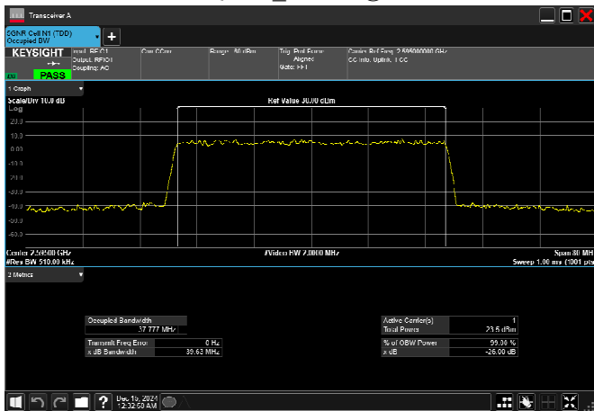
n38_40MHz_30kHz_2595MHz_CP-OFDM 64 QAM_RB106@0
