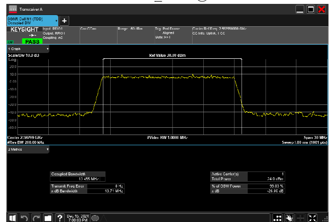
n41_15MHz_30kHz_2592.99MHz_DFT-s-OFDM 16 QAM_RB36@0
