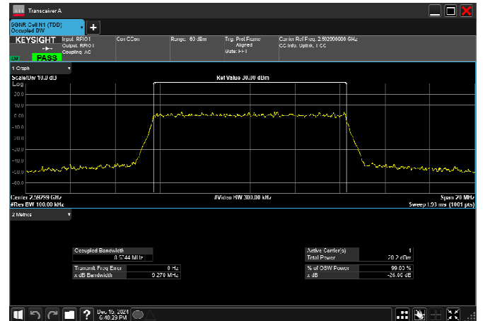
n41_15MHz_30kHz_2592.99MHz_DFT-s-OFDM \pi/2 BPSK_RB36@0
