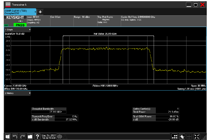
n38_40MHz_30kHz_2595MHz_CP-OFDM 16 QAM_RB106@0
