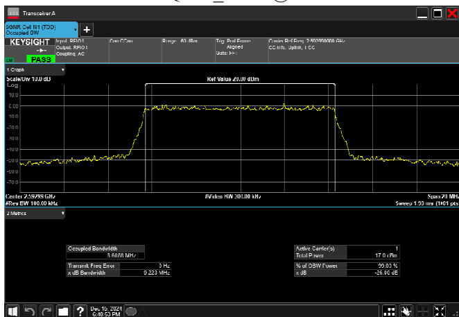
n41_15MHz_30kHz_2592.99MHz_DFT-s-OFDM QPSK_RB36@0
