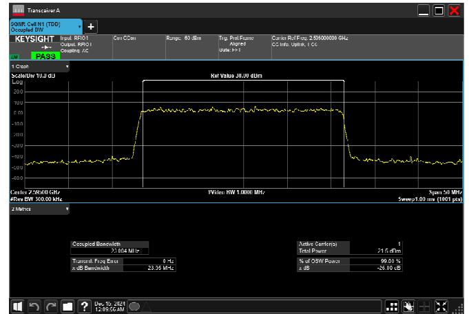
n38_25MHz_30kHz_2595MHz_CP-OFDM 16 QAM_RB65@0
