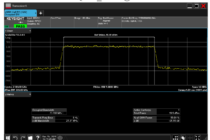
n38_25MHz_30kHz_2595MHz_CP-OFDM 256 QAM_RB65@0
