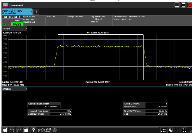
n38_25MHz_30kHz_2595MHz_CP-OFDM 64 QAM_RB65@0
