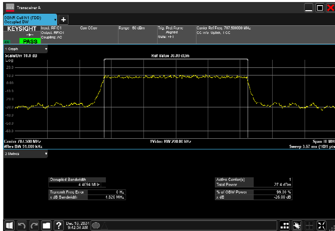
n12_5MHz_15kHz_707.5MHz_CP-OFDM 256 QAM_RB25@0
