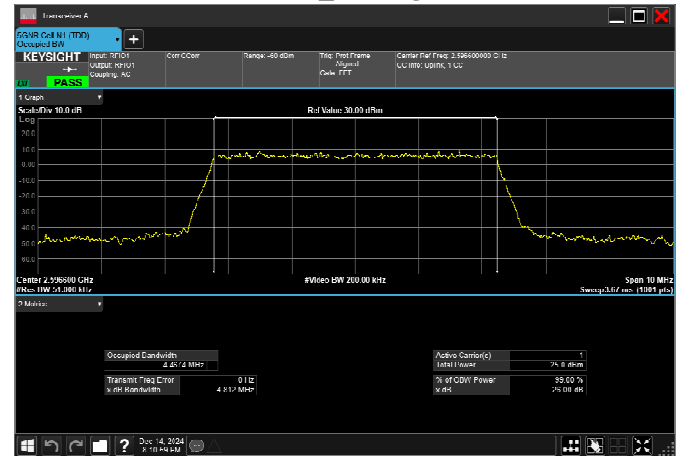
n38_5MHz_15kHz_2595MHz_DFT-s-OFDM 16 QAM_RB25@0
