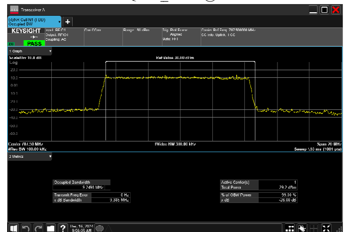
n12_10MHz_15kHz_707.5MHz_DFT-s-OFDM 16 QAM_RB50@0
