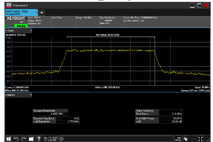
n38_5MHz_15kHz_2595MHz_CP-OFDM 256 QAM_RB25@0
