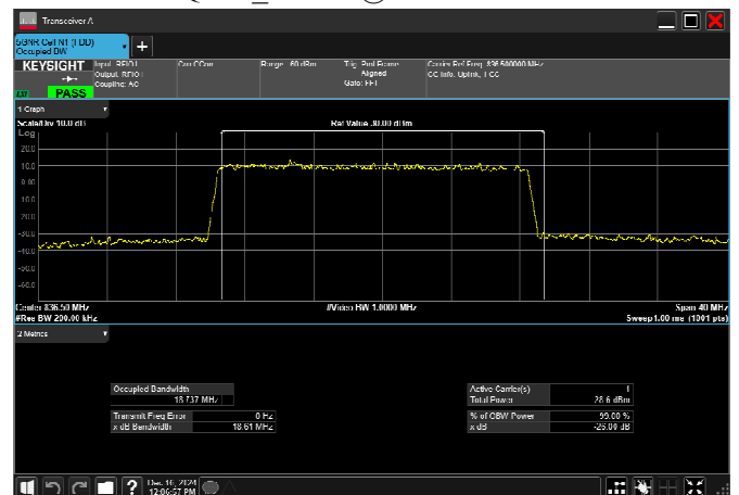
n5_20MHz_15kHz_836.5MHz_DFT-s-OFDM 16 QAM_RB100@0 18.737MHz
