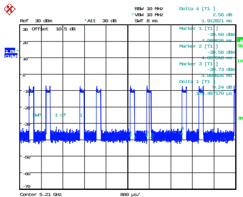
802.11ax80_5210MHz_RU_106/53_Chain 0 0.371ms,1.913ms
