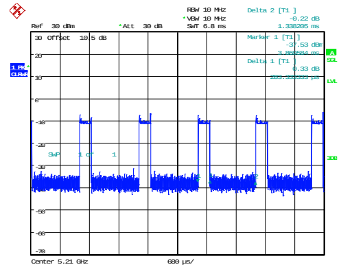
802.11ax80_5210MHz_RU_52/37_Chain 0 0.283ms,1.338ms
