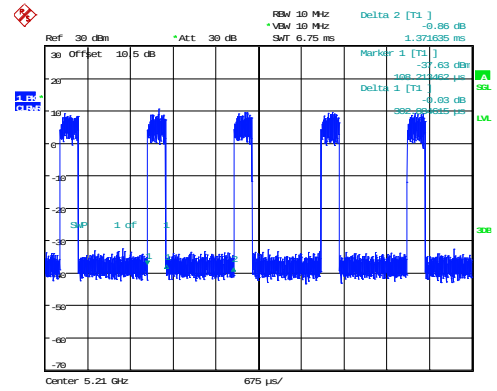
802.11ax80_5210MHz_RU_Full_Chain 0 0.303ms,1.372ms
