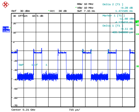
802.11ax80_5210MHz_RU_26/0_Chain 0 0.483ms,1.472ms
