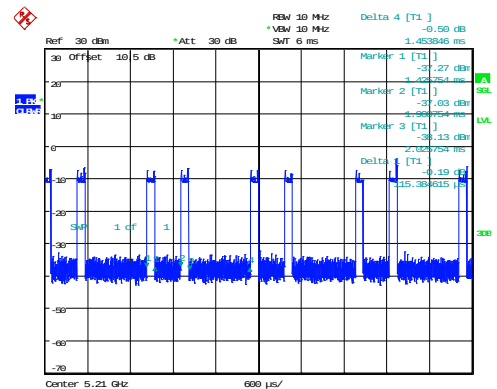
802.11ax80_5210MHz_RU_242/61_Chain 0 0.240ms,1.454ms
