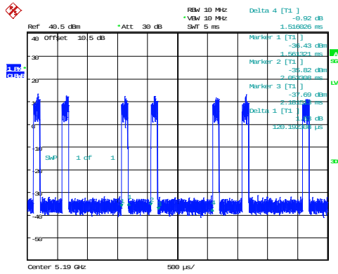
802.11ax40_5190MHz_RU_242/61_Chain 0 0.249ms,1.516ms
