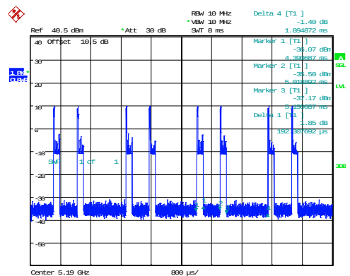
802.11ax40_5190MHz_RU_106/53_Chain 0 0.364ms,1.895ms
