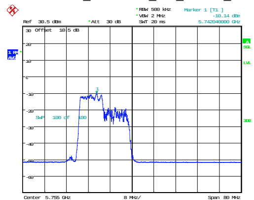
802.11ax40_5755MHz_RU_106/53_Chain 1
