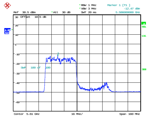
802.11ax80_5610MHz_RU_484/65_Chain 1
