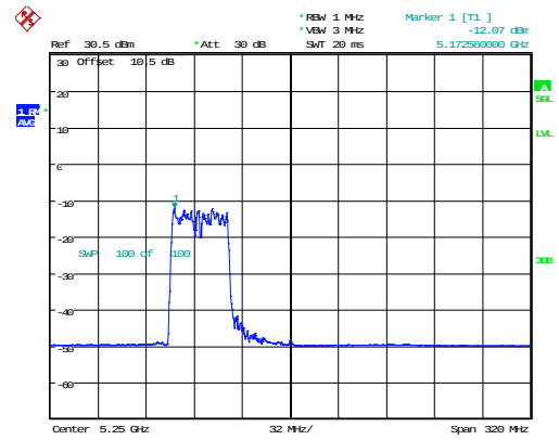
802.11ax160_5250MHz_RU_484/65_Chain 1
