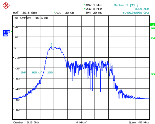
802.11ax20_5500MHz_RU_52/37_Chain 0
