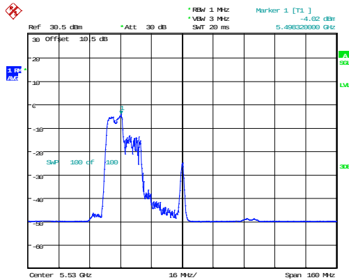
802.11ax80_5530MHz_RU_106/53_Chain 0
