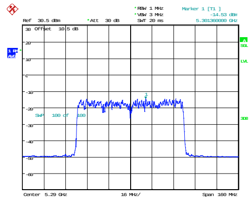
802.11ax80_5290MHz_RU_Full_Chain 1
