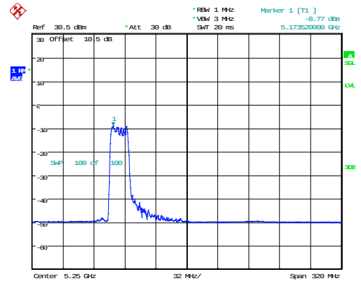
802.11ax160_5250MHz_RU_242/61_Chain 1
