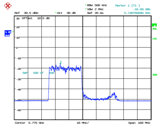
802.11ax80_5775MHz_RU_484/65_Chain 1
