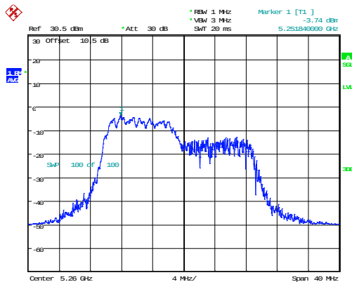
802.11ax20_5260MHz_RU_106/53_Chain 0
