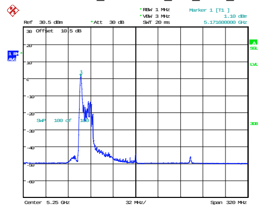
802.11ax160_5250MHz_RU_26/0_Chain 1
