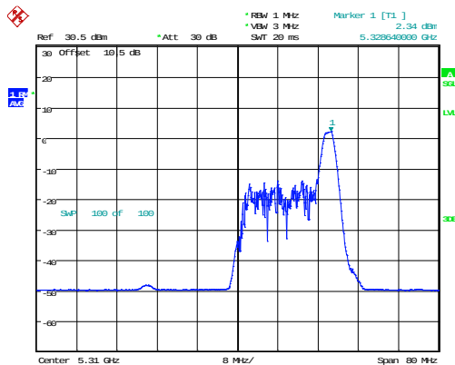
802.11ax40_5310MHz_RU_26/17_Chain 0
