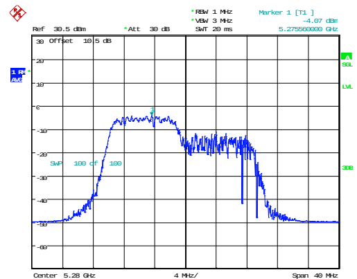
802.11ax20_5280MHz_RU_106/53_Chain 1
