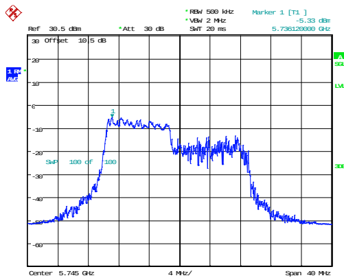
802.11ax20_5745MHz_RU_106/53_Chain 0
