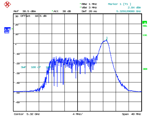
802.11ax20_5320MHz_RU_26/8_Chain 1
