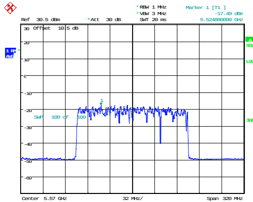
802.11ax160_5570MHz_RU_Full_Chain 0
