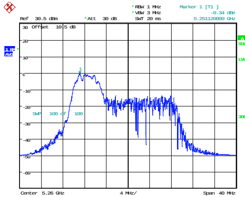
802.11ax20_5260MHz_RU_52/37_Chain 0
