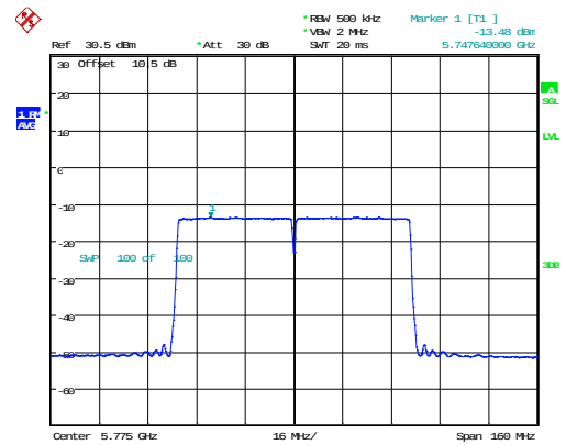
802.11ac80_5775MHz_Chain 1
