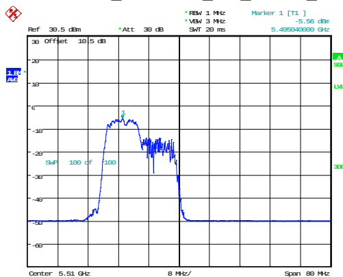
802.11ax40_5510MHz_RU_106/53_Chain 1
