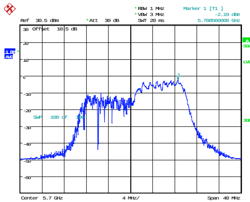
802.11ax20_5700MHz_RU_106/54_Chain 0
