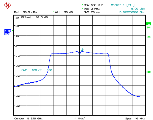
802.11n20_5825MHz_Chain 1
