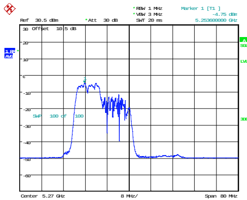
802.11ax40_5270MHz_RU_106/53_Chain 0
