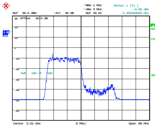
802.11ax40_5510MHz_RU_242/61_Chain 1
