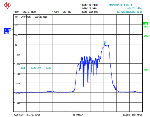
802.11ax40_5710MHz_RU_52/44_Chain 0
