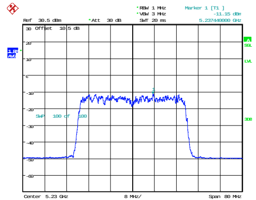
802.11ax40_5230MHz_RU_Full_Chain 0
