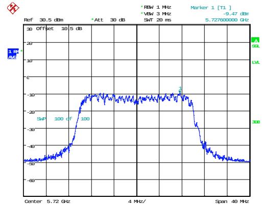
802.11ax20_5720MHz_RU_Full_Chain 1
