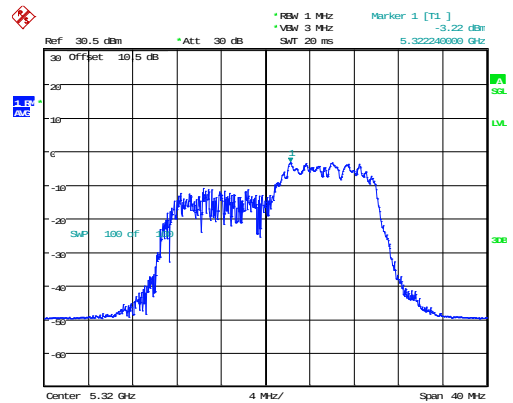
802.11ax20_5320MHz_RU_106/54_Chain 1
