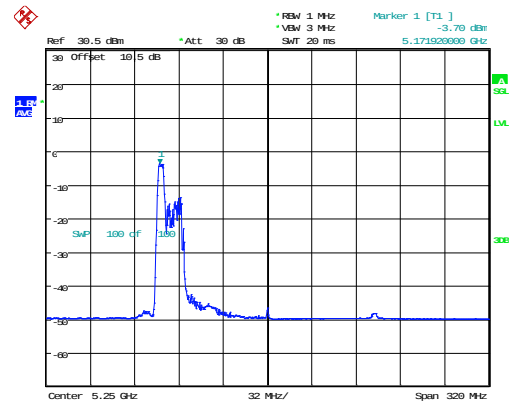
802.11ax160_5250MHz_RU_52/37_Chain 1
