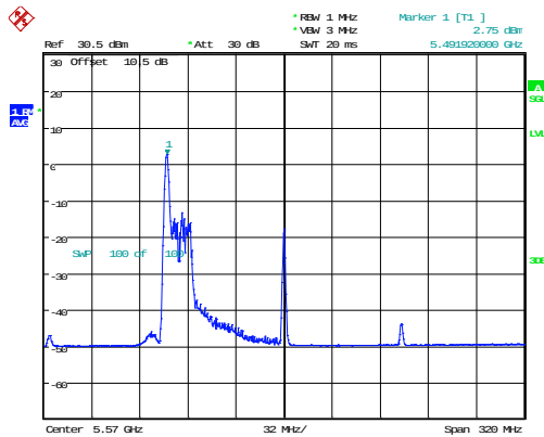
802.11ax160_5570MHz_RU_26/0_Chain 0
