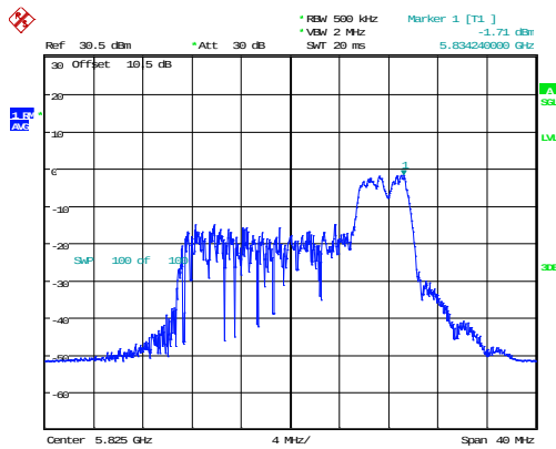
802.11ax20_5825MHz_RU_52/40_Chain 0
