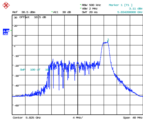
802.11ax20_5825MHz_RU_26/8_Chain 0
