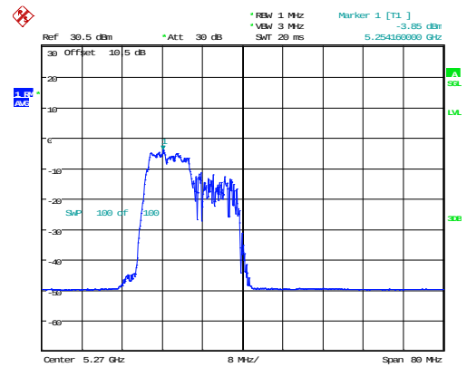
802.11ax40_5270MHz_RU_106/53_Chain 1
