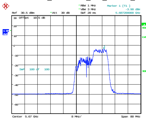
802.11ax40_5670MHz_RU_106/56_Chain 0
