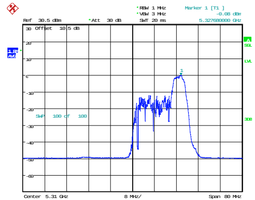
802.11ax40_5310MHz_RU_52/44_Chain 1
