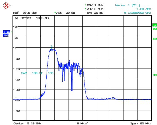
802.11ax40_5190MHz_RU_52/37_Chain 0
