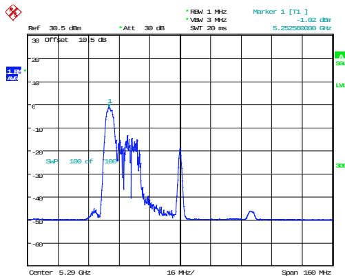
802.11ax80_5290MHz_RU_52/37_Chain 0
