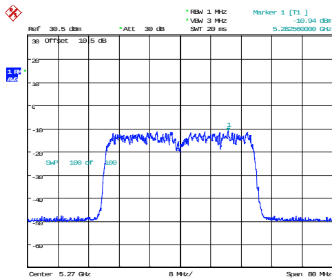
802.11ax40_5270MHz_RU_Full_Chain 1
