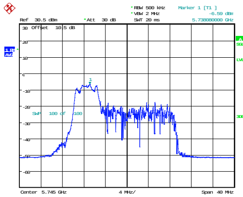
802.11ax20_5745MHz_RU_52/37_Chain 1
