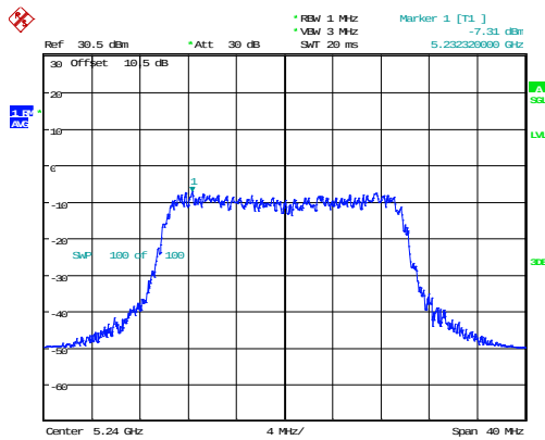
802.11ax20_5240MHz_RU_Full_Chain 0
