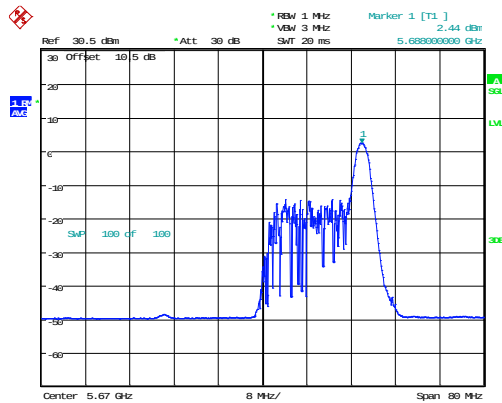
802.11ax40_5670MHz_RU_26/17_Chain 0
