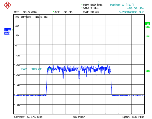
802.11ax80_5775MHz_RU_Full_Chain 1
