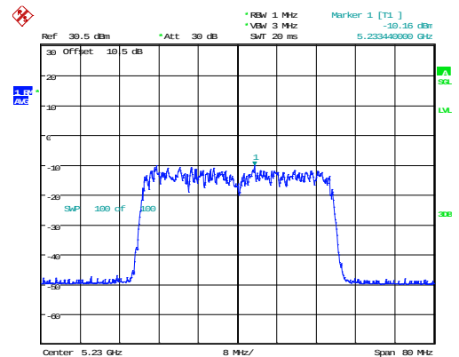
802.11ax40_5230MHz_RU_Full_Chain 1
