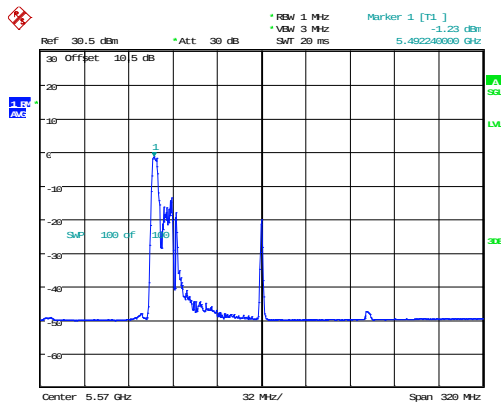
802.11ax160_5570MHz_RU_52/37_Chain 0
