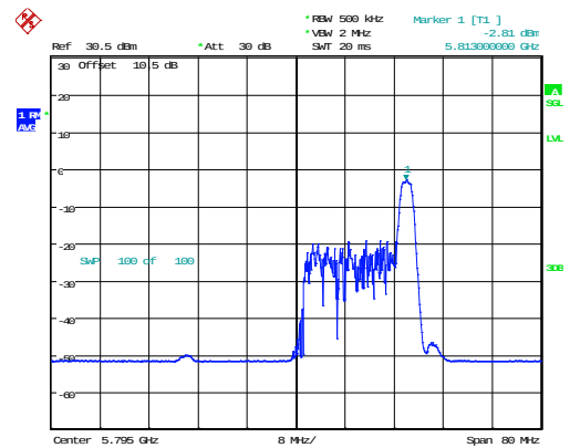
802.11ax40_5795MHz_RU_26/17_Chain 1
