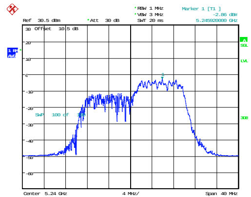
802.11ax20_5240MHz_RU_106/54_Chain 1
