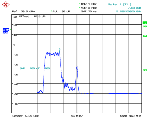
802.11ax80_5210MHz_RU_242/61_Chain 0
