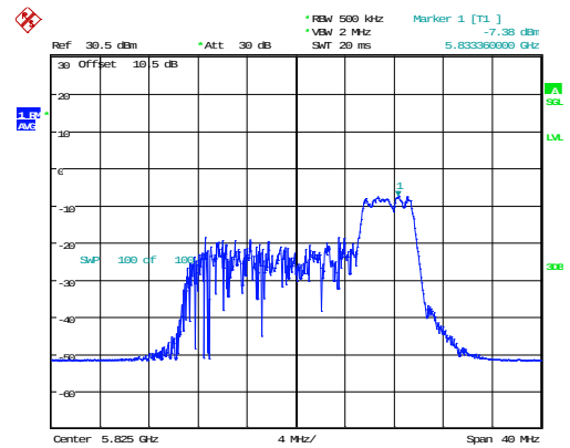
802.11ax20_5825MHz_RU_52/40_Chain 1
