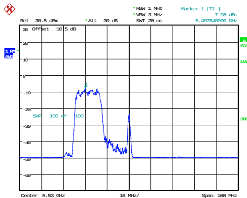
802.11ax80_5530MHz_RU_242/61_Chain 0
