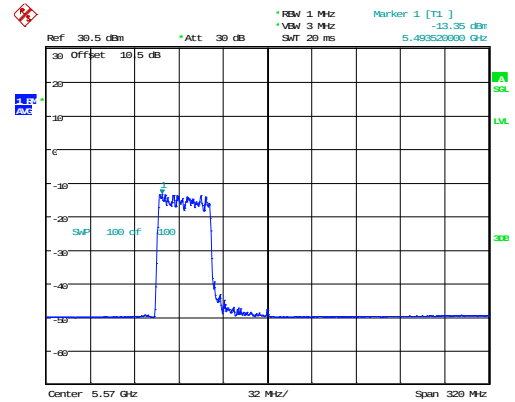
802.11ax160_5570MHz_RU_484/65_Chain 1
