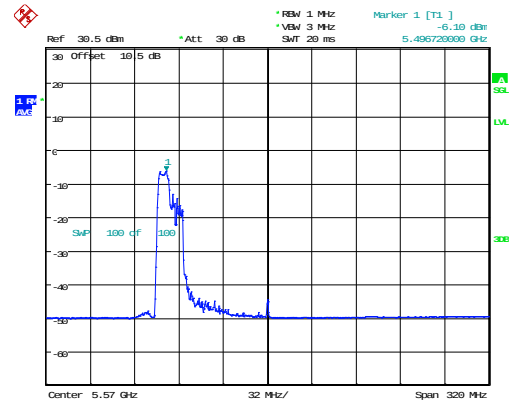
802.11ax160_5570MHz_RU_106/53_Chain 1
