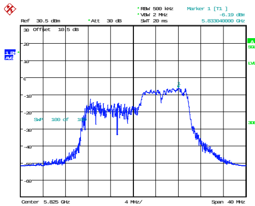
802.11ax20_5825MHz_RU_106/54_Chain 0
