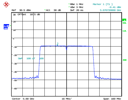
802.11ac80_5690MHz_Chain 1
