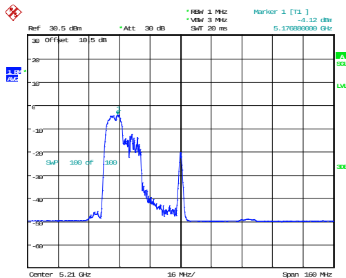
802.11ax80_5210MHz_RU_106/53_Chain 0
