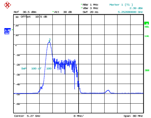
802.11ax40_5270MHz_RU_26/0_Chain 1
