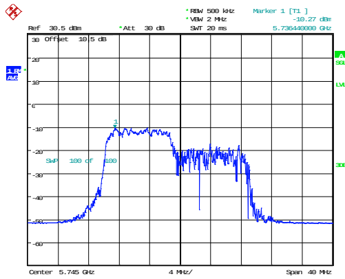
802.11ax20_5745MHz_RU_106/53_Chain 1
