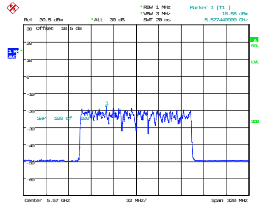
802.11ax160_5570MHz_RU_Full_Chain 1
