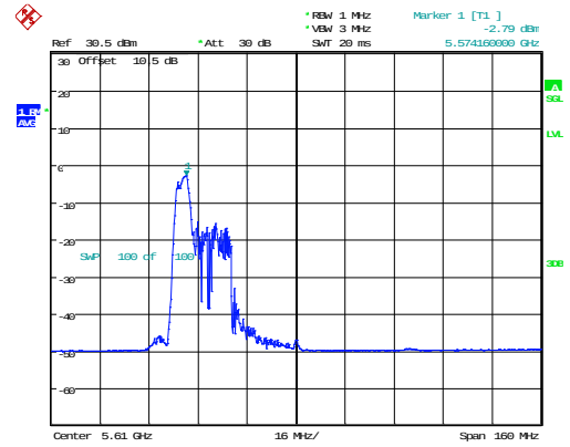
802.11ax80_5610MHz_RU_52/37_Chain 1
