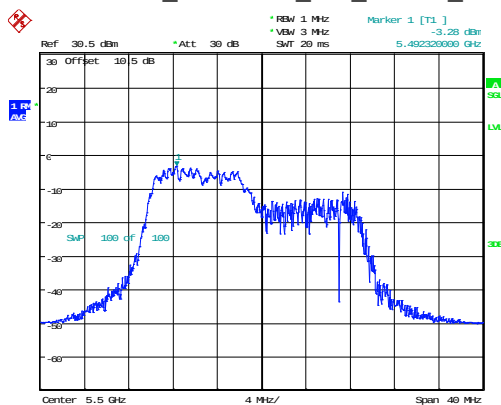
802.11ax20_5500MHz_RU_106/53_Chain 0
