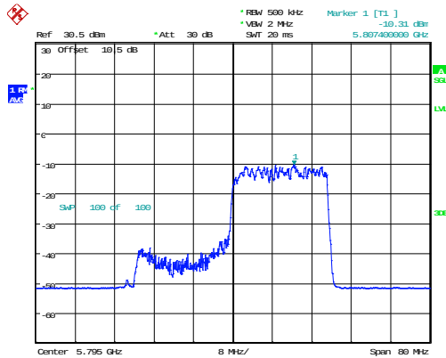
802.11ax40_5795MHz_RU_242/62_Chain 0
