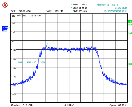
802.11ax20_5200MHz_RU_Full_Chain 1
