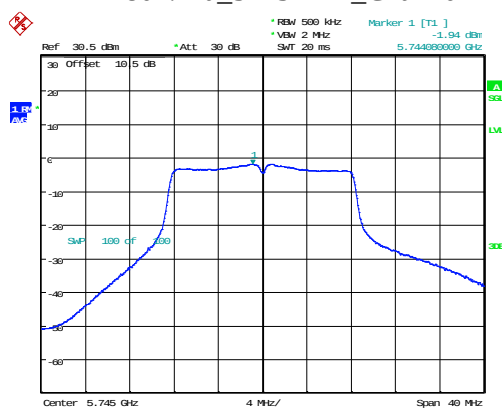
802.11a_5745MHz_Chain 0
