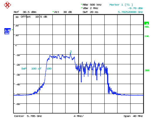
802.11ax20_5785MHz_RU_106/53_Chain 1
