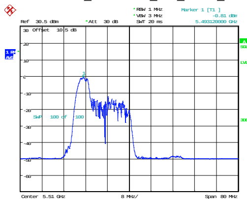
802.11ax40_5510MHz_RU_52/37_Chain 0
