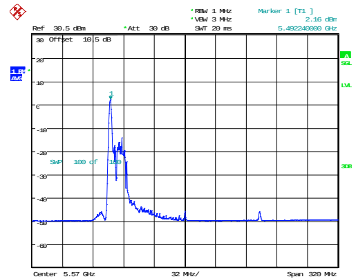
802.11ax160_5570MHz_RU_26/0_Chain 1
