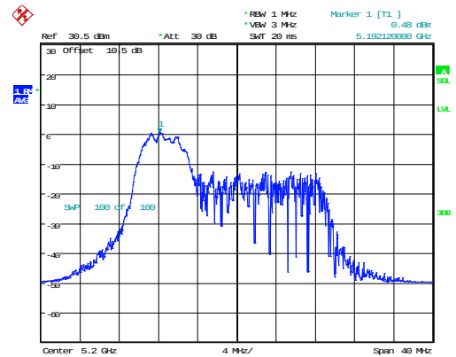
802.11ax20_5200MHz_RU_52/37_Chain 0
