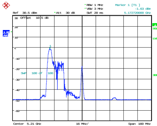
802.11ax80_5210MHz_RU_52/37_Chain 0
