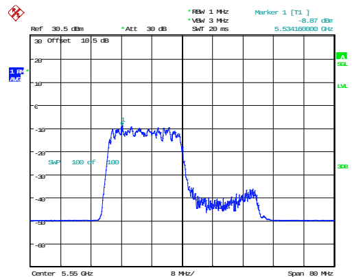
802.11ax40_5550MHz_RU_242/61_Chain 1
