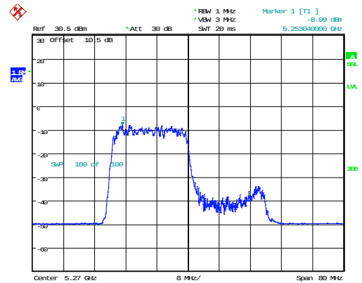
802.11ax40_5270MHz_RU_242/61_Chain 1
