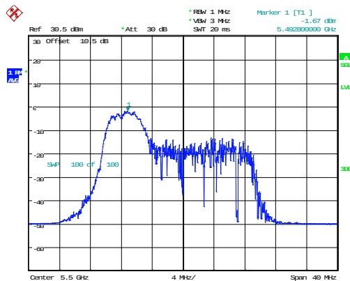
802.11ax20_5500MHz_RU_52/37_Chain 1
