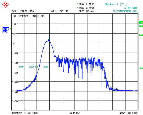
802.11ax20_5260MHz_RU_26/0_Chain 1
