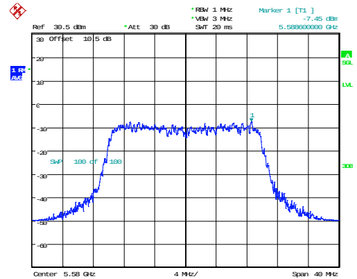
802.11ax20_5580MHz_RU_Full_Chain 0
