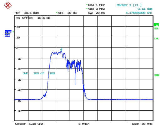
802.11ax40_5190MHz_RU_106/53_Chain 1
