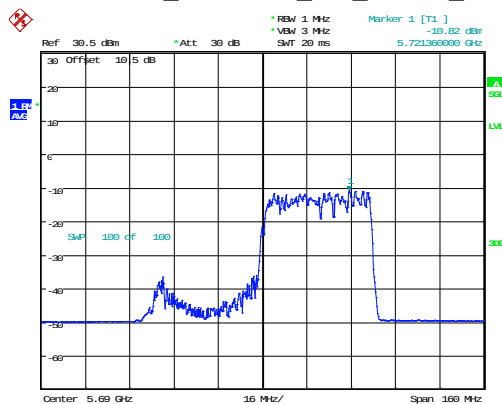
802.11ax80_5690MHz_RU_484/66_Chain 0
