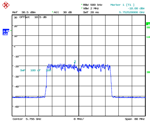
802.11ax40_5755MHz_RU_Full_Chain 1
