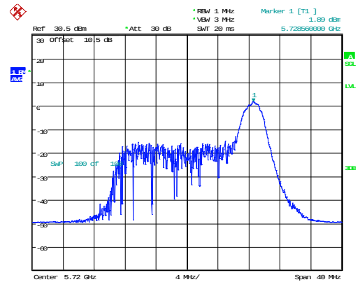
802.11ax20_5720MHz_RU_26/8_Chain 1
