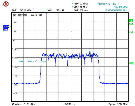
802.11ax80_5610MHz_RU_Full_Chain 0
