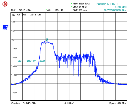
802.11ax20_5745MHz_RU_52/37_Chain 0
