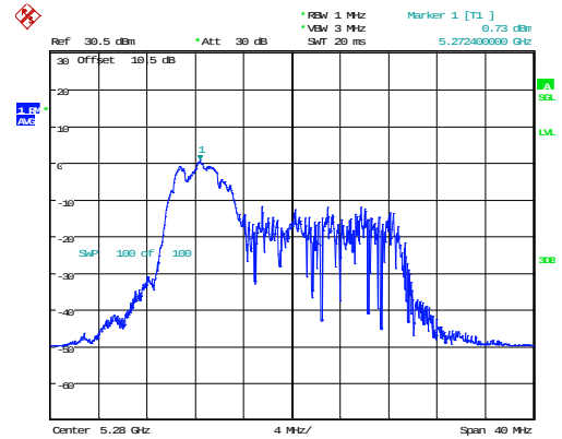
802.11ax20_5280MHz_RU_52/37_Chain 0
