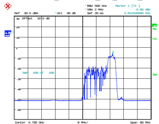
802.11ax40_5795MHz_RU_52/44_Chain 1
