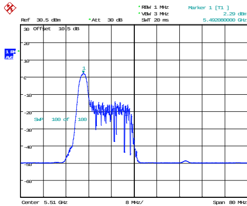
802.11ax40_5510MHz_RU_26/0_Chain 1
