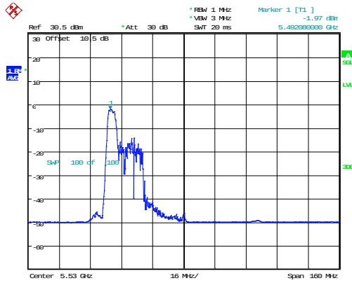
802.11ax80_5530MHz_RU_52/37_Chain 1
