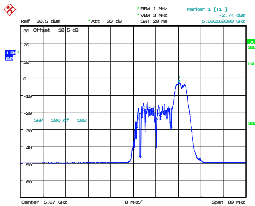
802.11ax40_5670MHz_RU_52/44_Chain 1
