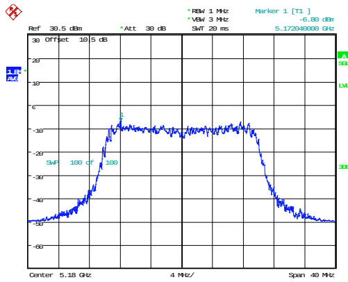
802.11ax20_5180MHz_RU_Full_Chain 0
