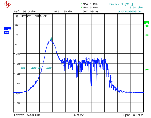
802.11ax20_5580MHz_RU_26/0_Chain 0
