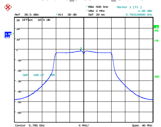
802.11a_5785MHz_Chain 0
