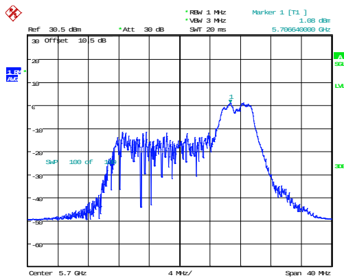
802.11ax20_5700MHz_RU_52/40_Chain 0
