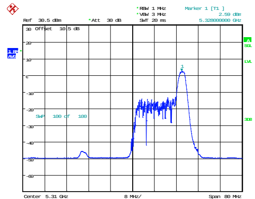
802.11ax40_5310MHz_RU_26/17_Chain 1
