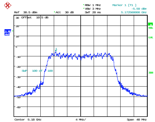
802.11ax20_5180MHz_RU_Full_Chain 1
