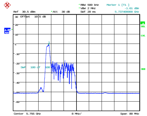
802.11ax40_5755MHz_RU_26/0_Chain 1
