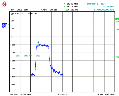
802.11ax80_5530MHz_RU_242/61_Chain 1
