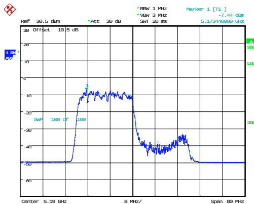
802.11ax40_5190MHz_RU_242/61_Chain 0
