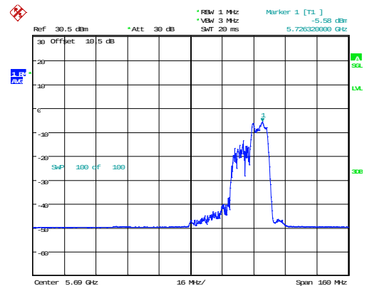
802.11ax80_5690MHz_RU_106/60_Chain 1
