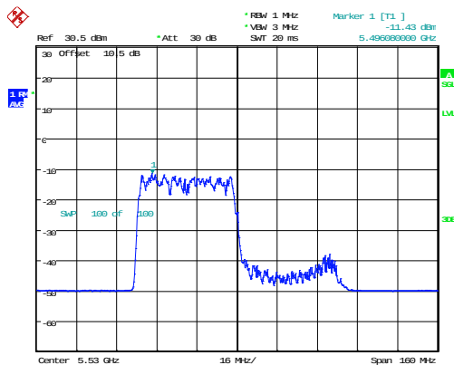
802.11ax80_5530MHz_RU_484/65_Chain 0
