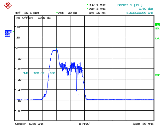
802.11ax40_5550MHz_RU_52/37_Chain 1
