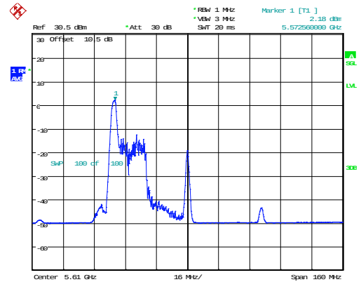
802.11ax80_5610MHz_RU_26/0_Chain 0
