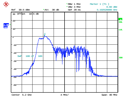
802.11ax20_5200MHz_RU_52/37_Chain 1
