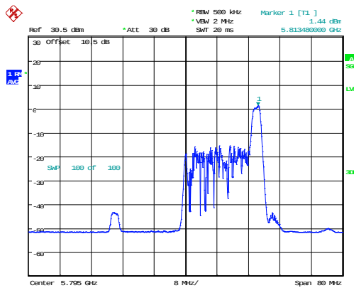
802.11ax40_5795MHz_RU_26/17_Chain 0
