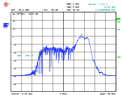
802.11ax20_5240MHz_RU_52/40_Chain 1
