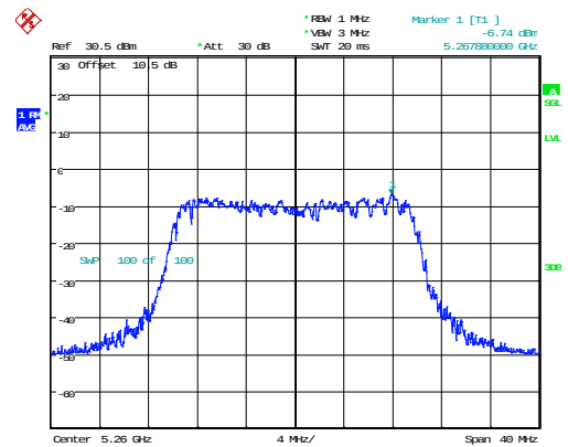
802.11ax20_5260MHz_RU_Full_Chain 1
