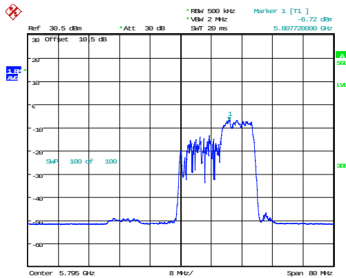
802.11ax40_5795MHz_RU_106/56_Chain 0
