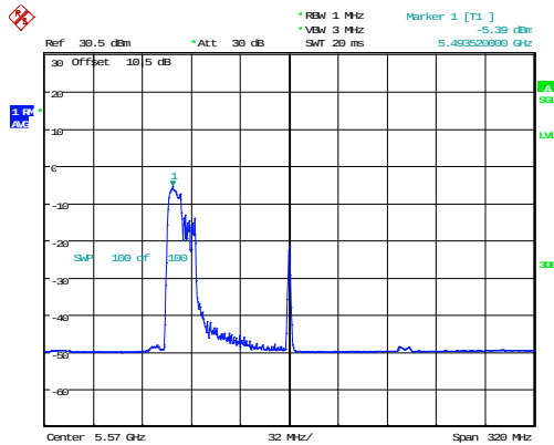
802.11ax160_5570MHz_RU_106/53_Chain 0
