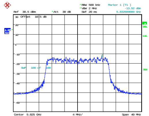
802.11ax20_5825MHz_RU_Full_Chain 1
