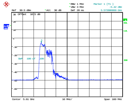
802.11ax80_5610MHz_RU_106/53_Chain 1
