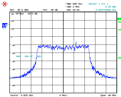
802.11ax20_5825MHz_RU_Full_Chain 0
