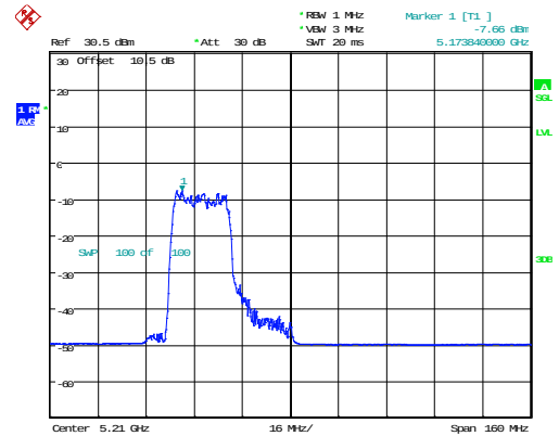
802.11ax80_5210MHz_RU_242/61_Chain 1
