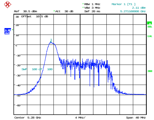
802.11ax20_5280MHz_RU_26/0_Chain 0
