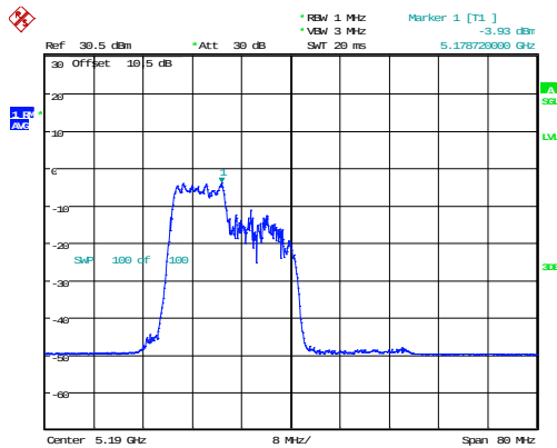
802.11ax40_5190MHz_RU_106/53_Chain 0
