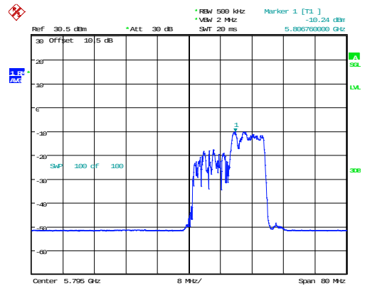
802.11ax40_5795MHz_RU_106/56_Chain 1
