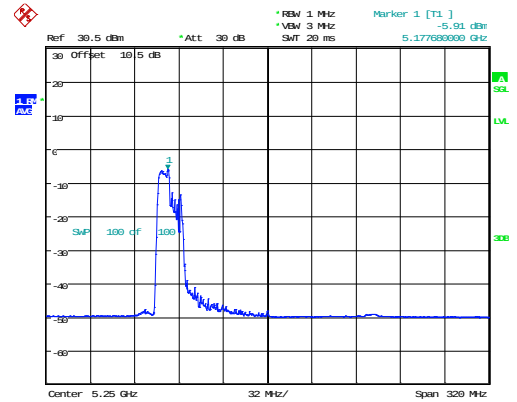
802.11ax160_5250MHz_RU_106/53_Chain 1
