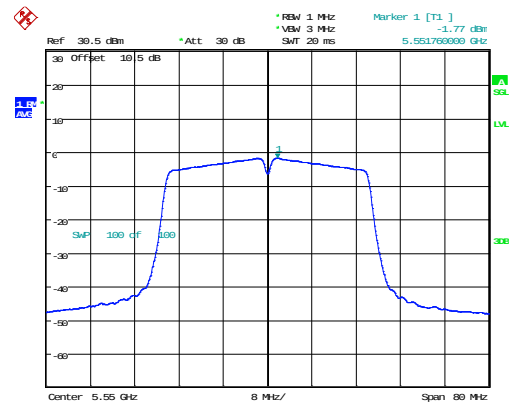
802.11n40_5550MHz_Chain 0
