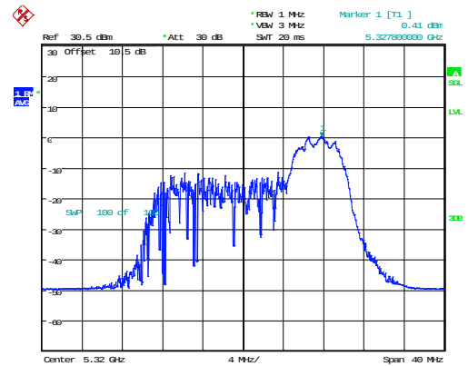
802.11ax20_5320MHz_RU_52/40_Chain 1
