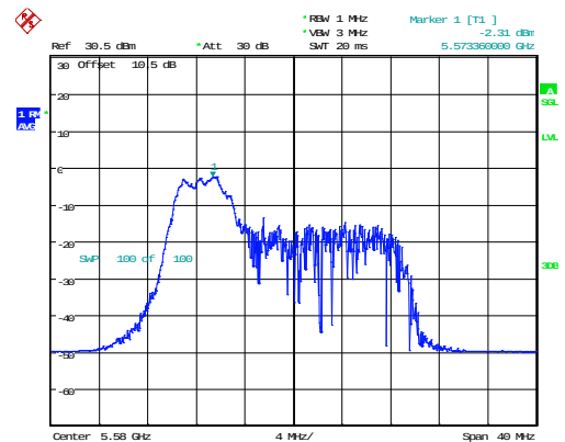
802.11ax20_5580MHz_RU_52/37_Chain 1
