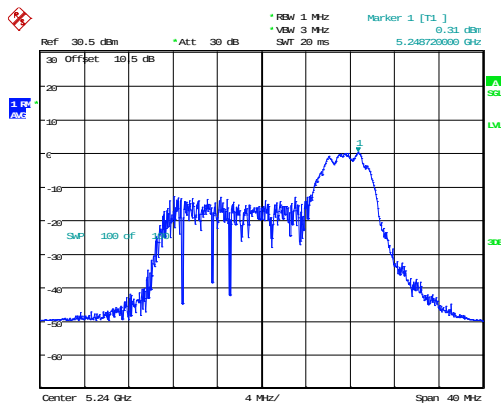
802.11ax20_5240MHz_RU_52/40_Chain 0
