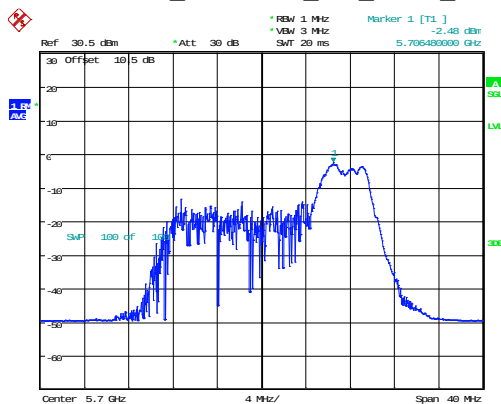
802.11ax20_5700MHz_RU_52/40_Chain 1
