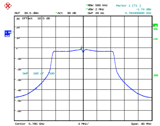
802.11n20_5785MHz_Chain 0
