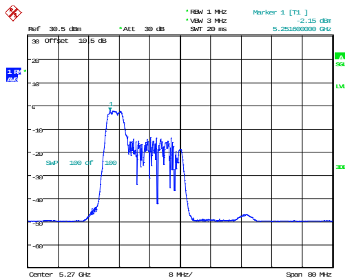
802.11ax40_5270MHz_RU_52/37_Chain 0
