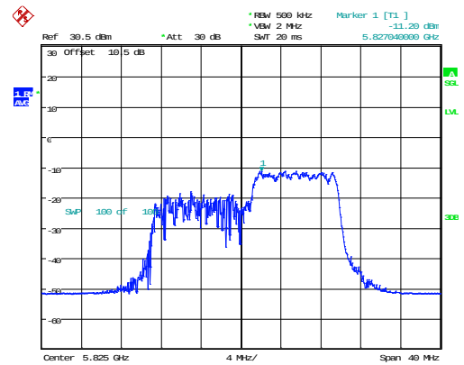
802.11ax20_5825MHz_RU_106/54_Chain 1
