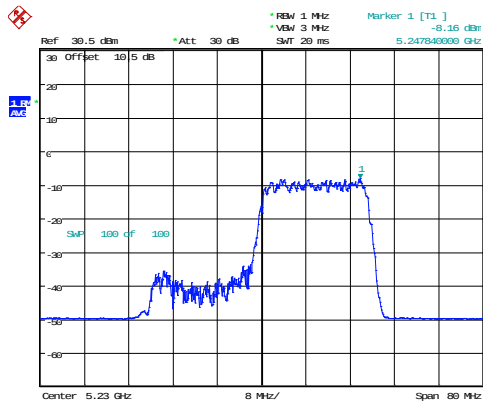
802.11ax40_5230MHz_RU_242/62_Chain 0
