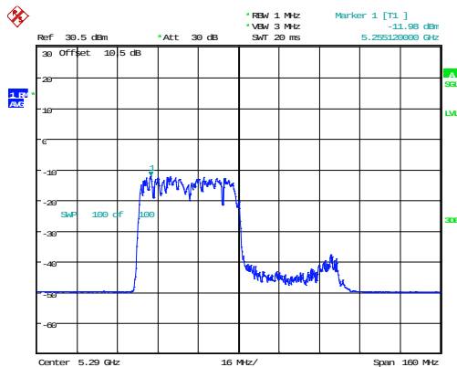
802.11ax80_5290MHz_RU_484/65_Chain 0
