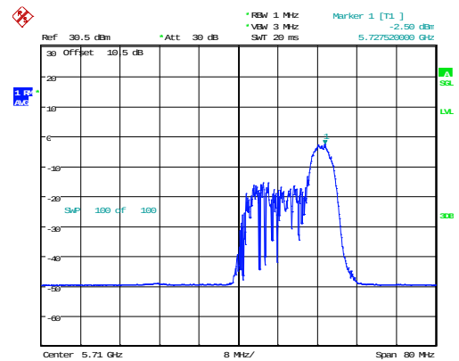
802.11ax40_5710MHz_RU_52/44_Chain 1
