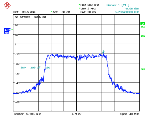
802.11ax20_5785MHz_RU_Full_Chain 0
