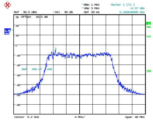
802.11ax20_5200MHz_RU_Full_Chain 0
