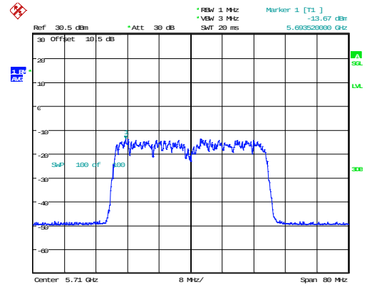
802.11ax40_5710MHz_RU_Full_Chain 1
