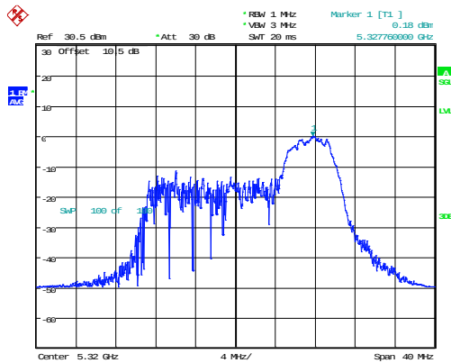
802.11ax20_5320MHz_RU_52/40_Chain 0
