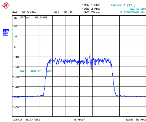
802.11ax40_5270MHz_RU_Full_Chain 0
