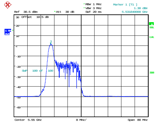
802.11ax40_5550MHz_RU_26/0_Chain 1
