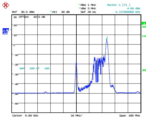
802.11ax80_5690MHz_RU_26/36_Chain 0
