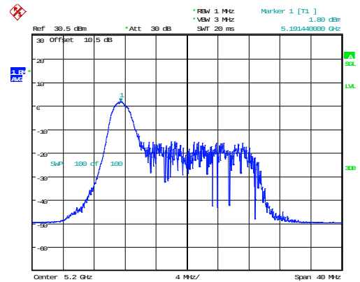
802.11ax20_5200MHz_RU_26/0_Chain 0
