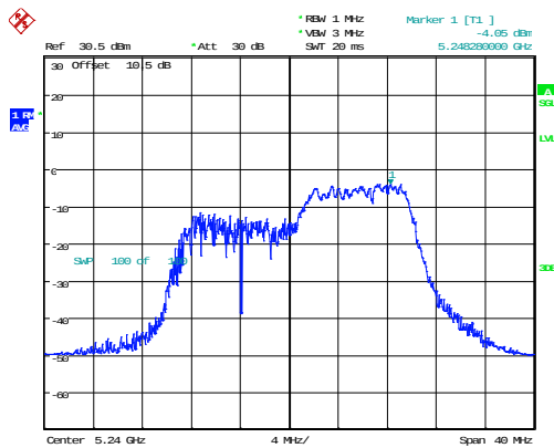
802.11ax20_5240MHz_RU_106/54_Chain 0
