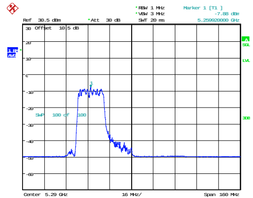
802.11ax80_5290MHz_RU_242/61_Chain 1
