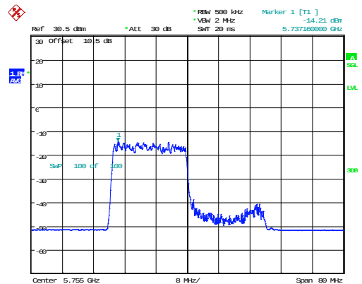
802.11ax40_5755MHz_RU_242/61_Chain 1
