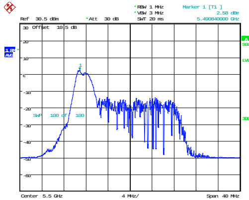
802.11ax20_5500MHz_RU_26/0_Chain 1
