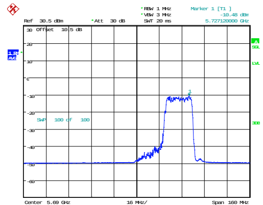
802.11ax80_5690MHz_RU_242/64_Chain 1
