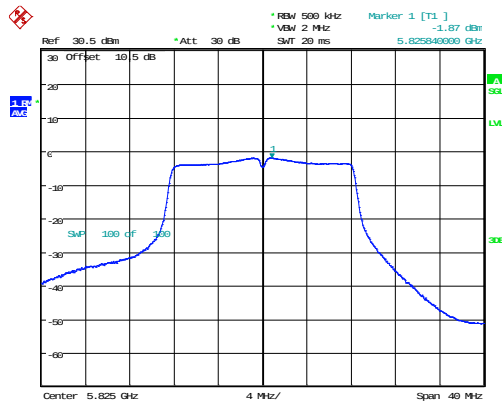
802.11a_5825MHz_Chain 0
