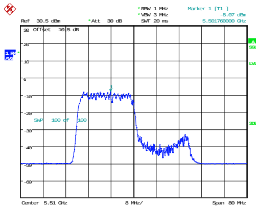
802.11ax40_5510MHz_RU_242/61_Chain 0
