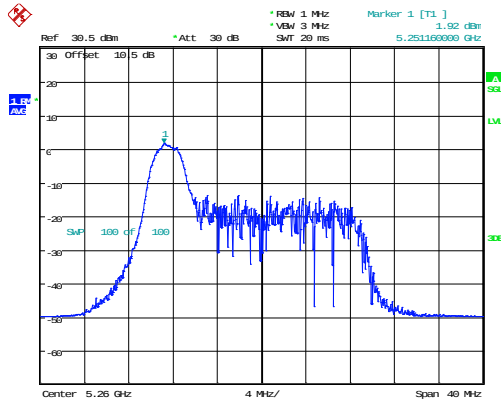
802.11ax20_5260MHz_RU_26/0_Chain 0
