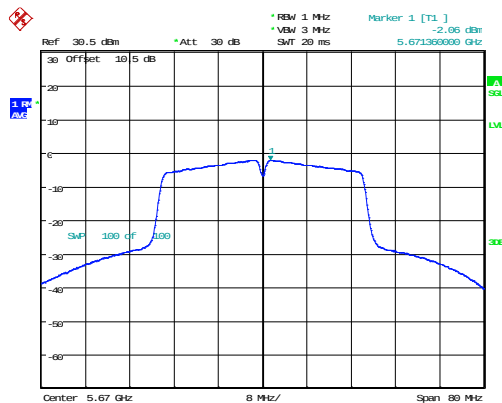
802.11n40_5670MHz_Chain 0
