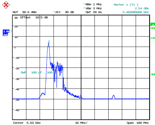
802.11ax80_5530MHz_RU_26/0_Chain 0
