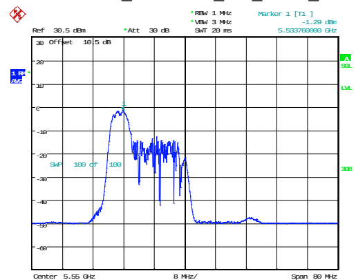
802.11ax40_5550MHz_RU_52/37_Chain 0
