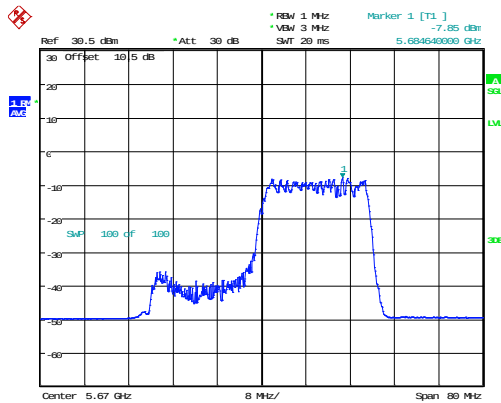
802.11ax40_5670MHz_RU_242/62_Chain 0
