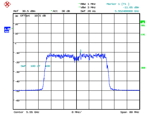
802.11ax40_5550MHz_RU_Full_Chain 0
