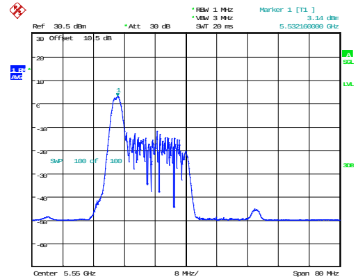
802.11ax40_5550MHz_RU_26/0_Chain 0
