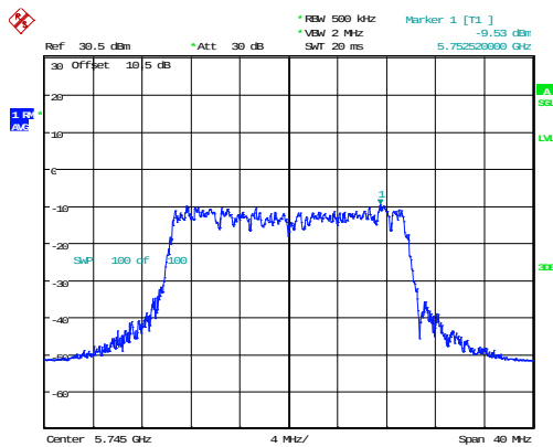
802.11ax20_5745MHz_RU_Full_Chain 0
