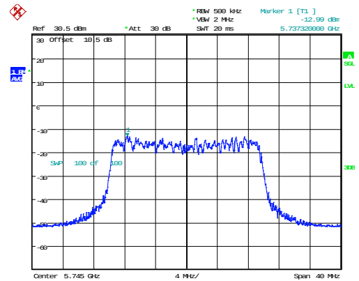
802.11ax20_5745MHz_RU_Full_Chain 1
