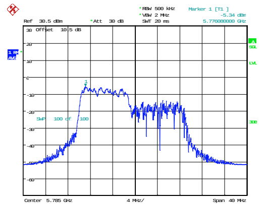
802.11ax20_5785MHz_RU_106/53_Chain 0
