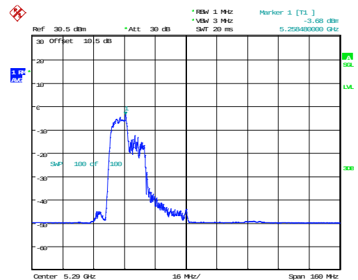
802.11ax80_5290MHz_RU_106/53_Chain 1
