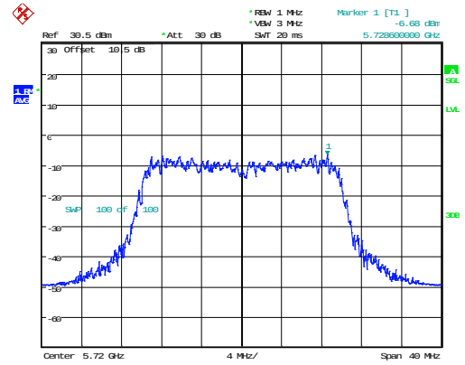
802.11ax20_5720MHz_RU_Full_Chain 0
