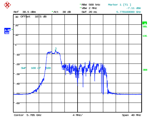
802.11ax20_5785MHz_RU_52/37_Chain 1
