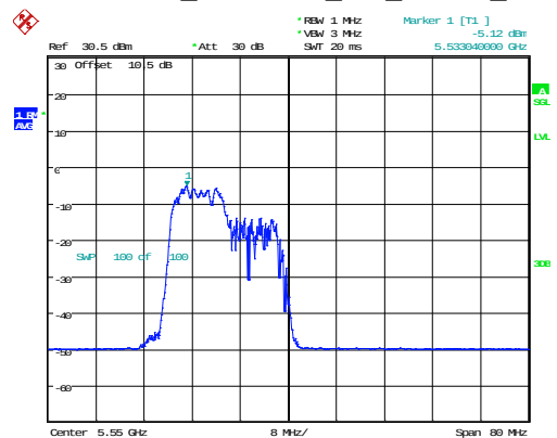
802.11ax40_5550MHz_RU_106/53_Chain 1
