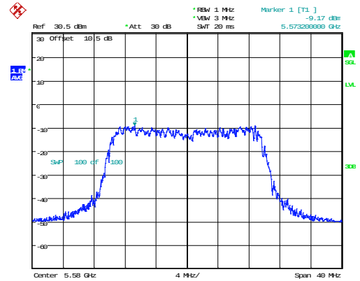
802.11ax20_5580MHz_RU_Full_Chain 1
