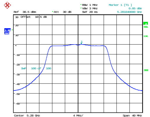
802.11n20_5280MHz_Chain 0
