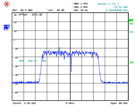
802.11ax40_5550MHz_RU_Full_Chain 1
