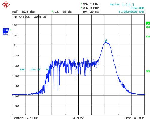
802.11ax20_5700MHz_RU_26/8_Chain 0
