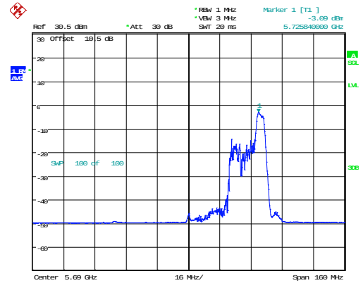
802.11ax80_5690MHz_RU_52/52_Chain 1
