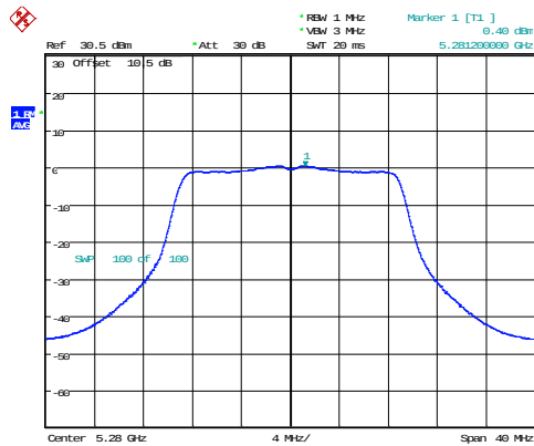
802.11n20_5280MHz_Chain 1
