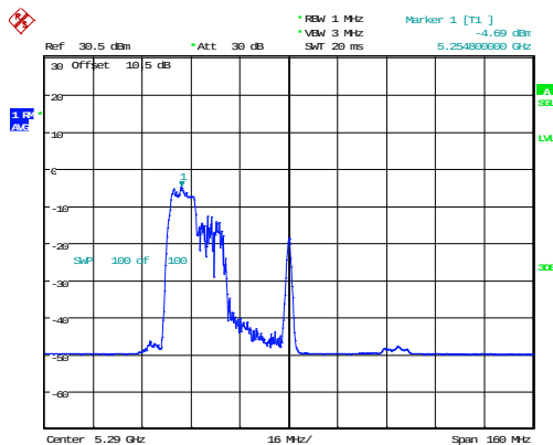
802.11ax80_5290MHz_RU_106/53_Chain 0
