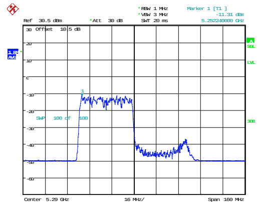
802.11ax80_5290MHz_RU_484/65_Chain 1
