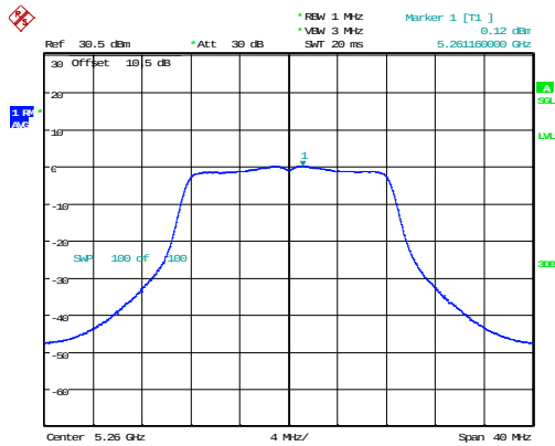
802.11a_5260MHz_Chain 0
