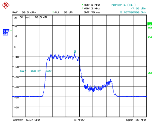
802.11ax40_5270MHz_RU_242/61_Chain 0
