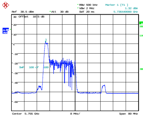
802.11ax40_5755MHz_RU_26/0_Chain 0
