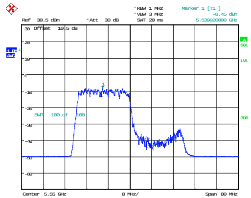
802.11ax40_5550MHz_RU_242/61_Chain 0
