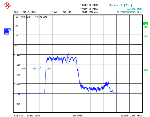
802.11ax80_5610MHz_RU_484/65_Chain 0
