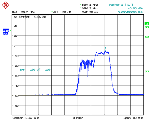
802.11ax40_5670MHz_RU_106/56_Chain 1
