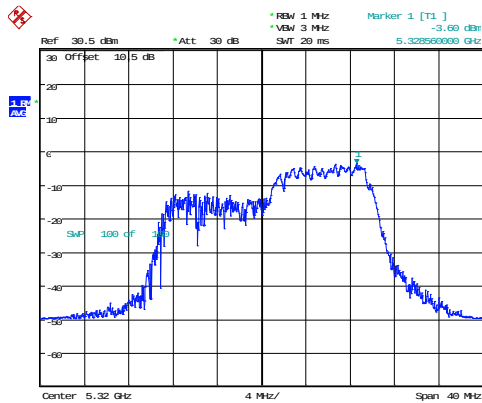
802.11ax20_5320MHz_RU_106/54_Chain 0
