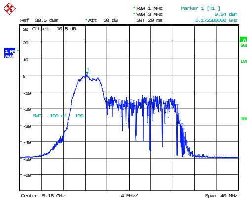
802.11ax20_5180MHz_RU_52/37_Chain 1
