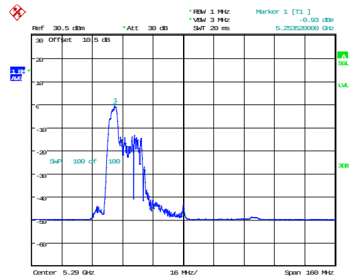
802.11ax80_5290MHz_RU_52/37_Chain 1
