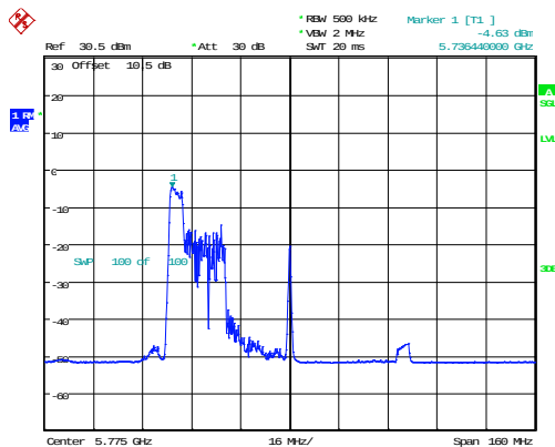
802.11ax80_5775MHz_RU_52/37_Chain 0
