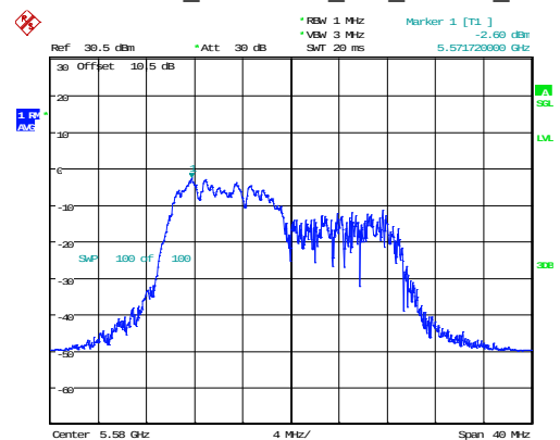
802.11ax20_5580MHz_RU_106/53_Chain 0
