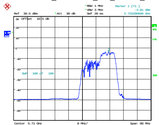
802.11ax40_5710MHz_RU_106/56_Chain 0
