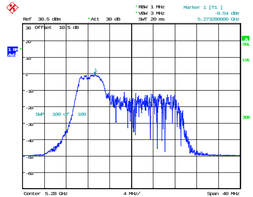
802.11ax20_5280MHz_RU_52/37_Chain 1
