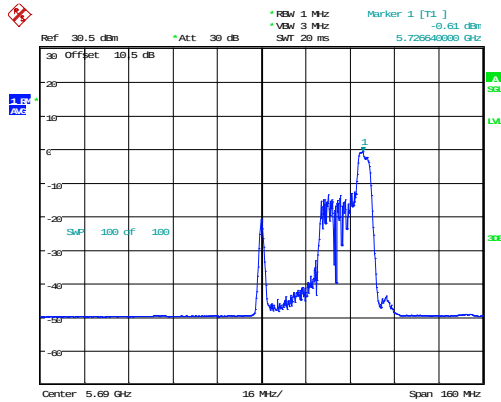
802.11ax80_5690MHz_RU_52/52_Chain 0
