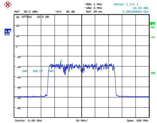
802.11ax80_5690MHz_RU_Full_Chain 1
