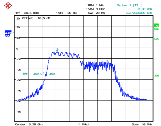
802.11ax20_5280MHz_RU_106/53_Chain 0
