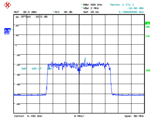
802.11ax40_5795MHz_RU_Full_Chain 1
