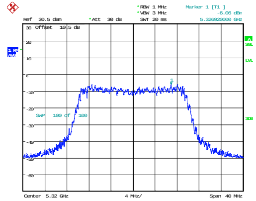
802.11ax20_5320MHz_RU_Full_Chain 1
