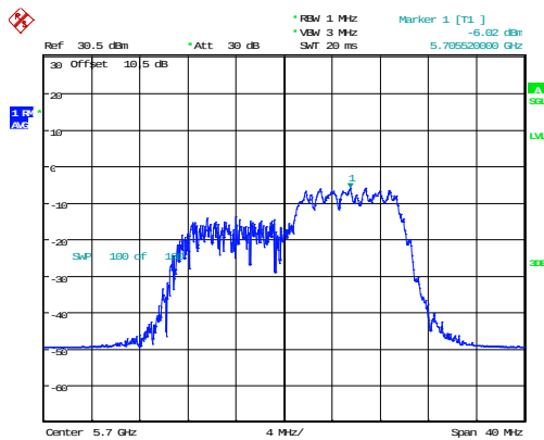
802.11ax20_5700MHz_RU_106/54_Chain 1
