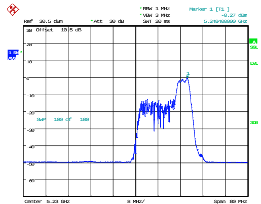
802.11ax40_5230MHz_RU_52/44_Chain 1
