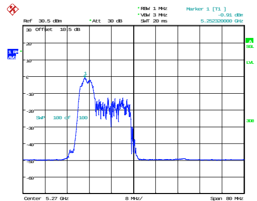
802.11ax40_5270MHz_RU_52/37_Chain 1
