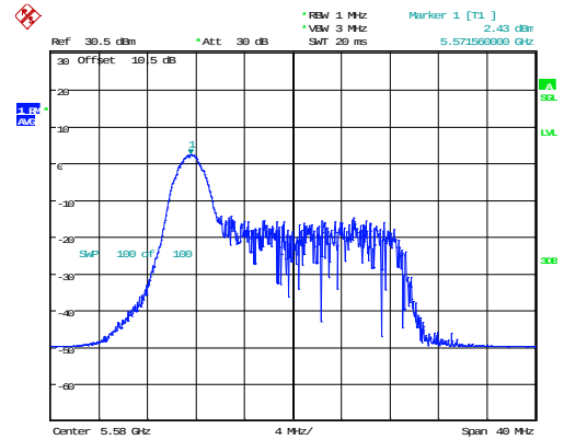
802.11ax20_5580MHz_RU_26/0_Chain 1
