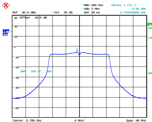
802.11n20_5785MHz_Chain 1
