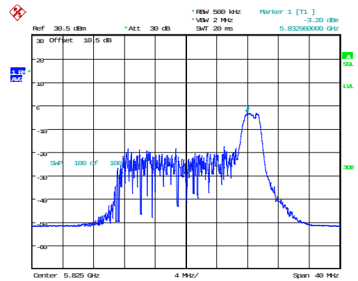
802.11ax20_5825MHz_RU_26/8_Chain 1
