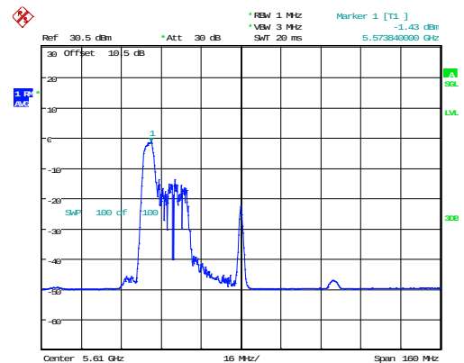
802.11ax80_5610MHz_RU_52/37_Chain 0
