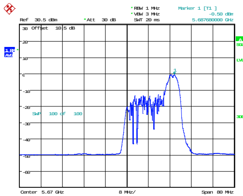
802.11ax40_5670MHz_RU_52/44_Chain 0
