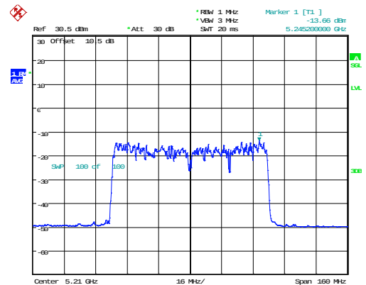
802.11ax80_5210MHz_RU_Full_Chain 1
