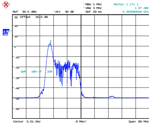
802.11ax40_5510MHz_RU_26/0_Chain 0
