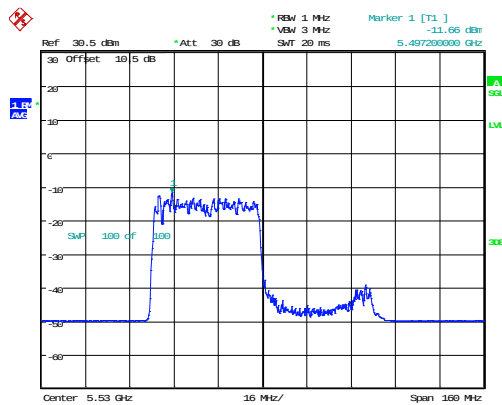
802.11ax80_5530MHz_RU_484/65_Chain 1
