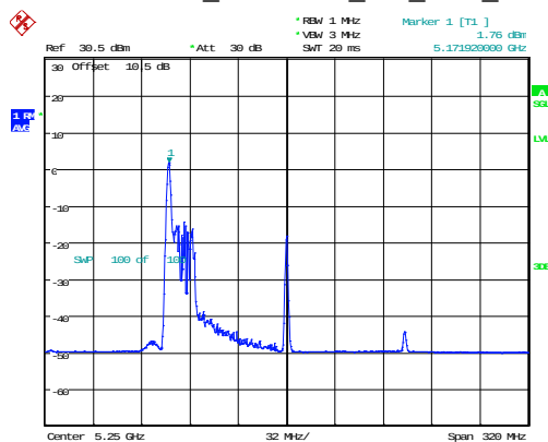
802.11ax160_5250MHz_RU_26/0_Chain 0
