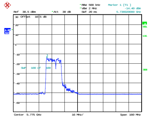
802.11ax80_5775MHz_RU_242/61_Chain 1
