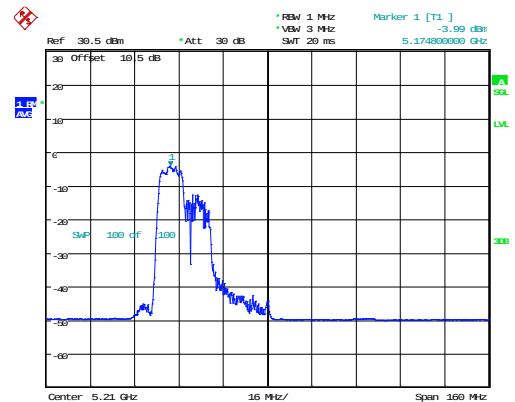
802.11ax80_5210MHz_RU_106/53_Chain 1
