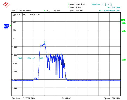
802.11ax40_5755MHz_RU_52/37_Chain 1
