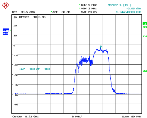
802.11ax40_5230MHz_RU_106/56_Chain 0
