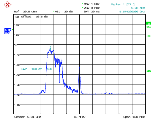
802.11ax80_5610MHz_RU_106/53_Chain 0
