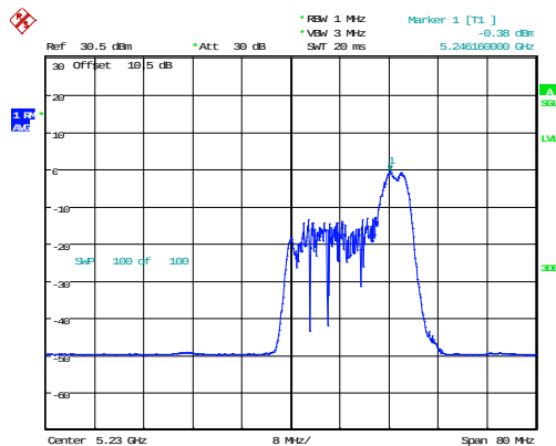
802.11ax40_5230MHz_RU_52/44_Chain 0
