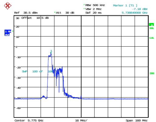
802.11ax80_5775MHz_RU_52/37_Chain 1
