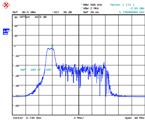
802.11ax20_5745MHz_RU_26/0_Chain 1
