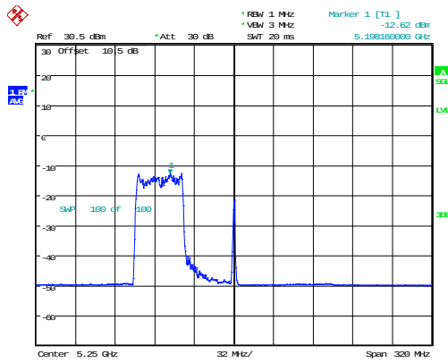
802.11ax160_5250MHz_RU_484/65_Chain 0
