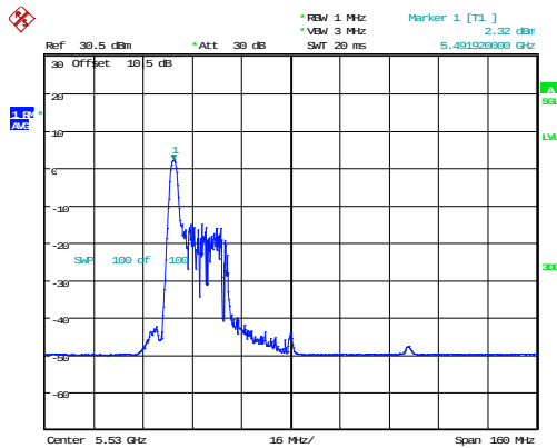
802.11ax80_5530MHz_RU_26/0_Chain 1
