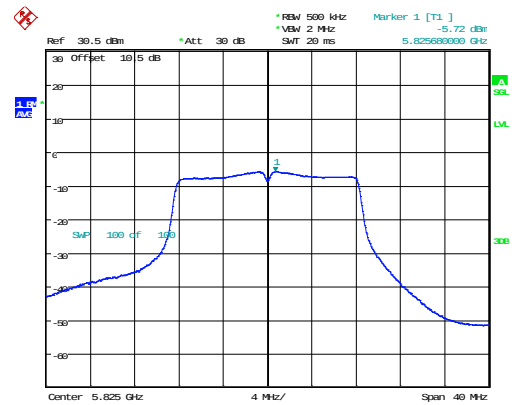
802.11a_5825MHz_Chain 1
