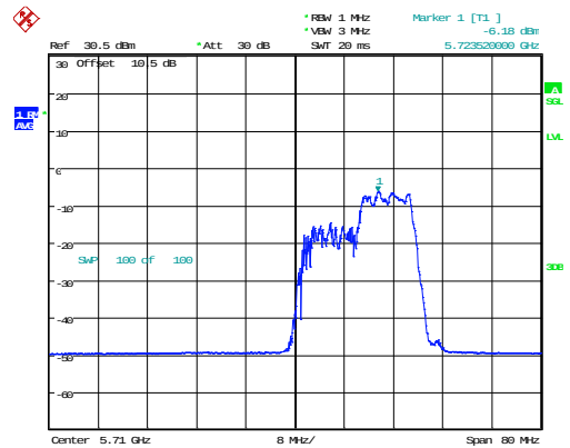
802.11ax40_5710MHz_RU_106/56_Chain 1
