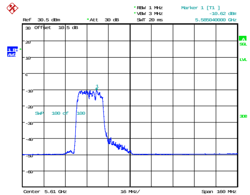
802.11ax80_5610MHz_RU_242/61_Chain 1
