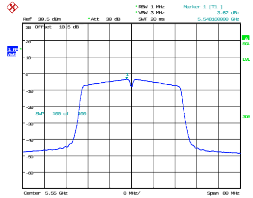
802.11n40_5550MHz_Chain 1
