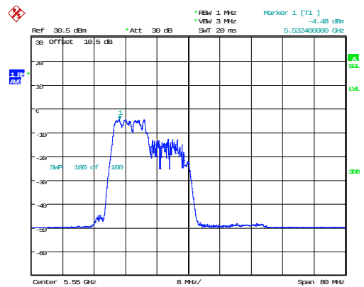
802.11ax40_5550MHz_RU_106/53_Chain 0
