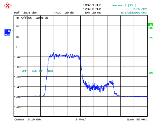
802.11ax40_5190MHz_RU_242/61_Chain 1
