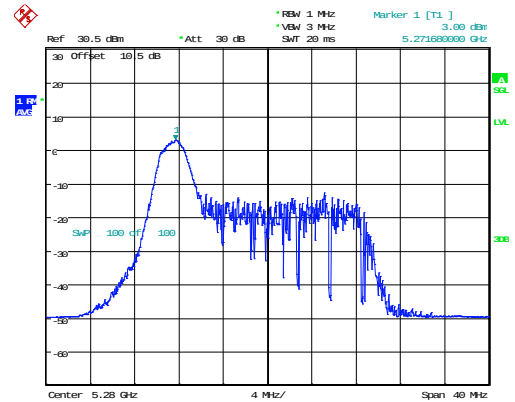
802.11ax20_5280MHz_RU_26/0_Chain 1
