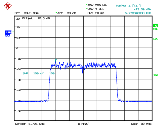
802.11ax40_5795MHz_RU_Full_Chain 0
