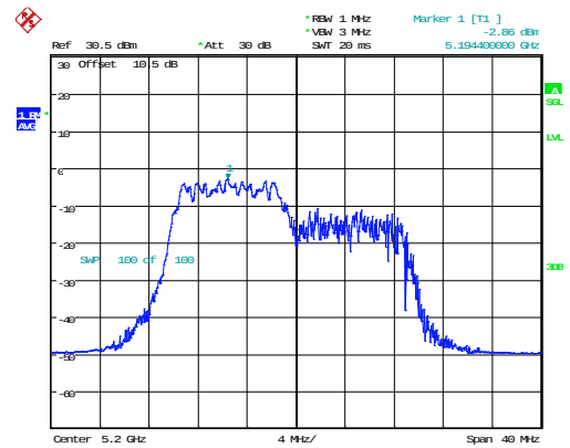
802.11ax20_5200MHz_RU_106/53_Chain 1
