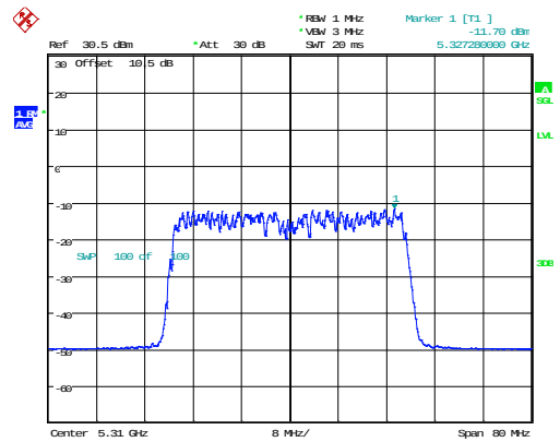
802.11ax40_5310MHz_RU_Full_Chain 0
