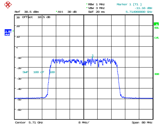
802.11ax40_5710MHz_RU_Full_Chain 0
