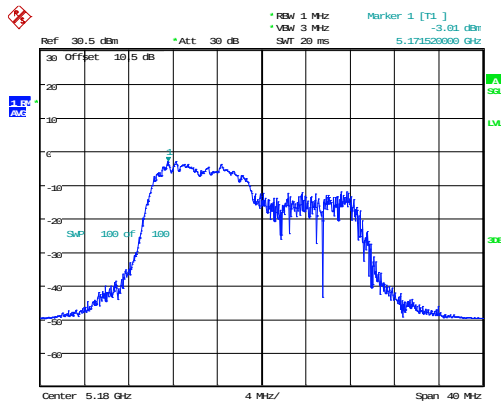
802.11ax20_5180MHz_RU_106/53_Chain 0
