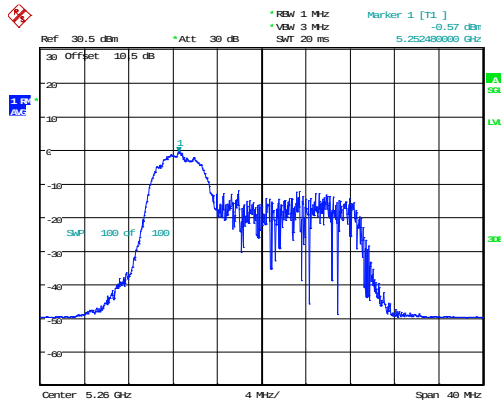
802.11ax20_5260MHz_RU_52/37_Chain 1
