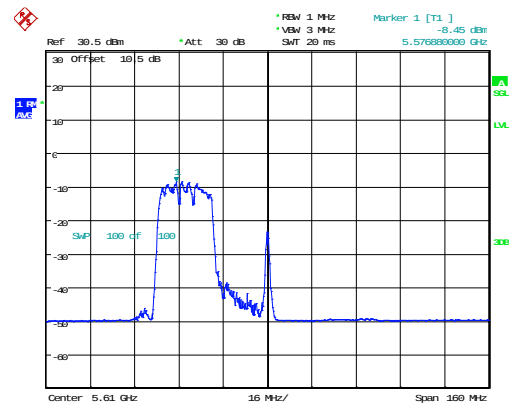
802.11ax80_5610MHz_RU_242/61_Chain 0
