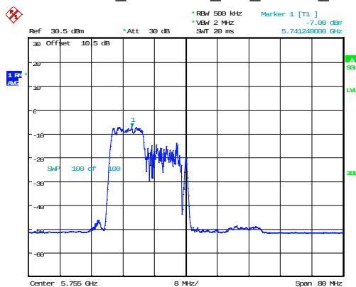
802.11ax40_5755MHz_RU_106/53_Chain 0
