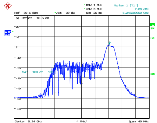
802.11ax20_5240MHz_RU_26/8_Chain 1
