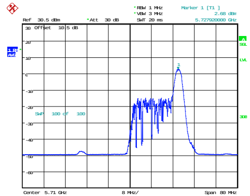
802.11ax40_5710MHz_RU_26/17_Chain 0
