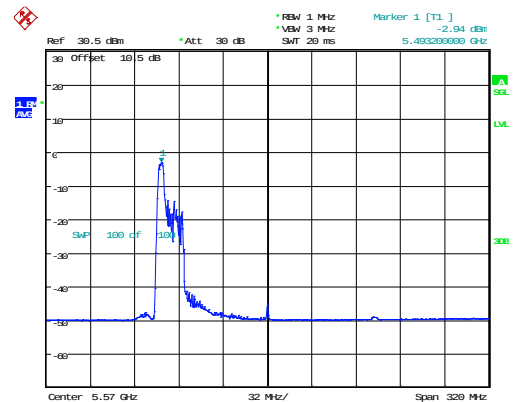
802.11ax160_5570MHz_RU_52/37_Chain 1
