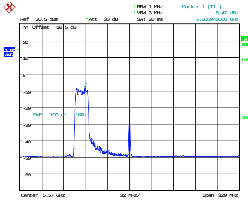
802.11ax160_5570MHz_RU_242/61_Chain 0
