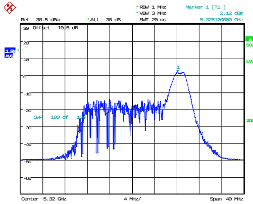
802.11ax20_5320MHz_RU_26/8_Chain 0
