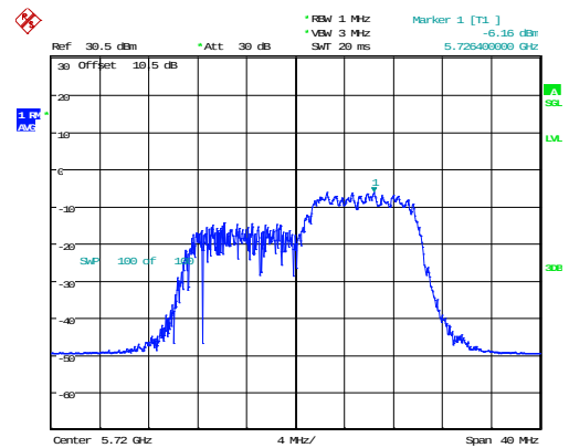
802.11ax20_5720MHz_RU_106/54_Chain 1
