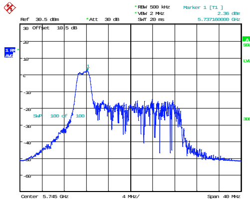
802.11ax20_5745MHz_RU_26/0_Chain 0
