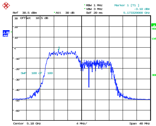
802.11ax20_5180MHz_RU_106/53_Chain 1
