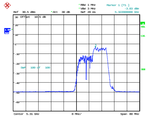
802.11ax40_5310MHz_RU_106/56_Chain 1
