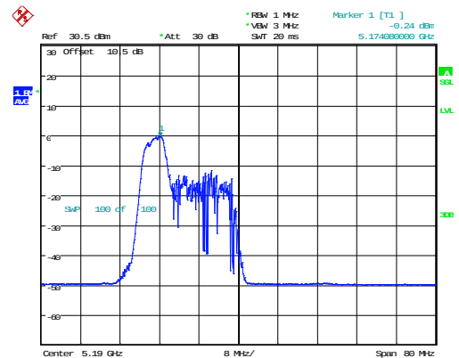
802.11ax40_5190MHz_RU_52/37_Chain 1
