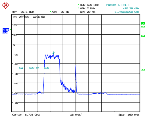
802.11ax80_5775MHz_RU_242/61_Chain 0
