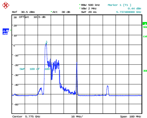
802.11ax80_5775MHz_RU_26/0_Chain 0
