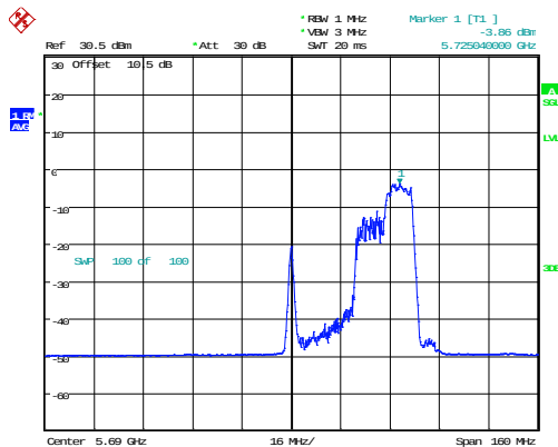
802.11ax80_5690MHz_RU_106/60_Chain 0
