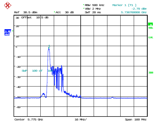
802.11ax80_5775MHz_RU_26/0_Chain 1
