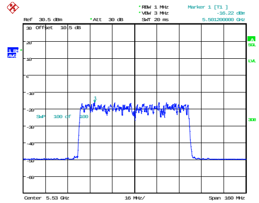
802.11ax80_5530MHz_RU_Full_Chain 1
