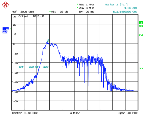
802.11ax20_5180MHz_RU_52/37_Chain 0
