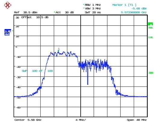
802.11ax20_5580MHz_RU_106/53_Chain 1
