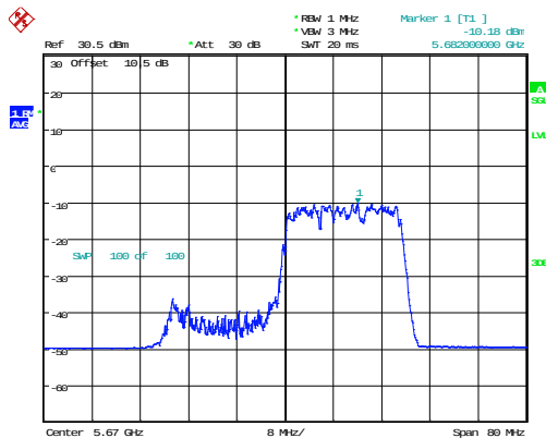
802.11ax40_5670MHz_RU_242/62_Chain 1
