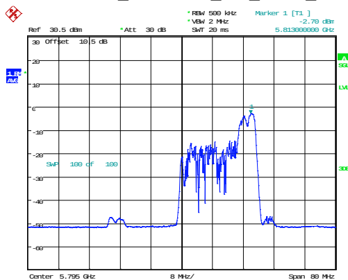
802.11ax40_5795MHz_RU_52/44_Chain 0
