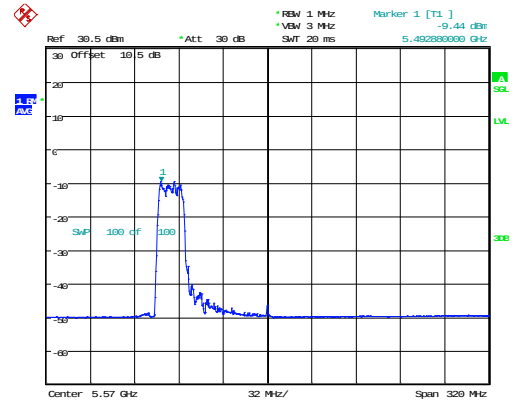
802.11ax160_5570MHz_RU_242/61_Chain 1
