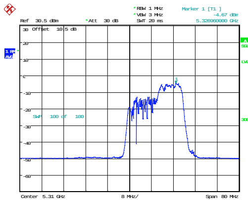
802.11ax40_5310MHz_RU_106/56_Chain 0
