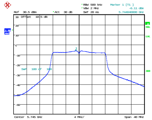
802.11a_5745MHz_Chain 1
