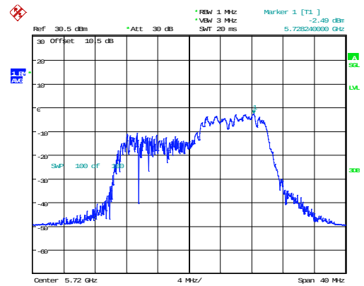
802.11ax20_5720MHz_RU_106/54_Chain 0
