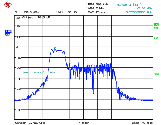
802.11ax20_5785MHz_RU_52/37_Chain 0
