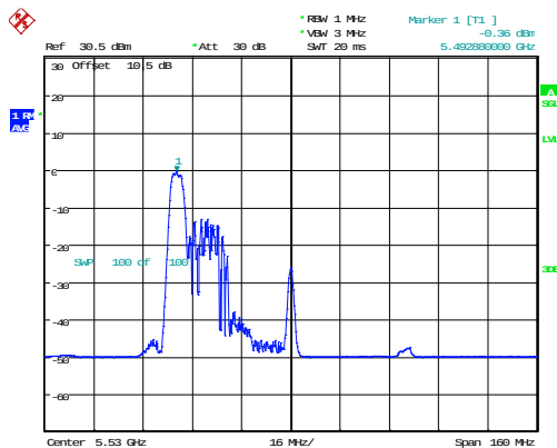
802.11ax80_5530MHz_RU_52/37_Chain 0
