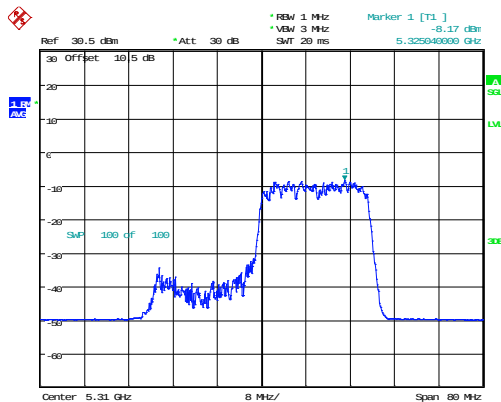
802.11ax40_5310MHz_RU_242/62_Chain 0
