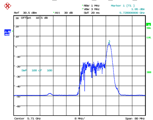
802.11ax40_5710MHz_RU_26/17_Chain 1
