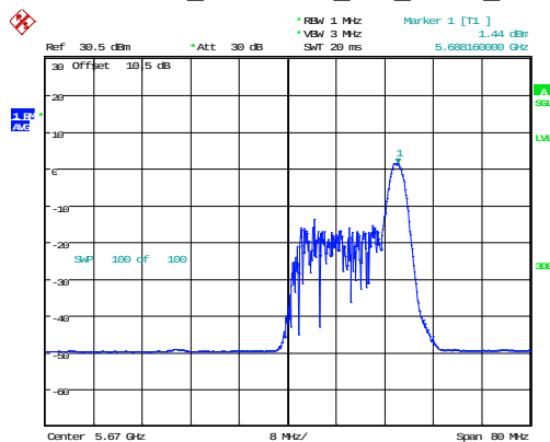
802.11ax40_5670MHz_RU_26/17_Chain 1
