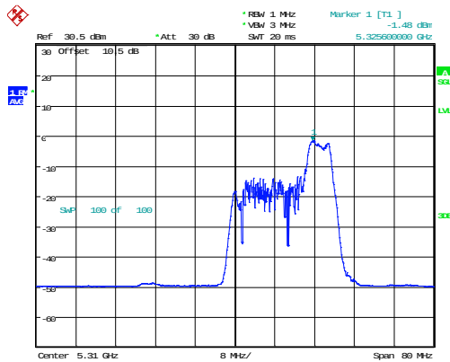
802.11ax40_5310MHz_RU_52/44_Chain 0
