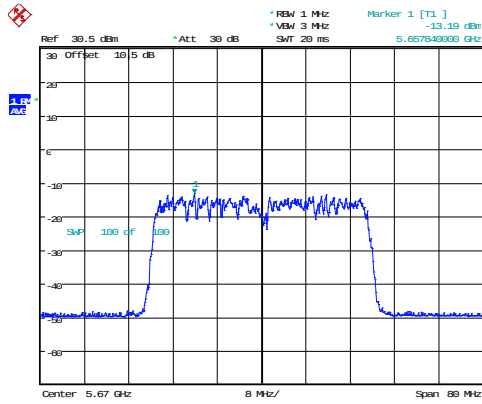
802.11ax40_5670MHz_RU_Full_Chain 1
