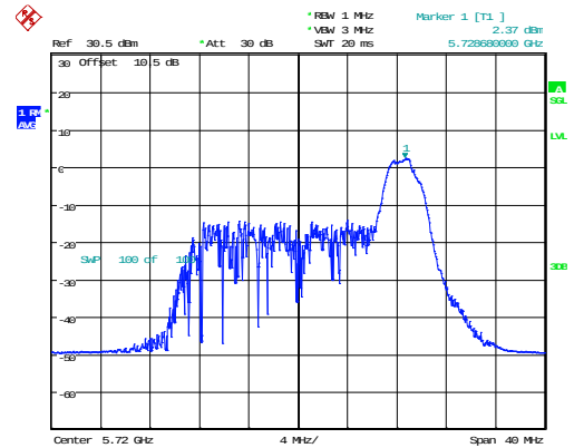
802.11ax20_5720MHz_RU_26/8_Chain 0
