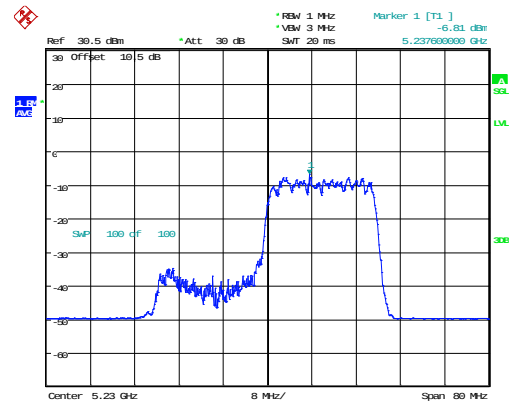
802.11ax40_5230MHz_RU_242/62_Chain 1
