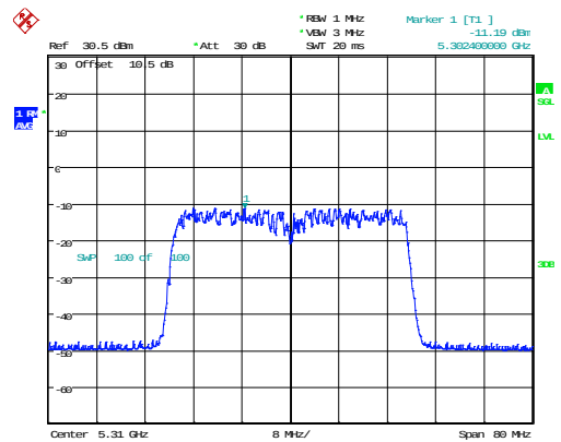
802.11ax40_5310MHz_RU_Full_Chain 1
