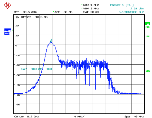
802.11ax20_5200MHz_RU_26/0_Chain 1
