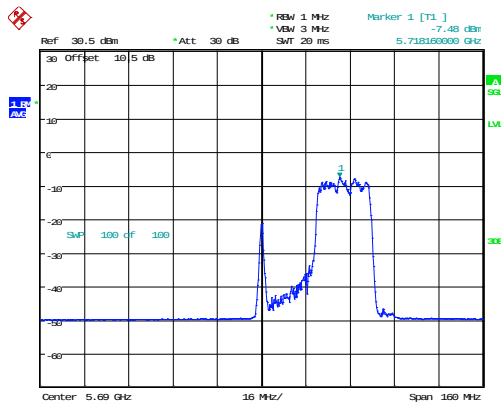
802.11ax80_5690MHz_RU_242/64_Chain 0
