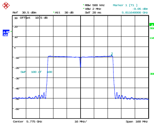
802.11ac80_5775MHz_Chain 0
