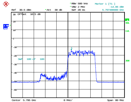
802.11ax40_5795MHz_RU_242/62_Chain 1
