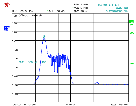
802.11ax40_5190MHz_RU_26/0_Chain 1
