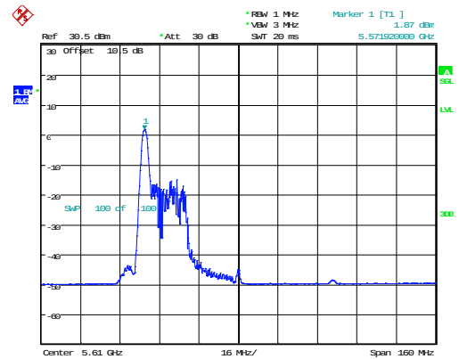
802.11ax80_5610MHz_RU_26/0_Chain 1
