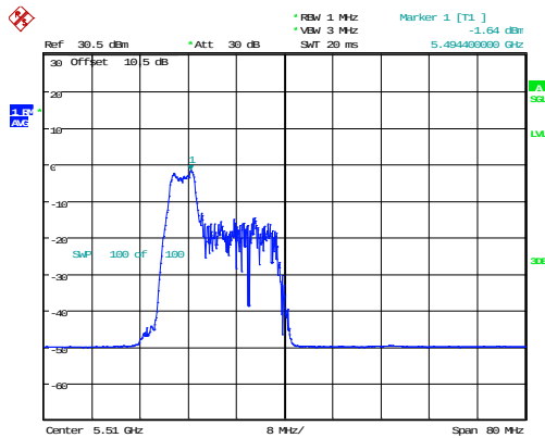
802.11ax40_5510MHz_RU_52/37_Chain 1
