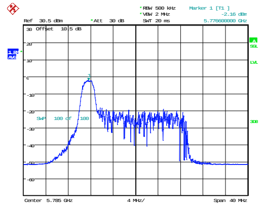
802.11ax20_5785MHz_RU_26/0_Chain 1
