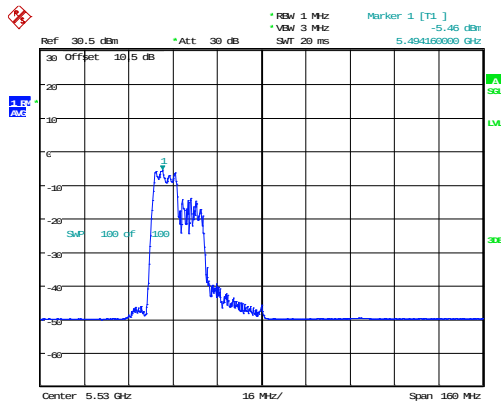
802.11ax80_5530MHz_RU_106/53_Chain 1
