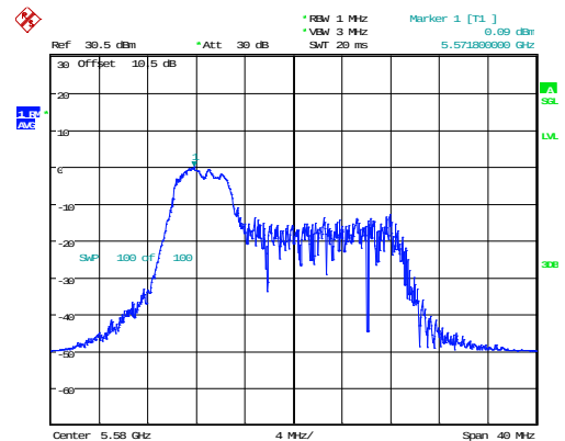
802.11ax20_5580MHz_RU_52/37_Chain 0
