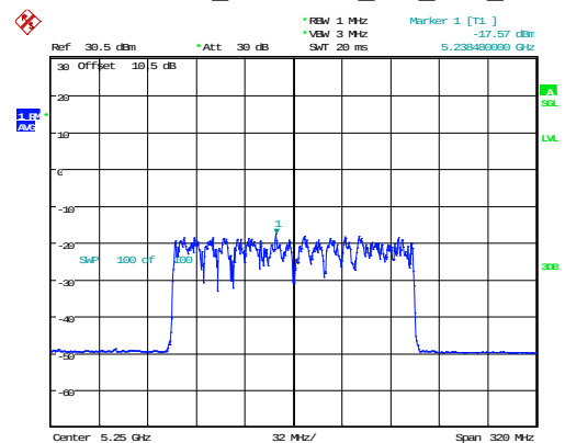
802.11ax160_5250MHz_RU_Full_Chain 1
