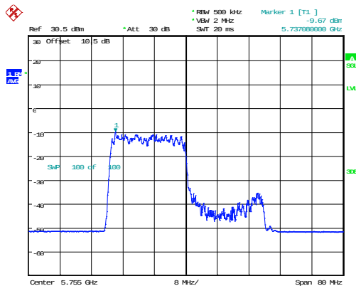
802.11ax40_5755MHz_RU_242/61_Chain 0
