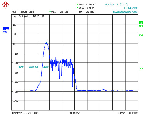
802.11ax40_5270MHz_RU_26/0_Chain 0
