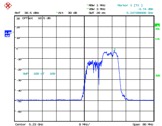
802.11ax40_5230MHz_RU_106/56_Chain 1
