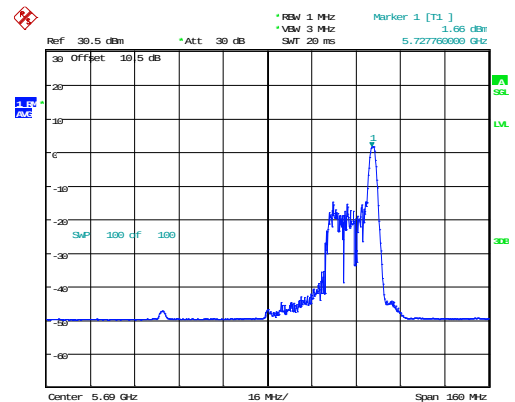
802.11ax80_5690MHz_RU_26/36_Chain 1
