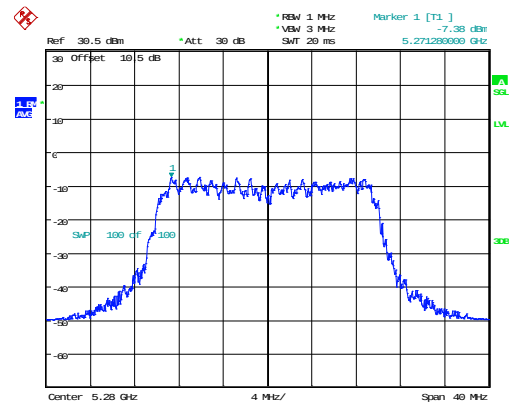
802.11ax20_5280MHz_RU_Full_Chain 0
