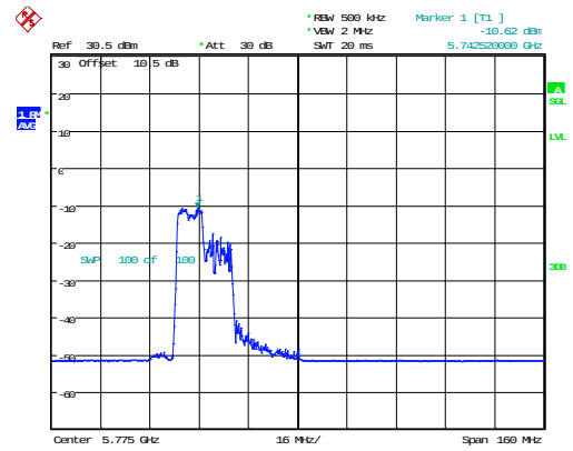
802.11ax80_5775MHz_RU_106/53_Chain 1
