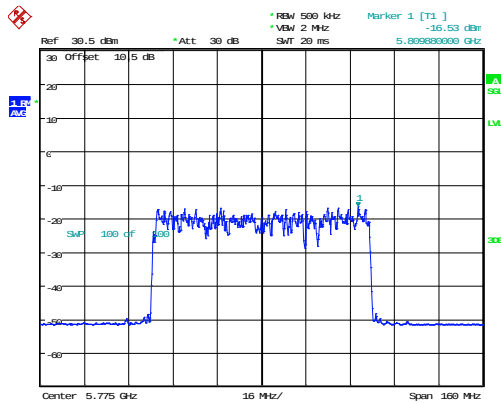
802.11ax80_5775MHz_RU_Full_Chain 0
