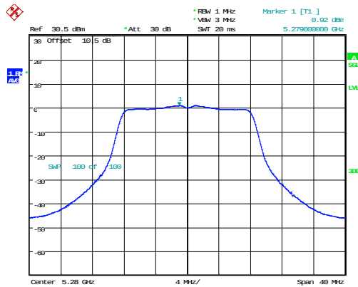
802.11a_5280MHz_Chain 1
