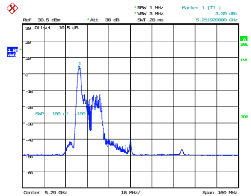
802.11ax80_5290MHz_RU_26/0_Chain 1
