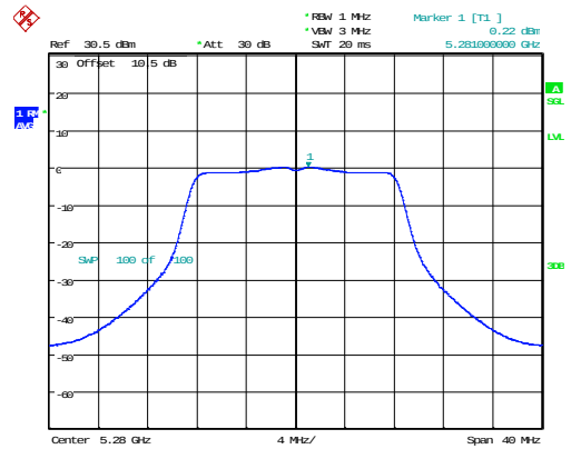
802.11a_5280MHz_Chain 0
