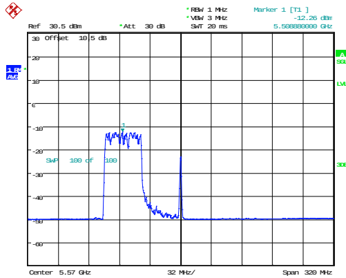
802.11ax160_5570MHz_RU_484/65_Chain 0
