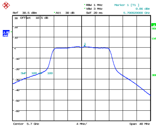
802.11a_5700MHz_Chain 0
