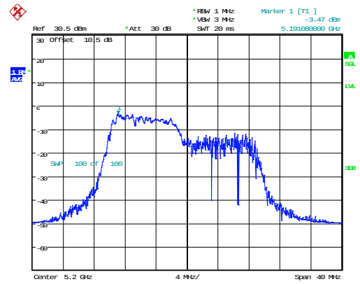
802.11ax20_5200MHz_RU_106/53_Chain 0
