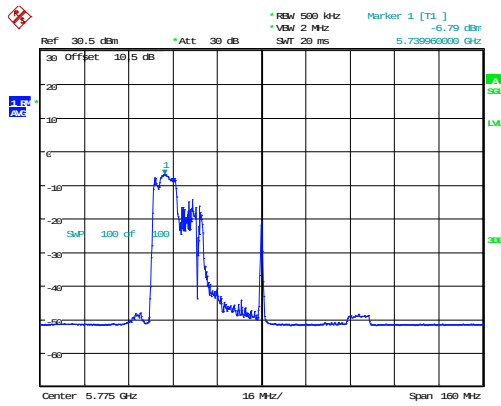
802.11ax80_5775MHz_RU_106/53_Chain 0
