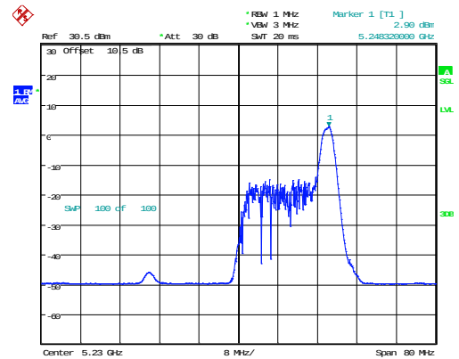
802.11ax40_5230MHz_RU_26/17_Chain 1
