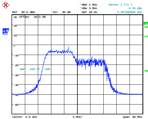
802.11ax20_5500MHz_RU_106/53_Chain 1
