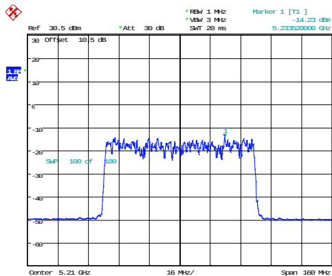
802.11ax80_5210MHz_RU_Full_Chain 0
