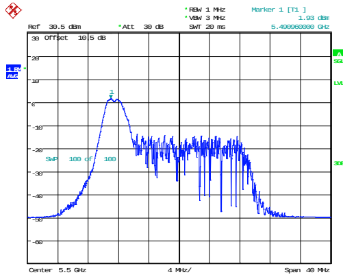
802.11ax20_5500MHz_RU_26/0_Chain 0
