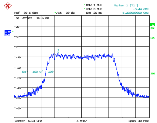
802.11ax20_5240MHz_RU_Full_Chain 1
