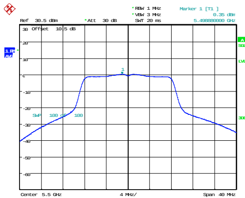
802.11a_5500MHz_Chain 0
