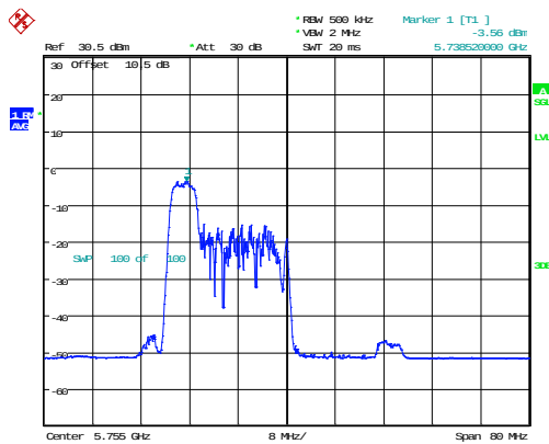
802.11ax40_5755MHz_RU_52/37_Chain 0
