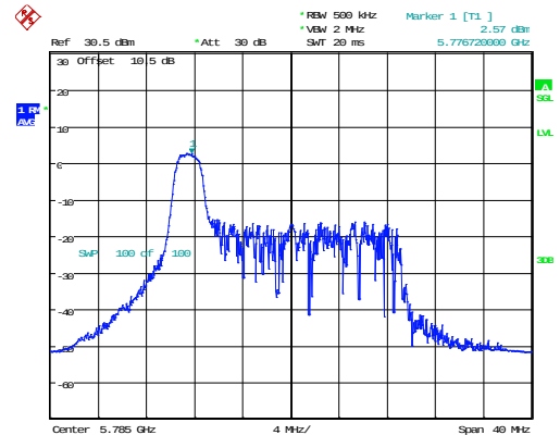
802.11ax20_5785MHz_RU_26/0_Chain 0
