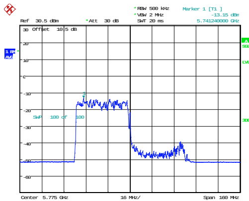
802.11ax80_5775MHz_RU_484/65_Chain 0
