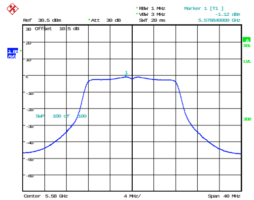
802.11a_5580MHz_Chain 1
