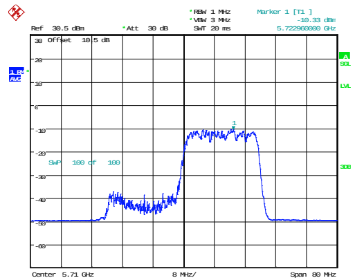
802.11ax40_5710MHz_RU_242/62_Chain 1
