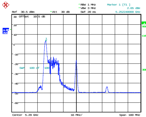
802.11ax80_5290MHz_RU_26/0_Chain 0
