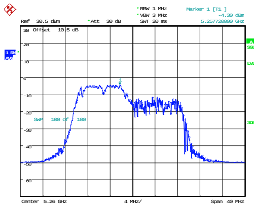
802.11ax20_5260MHz_RU_106/53_Chain 1
