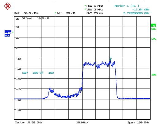
802.11ax80_5690MHz_RU_484/66_Chain 1
