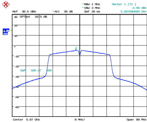
802.11n40_5670MHz_Chain 1
