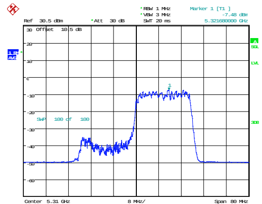
802.11ax40_5310MHz_RU_242/62_Chain 1
