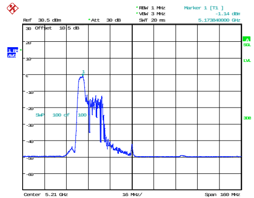
802.11ax80_5210MHz_RU_52/37_Chain 1
