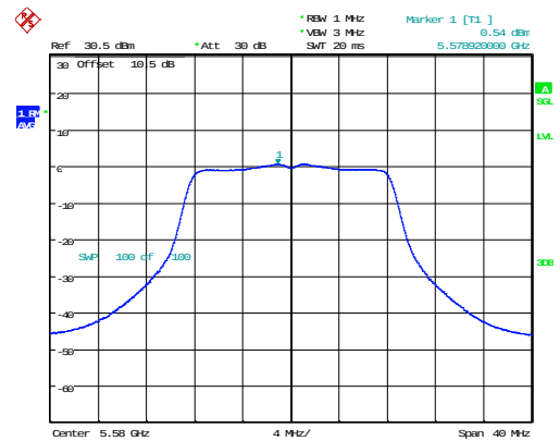
802.11a_5580MHz_Chain 0
