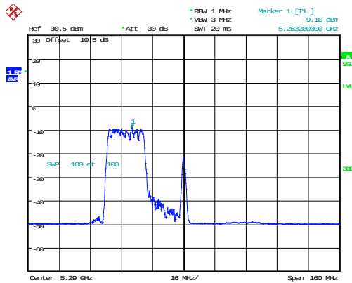
802.11ax80_5290MHz_RU_242/61_Chain 0
