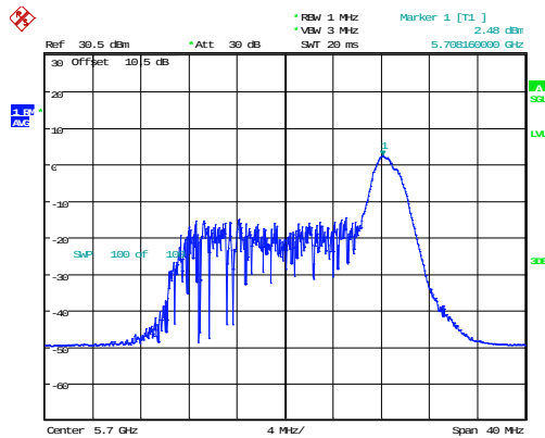
802.11ax20_5700MHz_RU_26/8_Chain 1
