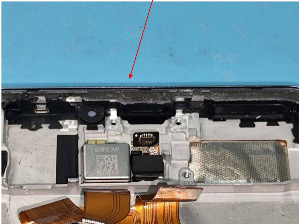
ANT3 MHB PRX
