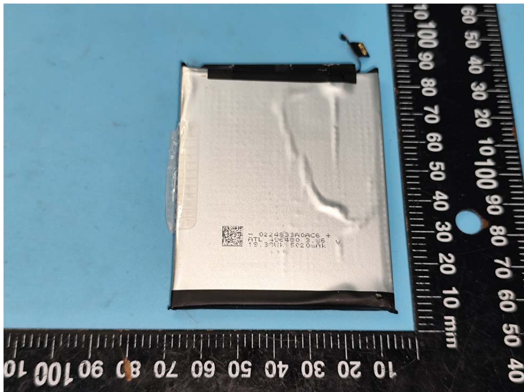
battery
