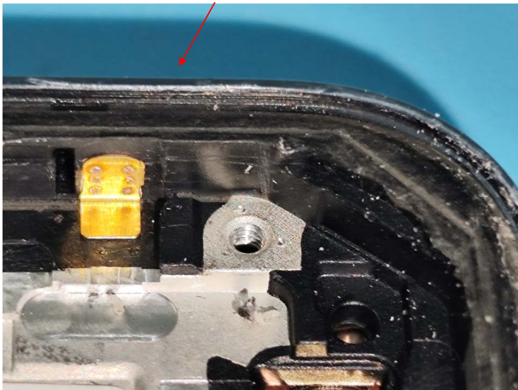
ANT0 n77/78 PRX2 + 5G Wi-Fi Chain 0
