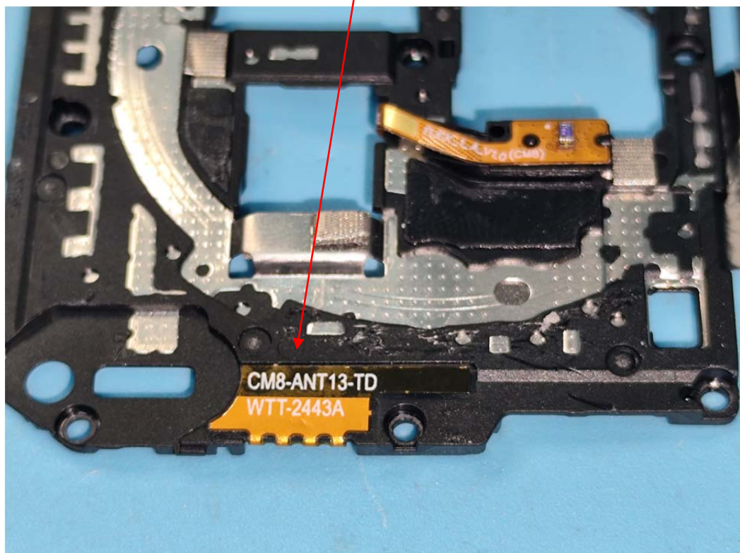
ANT13 5G Wi-Fi Chain 1
