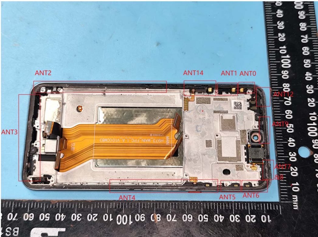
ANT position
