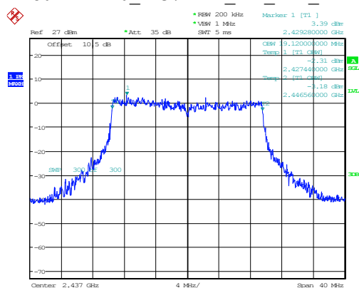
802.11ax20 2437MHz RU Full Chain 0
