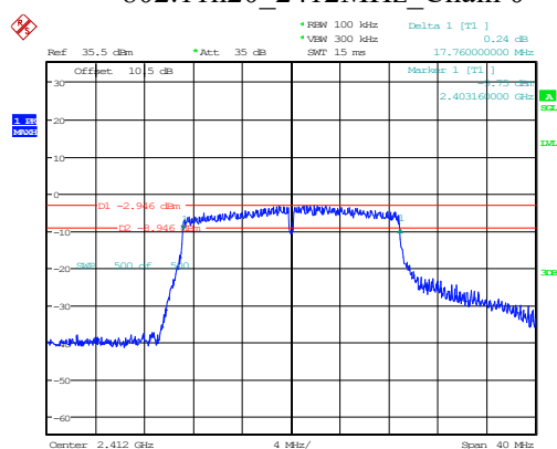
802.11n20 2412MHz Chain 0
