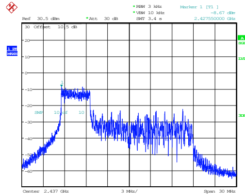
802.11ax20_2437MHz_RU_52/37_Chain 0
