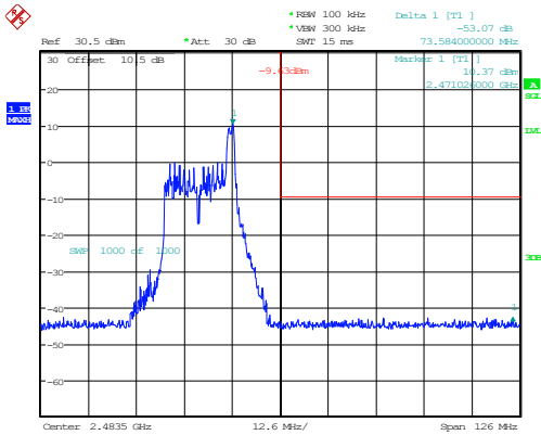
802.11ax20_2462MHz_RU_26/8_Chain 0
