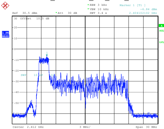
802.11ax20_2412MHz_RU_26/0_Chain 1
