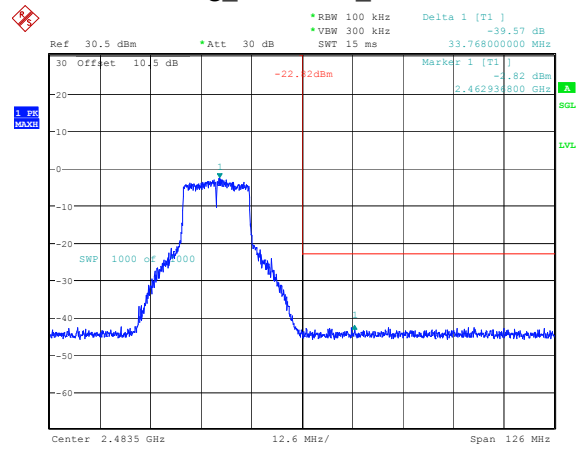
802.11g_2462MHz_Chain 1
