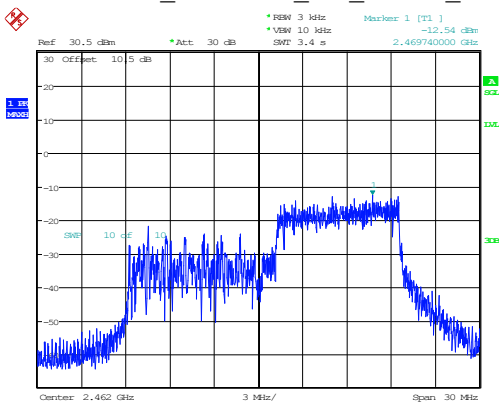
802.11ax20_2462MHz_RU_106/54_Chain 0
