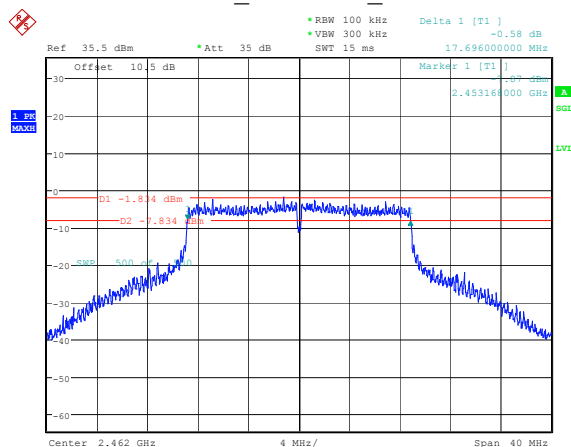
802.11n20 2462MHz Chain 1
