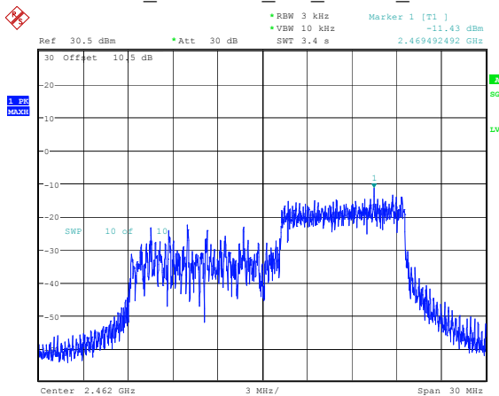
802.11ax20_2462MHz_RU_106/54_Chain 1
