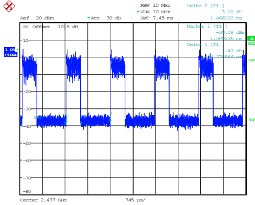
802.11ax20_2437MHz_RU_52/37_Chain 0
