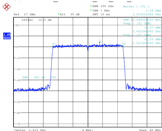
802.11ax20 2412MHz RU Full Chain 1
