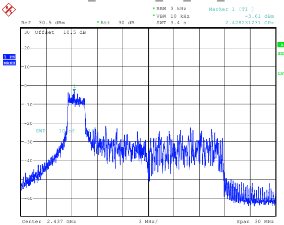
802.11ax20_2437MHz_RU_26/0_Chain 1
