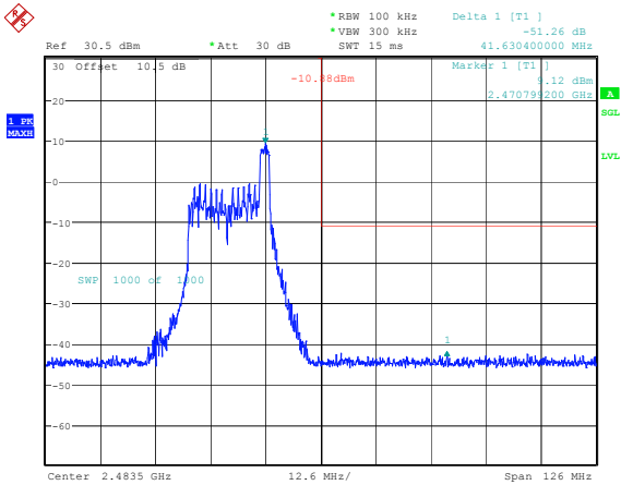
802.11ax20_2462MHz_RU_26/8_Chain 1
