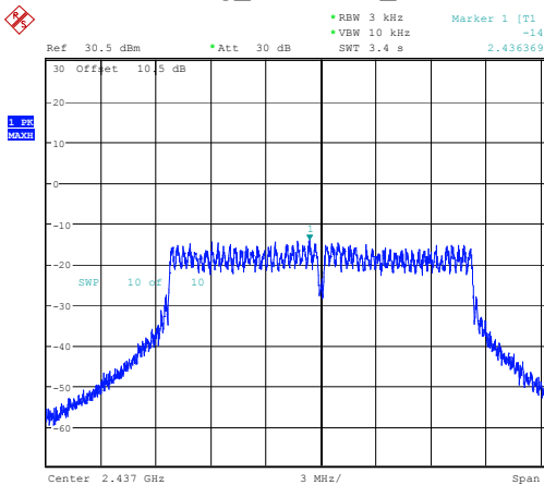
802.11g_2437MHz_Chain 1
