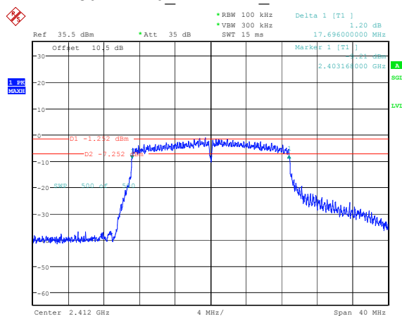
802.11n20 2412MHz Chain 1
