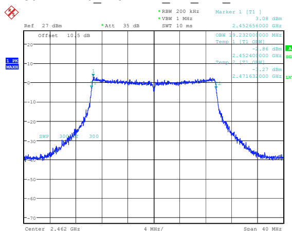
802.11ax20 2462MHz RU Full Chain 1
