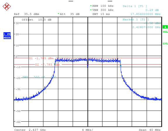
802.11n20 2437MHz Chain 1
