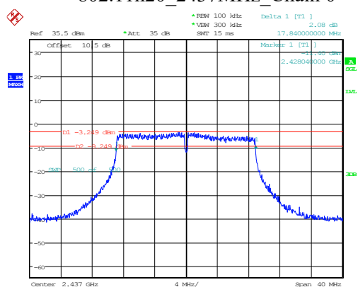
802.11n20 2437MHz Chain 0
