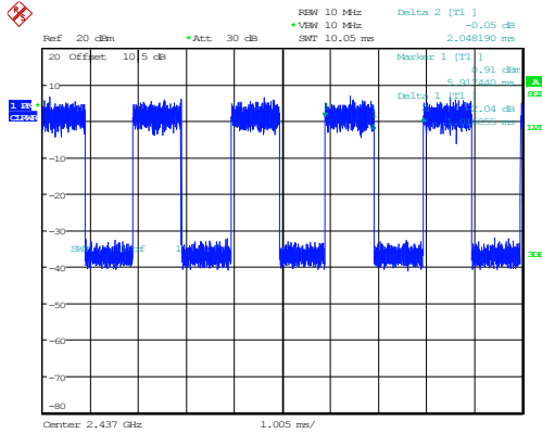
802.11ax20_2437MHz_RU_Full_Chain 0
