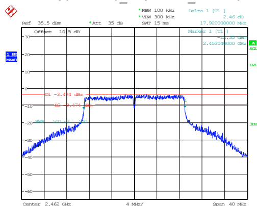
802.11n20 2462MHz Chain 0
