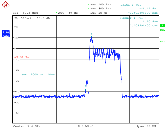
802.11ax20_2412MHz_RU_26/0_Chain 1
