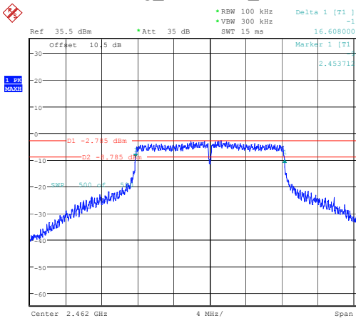
802.11g_2462MHz_Chain 1
