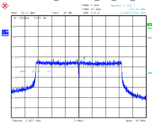
802.11ax20_2437MHz_RU_Full_Chain 1
