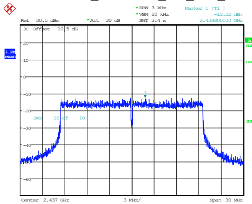
802.11ax20_2437MHz_RU_Full_Chain 0
