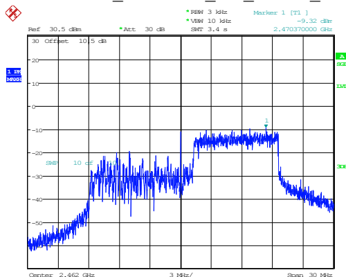
802.11ax20_2462MHz_RU_106/54_Chain 1
