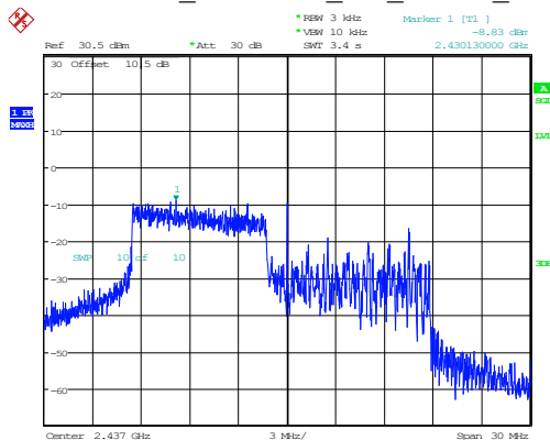
802.11ax20_2437MHz_RU_106/53_Chain 1
