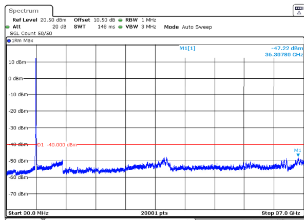
n77_2_60MHz_30kHz_3670MHz_DFT-s-OFDM QPSK_RB162@0 -47.22dBm
