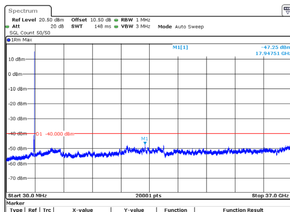
n77_2_70MHz_30kHz_3585MHz_DFT-s-OFDM QPSK_RB1@188 -47.25dBm
