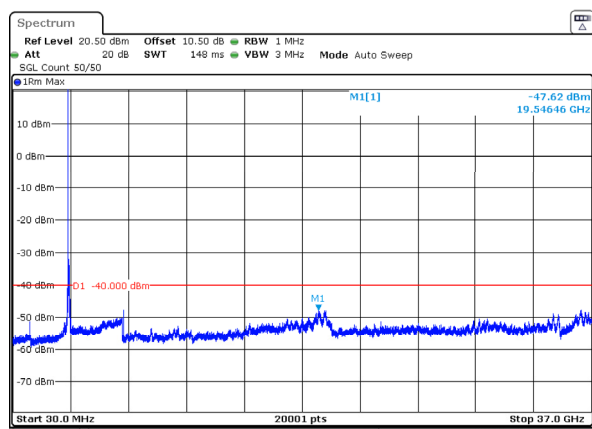
n77_2_70MHz_30kHz_3585MHz_DFT-s-OFDM QPSK_RB1@0 -47.62dBm
