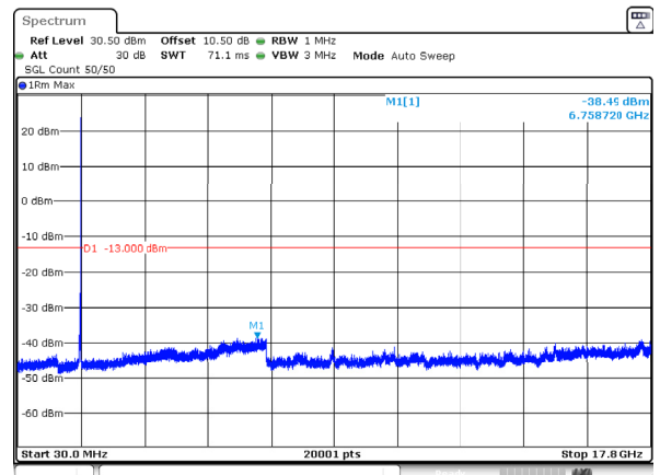
n66_25MHz_15kHz_1767.5MHz_DFT-s-OFDM QPSK_RB1@132 -38.49dBm
