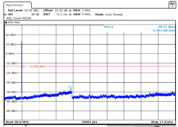
n66_15MHz_15kHz_1772.5MHz_DFT-s-OFDM QPSK_RB75@0 -38.22dBm
