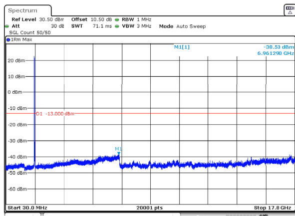
n66_30MHz_15kHz_1765MHz_DFT-s-OFDM QPSK_RB1@0 -38.53dBm
