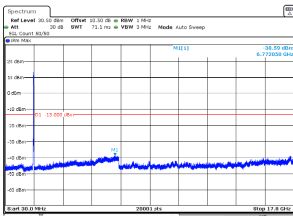
n66_20MHz_15kHz_1770MHz_DFT-s-OFDM QPSK_RB100@0 -38.59dBm
