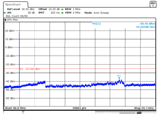
n7_5MHz_15kHz_2535MHz_DFT-s-OFDM QPSK_RB1@0 -36.95dBm
