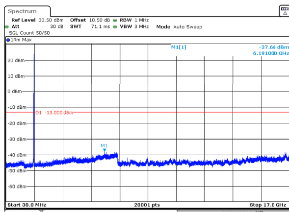
n66_15MHz_15kHz_1745MHz_DFT-s-OFDM QPSK_RB1@78 -37.66dBm
