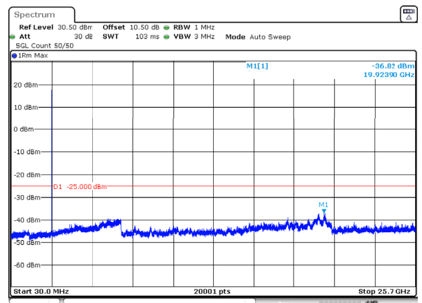
n7_5MHz_15kHz_2567.5MHz_DFT-s-OFDM QPSK_RB1@24 -36.82dBm
