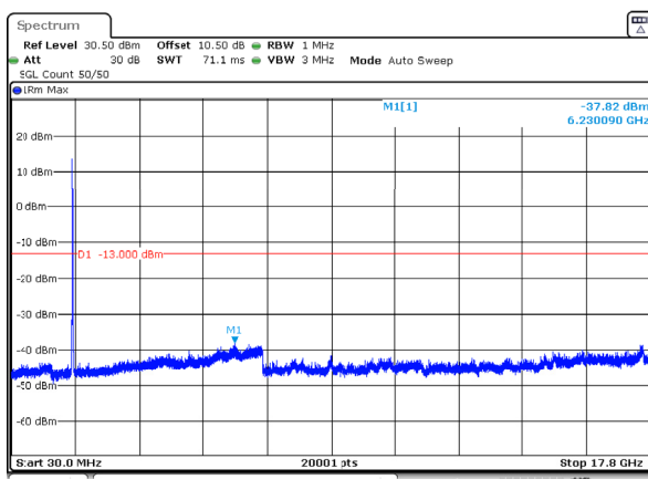
n66_20MHz_15kHz_1720MHz_DFT-s-OFDM QPSK_RB100@0 -37.82dBm
