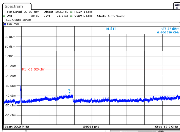
n66_30MHz_15kHz_1745MHz_DFT-s-OFDM QPSK_RB160@0 -37.72dBm
