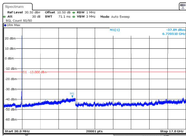
n66_30MHz_15kHz_1745MHz_DFT-s-OFDM QPSK_RB1@159 -37.89dBm
