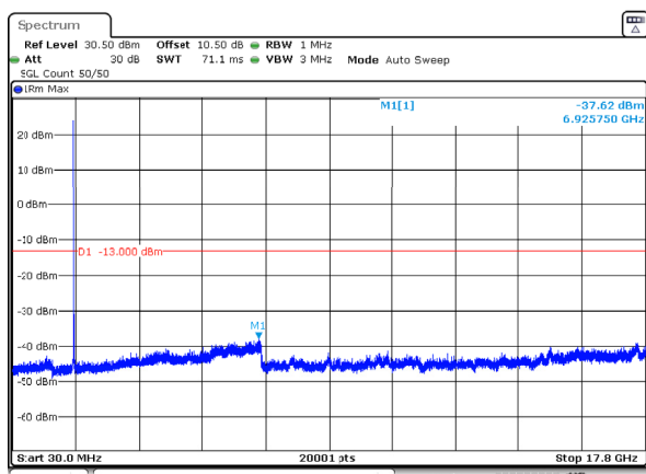
n66_15MHz_15kHz_1745MHz_DFT-s-OFDM QPSK_RB1@0 -37.62dBm
