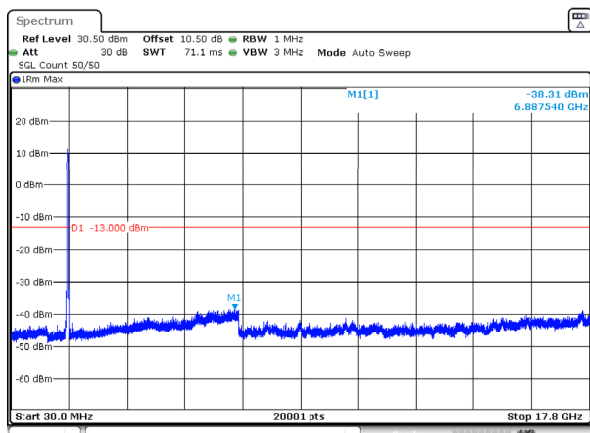
n66_30MHz_15kHz_1765MHz_DFT-s-OFDM QPSK_RB160@0 -38.31dBm
