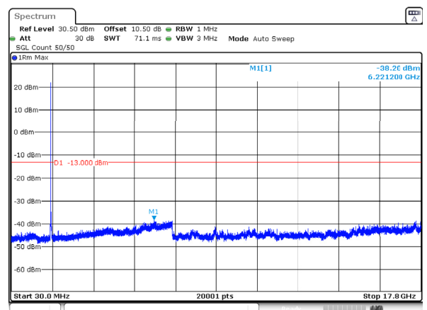
n66_30MHz_15kHz_1725MHz_DFT-s-OFDM QPSK_RB1@0 -38.20dBm
