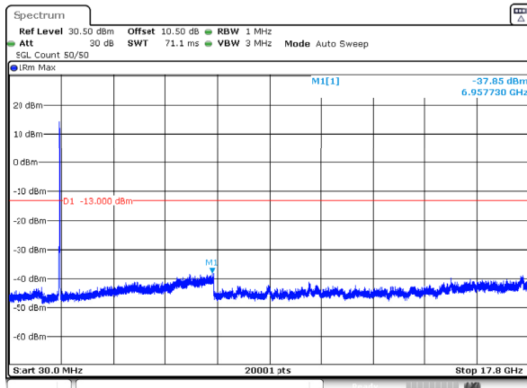
n66_15MHz_15kHz_1745MHz_DFT-s-OFDM QPSK_RB75@0 -37.85dBm
