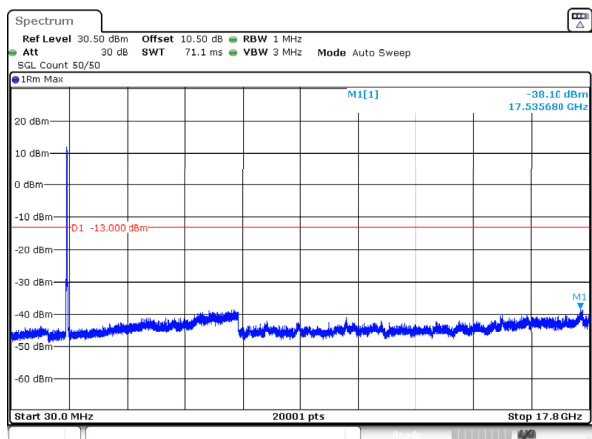
n66_25MHz_15kHz_1722.5MHz_DFT-s-OFDM QPSK_RB128@0 -38.10dBm
