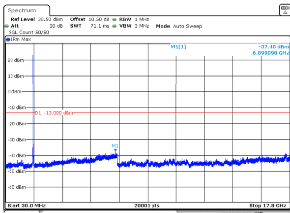
n66_30MHz_15kHz_1745MHz_DFT-s-OFDM QPSK_RB1@0 -37.40dBm
