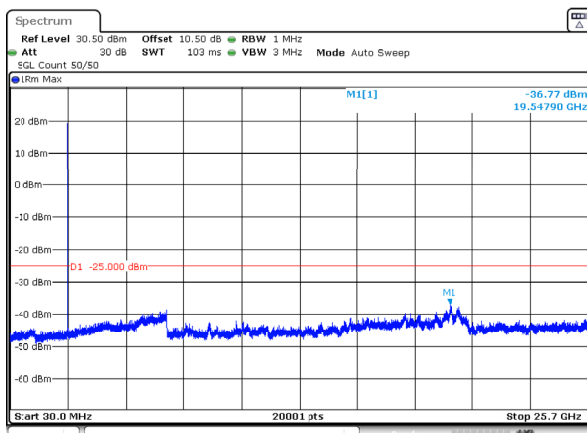
n7_5MHz_15kHz_2567.5MHz_DFT-s-OFDM QPSK_RB1@0 -36.77dBm
