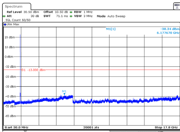
n66_15MHz_15kHz_1717.5MHz_DFT-s-OFDM QPSK_RB1@78 -38.34dBm
