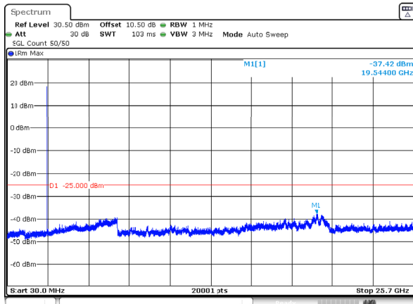
n7_5MHz_15kHz_2535MHz_DFT-s-OFDM QPSK_RB1@24 -37.42dBm
