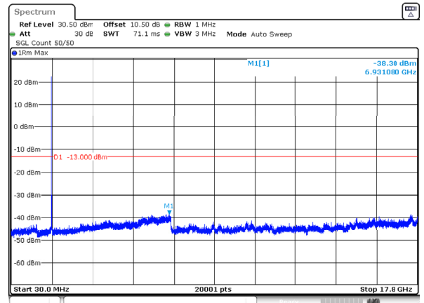
n66_15MHz_15kHz_1772.5MHz_DFT-s-OFDM QPSK_RB1@0 -38.30dBm
