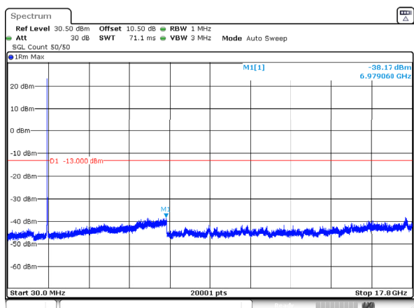
n66_25MHz_15kHz_1745MHz_DFT-s-OFDM QPSK_RB1@0 -38.17dBm
