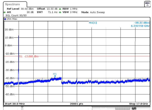
n66_25MHz_15kHz_1767.5MHz_DFT-s-OFDM QPSK_RB128@0 -38.32dBm
