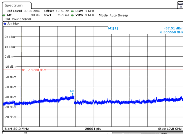
n66_15MHz_15kHz_1772.5MHz_DFT-s-OFDM QPSK_RB1@78 -37.51dBm
