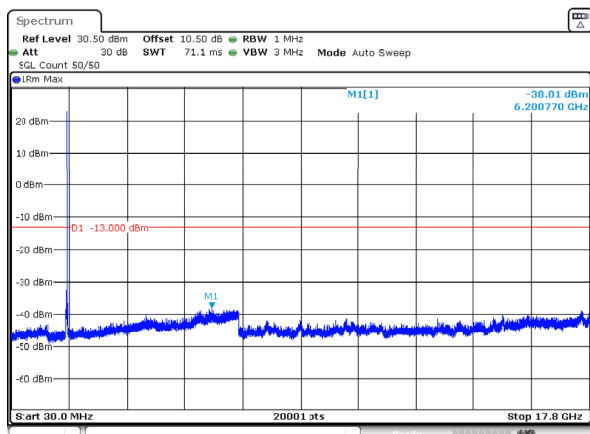
n66_30MHz_15kHz_1725MHz_DFT-s-OFDM QPSK_RB1@159 -38.01dBm
