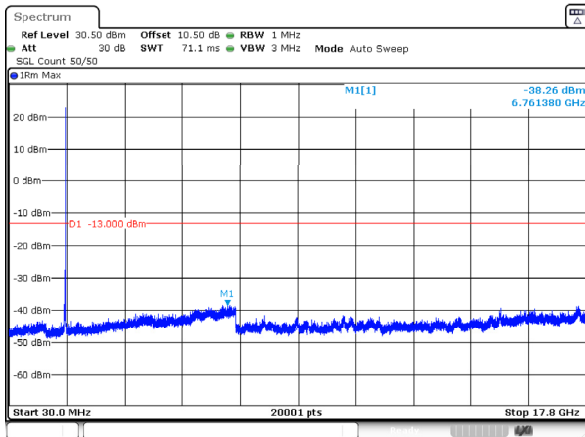
n66_25MHz_15kHz_1745MHz_DFT-s-OFDM QPSK_RB1@132 -38.26dBm
