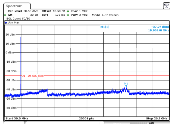
n41_80MHz_30kHz_2536.02MHz_DFT-s-OFDM QPSK_RB1@216 -37.22dBm
