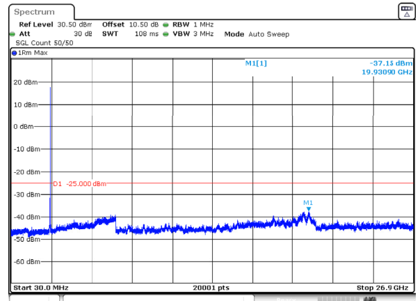
n41_50MHz_30kHz_2592.99MHz_DFT-s-OFDM QPSK_RB1@132 -37.15dBm
