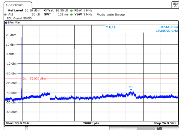
n41_100MHz_30kHz_2592.99MHz_DFT-s-OFDM QPSK_RB1@0 -37.65dBm
