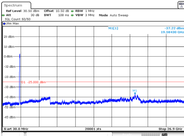
n41_100MHz_30kHz_2546.01MHz_DFT-s-OFDM QPSK_RB270@0 -37.22dBm
