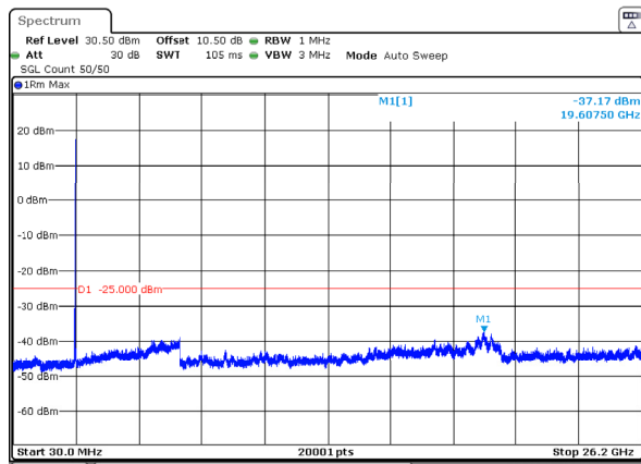
n38_30MHz_30kHz_2605MHz_DFT-s-OFDM QPSK_RB1@77 -37.17dBm
