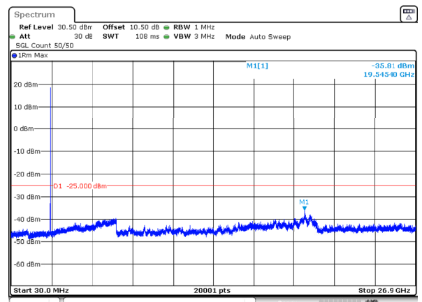
n41_20MHz_30kHz_2592.99MHz_DFT-s-OFDM QPSK_RB1@50 -35.81dBm
