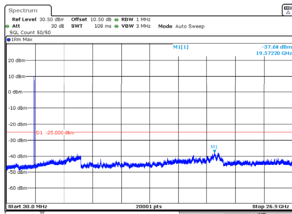
n41_15MHz_30kHz_2592.99MHz_DFT-s-OFDM QPSK_RB36@0 -37.60dBm
