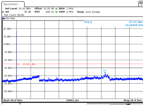
n41_20MHz_30kHz_2679.99MHz_DFT-s-OFDM QPSK_RB1@50 -37.22dBm
