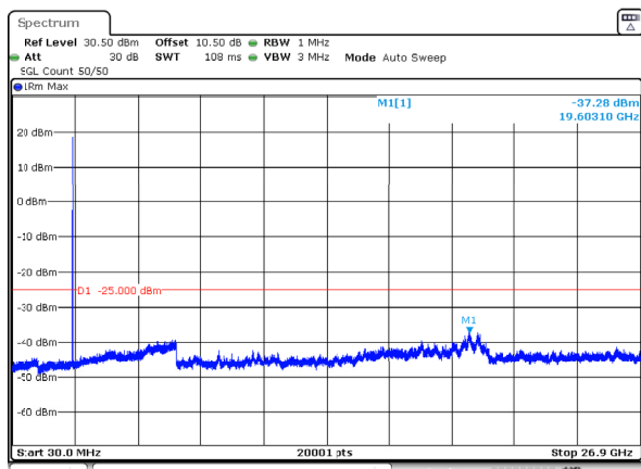
n41_15MHz_30kHz_2592.99MHz_DFT-s-OFDM QPSK_RB1@37 -37.28dBm
