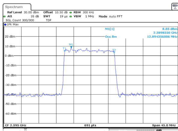
n38_15MHz_30kHz_2595MHz_DFT-s-OFDM 256 QAM_RB36@0
