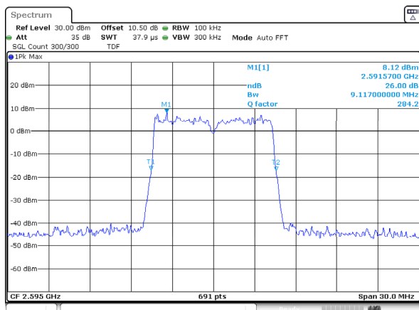
n38_10MHz_30kHz_2595MHz_DFT-s-OFDM 16 QAM_RB24@0
