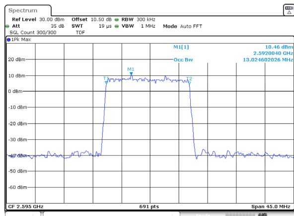
n38_15MHz_30kHz_2595MHz_DFT-s-OFDM 64 QAM_RB36@0
