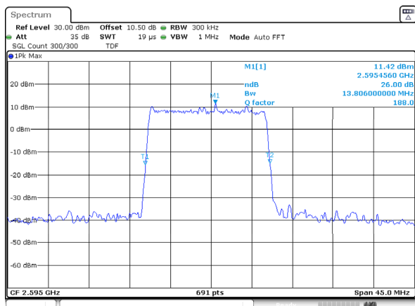
n38_15MHz_30kHz_2595MHz_DFT-s-OFDM 16 QAM_RB36@0
