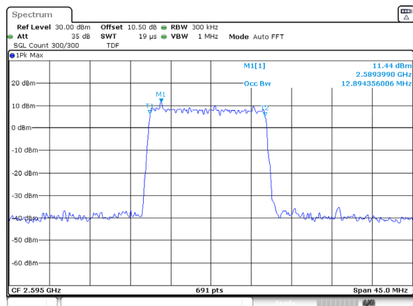
n38_15MHz_30kHz_2595MHz_DFT-s-OFDM 16 QAM_RB36@0
