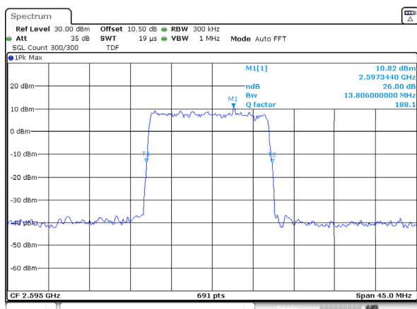
n38_15MHz_30kHz_2595MHz_DFT-s-OFDM 64 QAM_RB36@0
