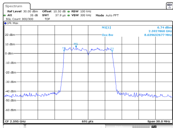
n38_10MHz_30kHz_2595MHz_DFT-s-OFDM 16 QAM_RB24@0
