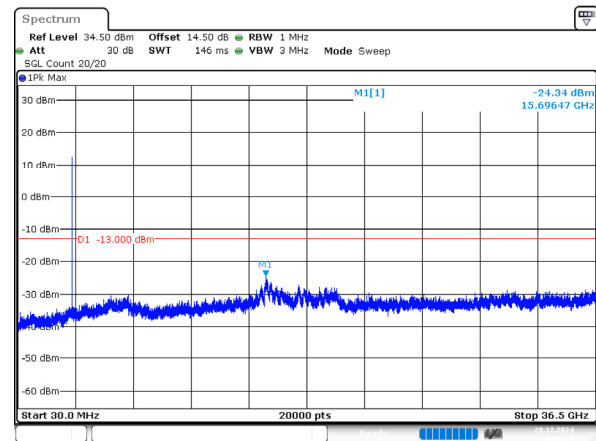
1_10MHz_Low_QPSK_1@0(30MHz~36.5GHz)
