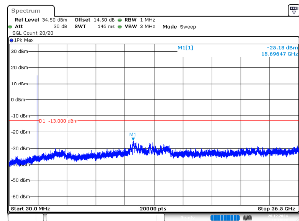
1_10MHz_High_QPSK_1@0(30MHz~36.5GHz)
