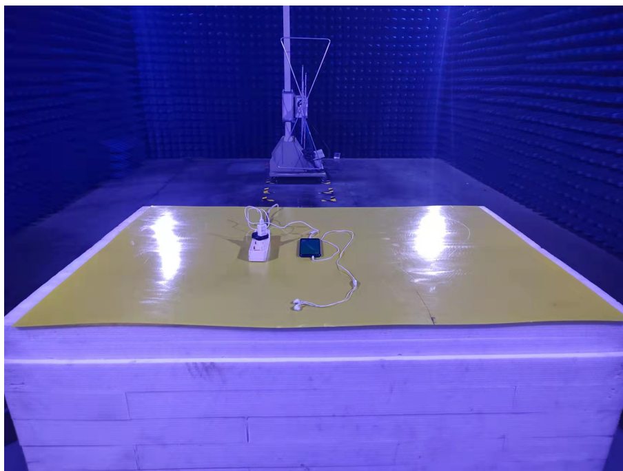
Photo of Radiated Emission Measurement (30MHz-1GHz)
