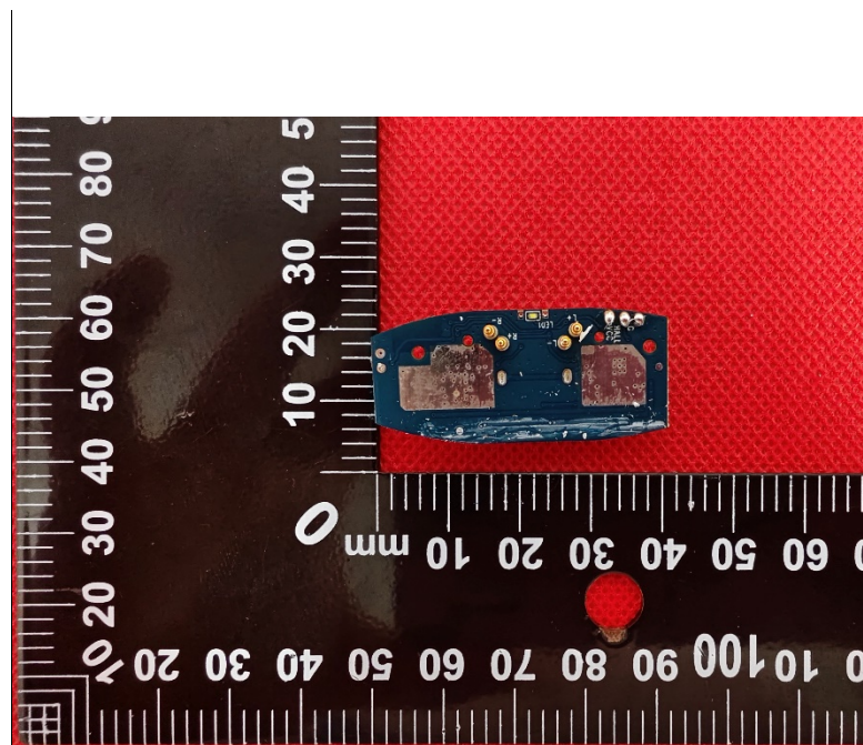
Internal photograph of EUT
