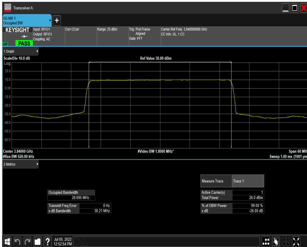
n77(3700-3980) SCS=15kHz DFT_QPSK BW=30MHz Channel=656000 RB=160@0
