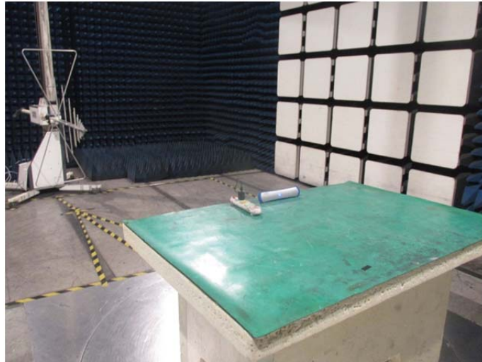
Photo of Radiated Emission Measurement
