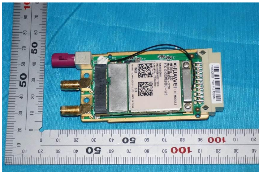
ME909u-523(4G):
