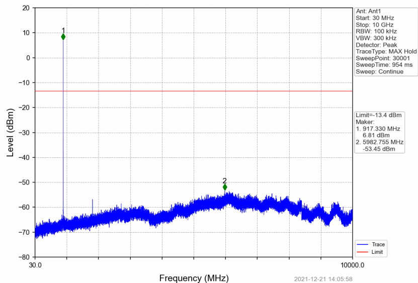
P_HCH_917.4MHz_Ant1_NTNV
