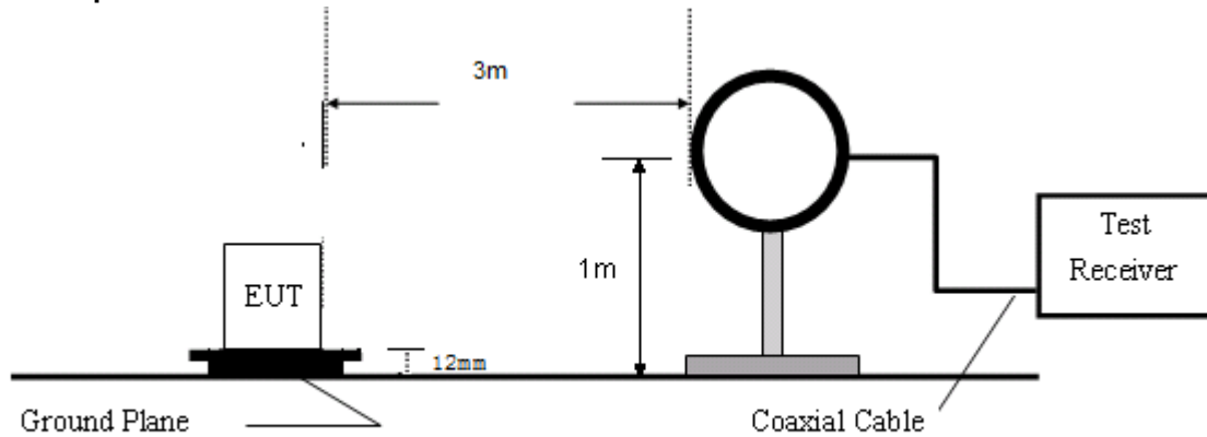
Figure1. Blow 30MHz radiated emissions test configuration
