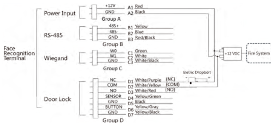
Figure 4-4 Wire Device
