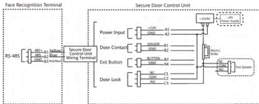
Figure 4-9 Wiring Diagram
