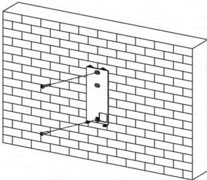
Figure 3-2 Install Mounting Plate
