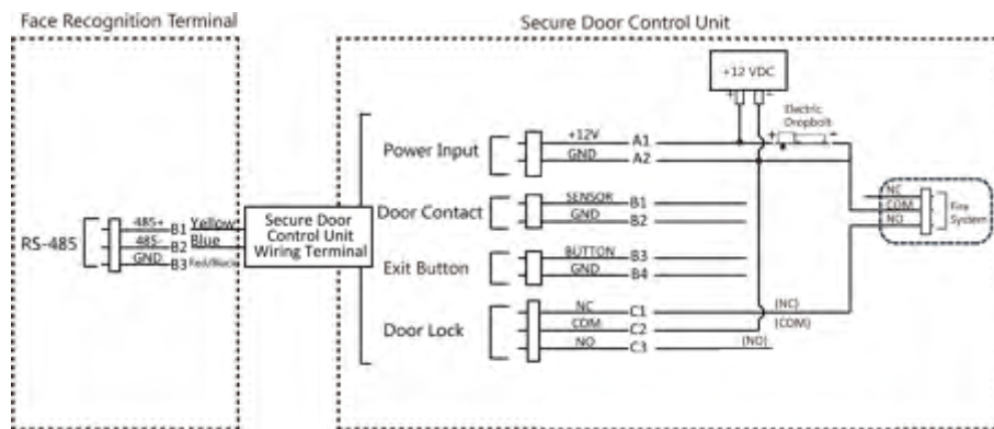
Figure 4-7 Wiring Secure Door Control Unit
