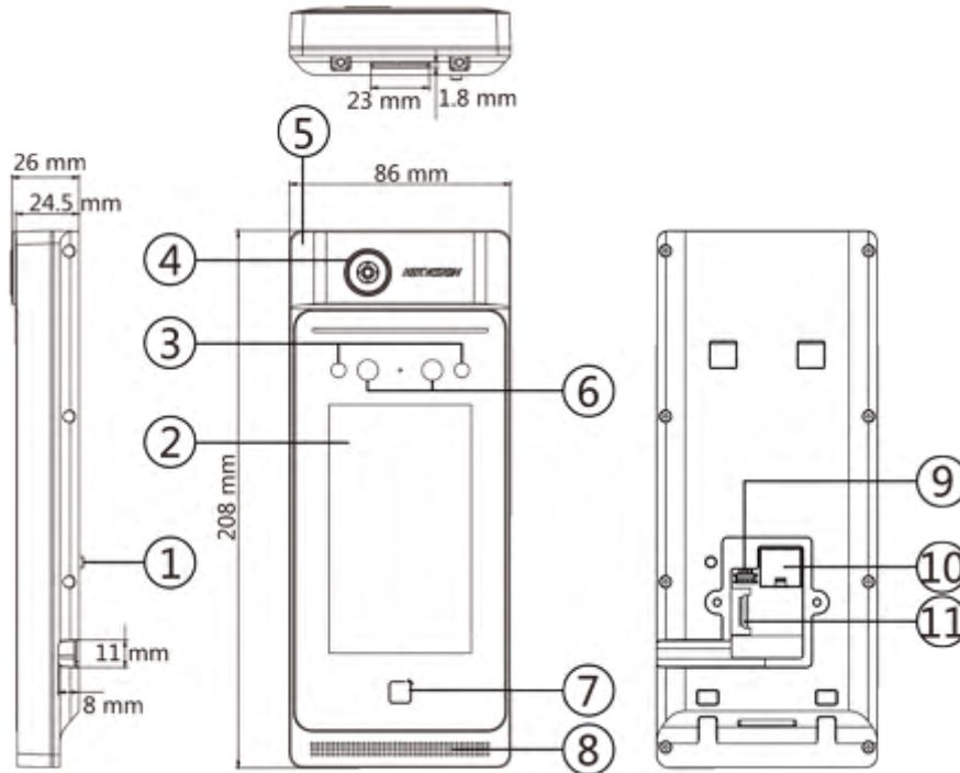
Figure 2-1 Face Recognition Terminal Diagram
