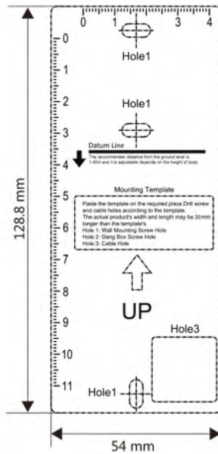
Figure 3-4 Mounting Template
