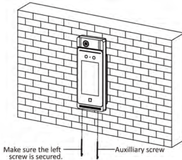
Figure 3-3 Secure Device
