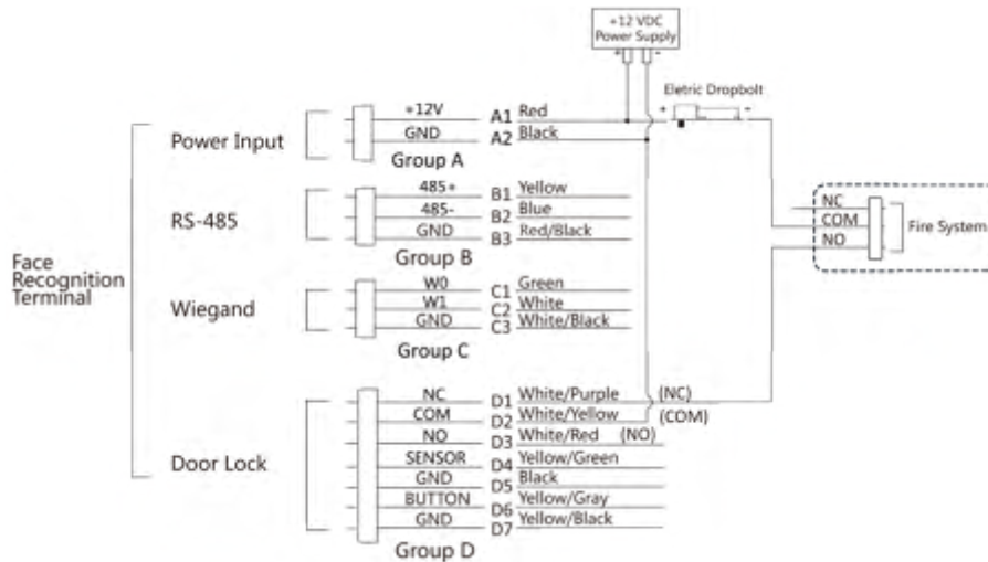
Figure 4-6 Wiring Device
