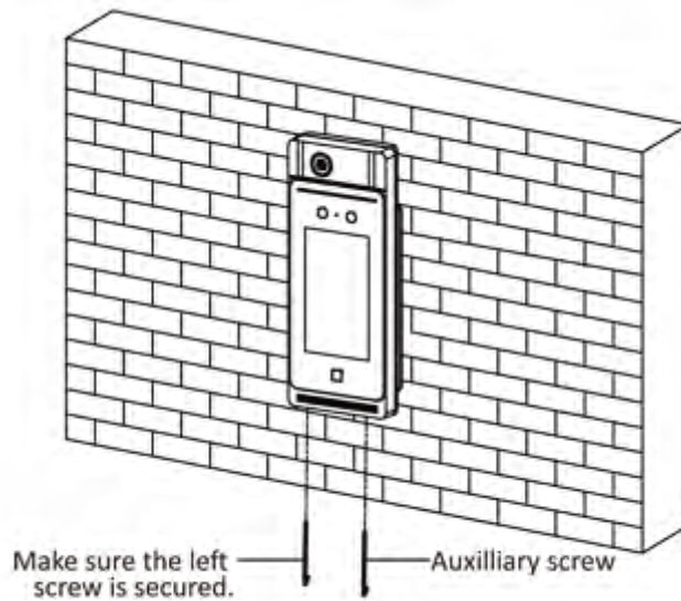
Figure 3-6 Secure Device
