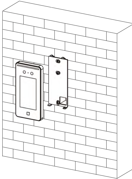
Figure 3-22 Install Device
