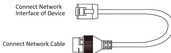
Figure 4-8 Cable Diagram
