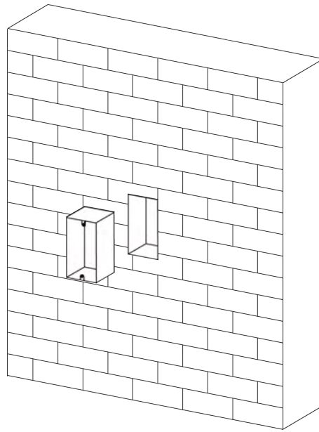
Figure 3-13 Install Gang Box
