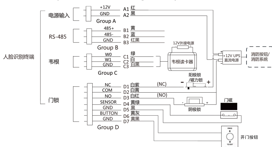
Figure 4-3 Device Wiring
