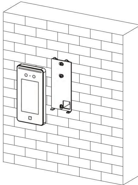
Figure 3-16 Install Device
