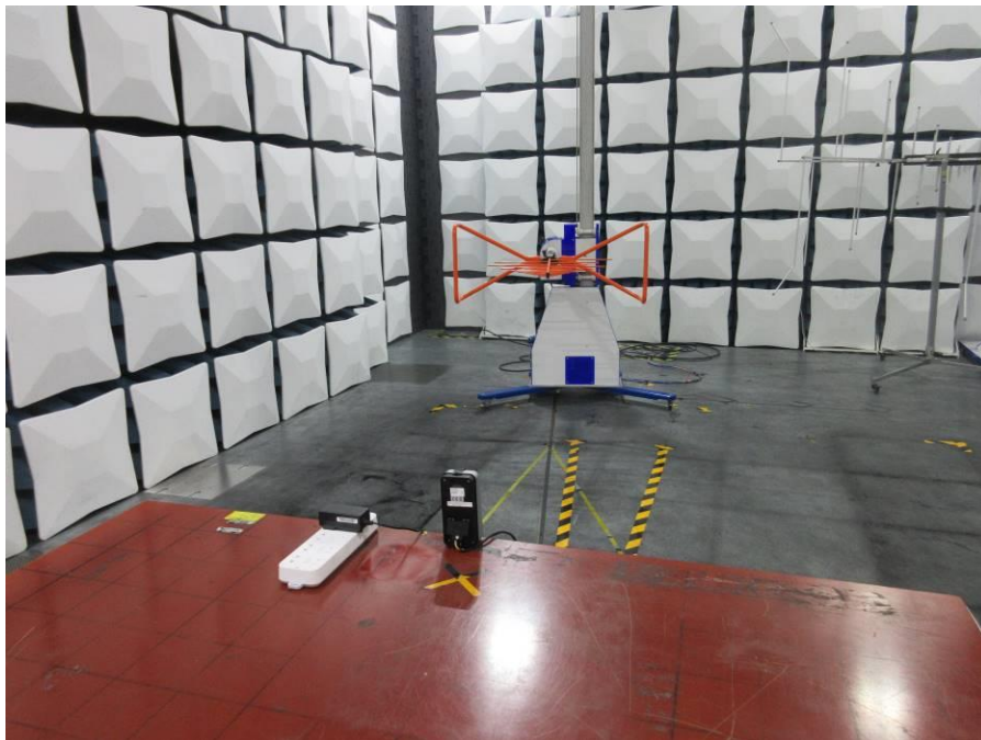
RADIATED RF MEASUREMENT SETUP (30MHz ~ 1 GHz)-Z
