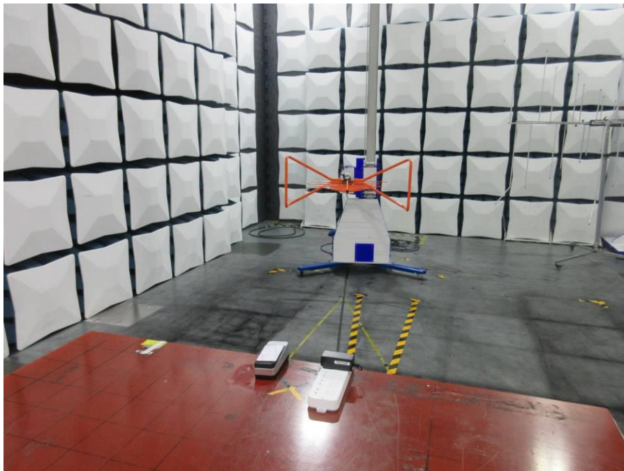
RADIATED RF MEASUREMENT SETUP (30MHz ~ 1 GHz)-X
