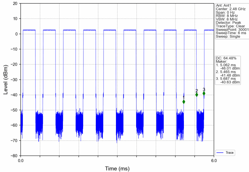
1M_HCH_2480MHz_Ant1_NTNV
