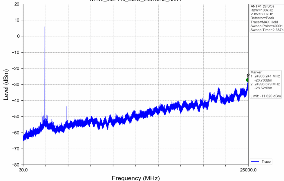
Unwanted Emissions in Non-restricted Frequency Bands NTNV_802.11b_SISO_2437MHz_ANT1
