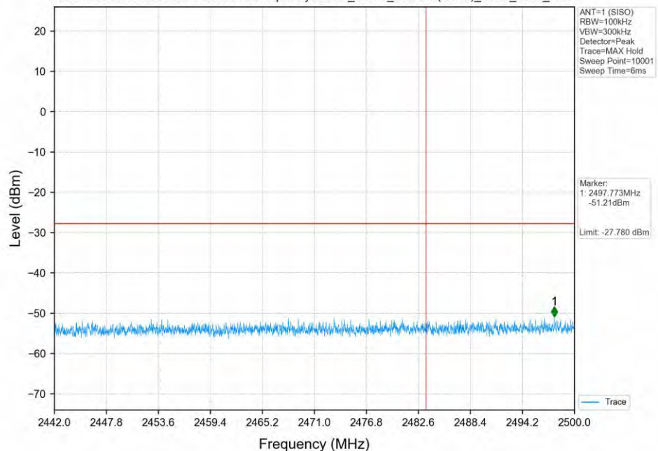
Unwanted Emissions in Non-restricted Frequency Bands_NTNV_802.11n(HT20)_SISO_2462_ANT1
