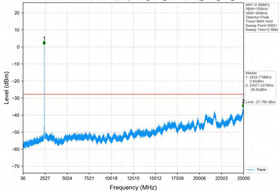
Unwanted Emissions in Non-restricted Frequency Bands_NTNV_802.11n(HT20)_MIMO_2437_ANT2
