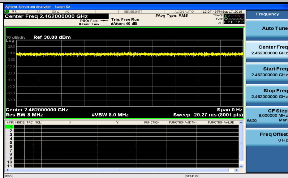
Duty Cycle_11G_2462_Ant1
