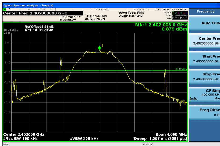
RF Conducted Spurious Emissions_BLE_2402
