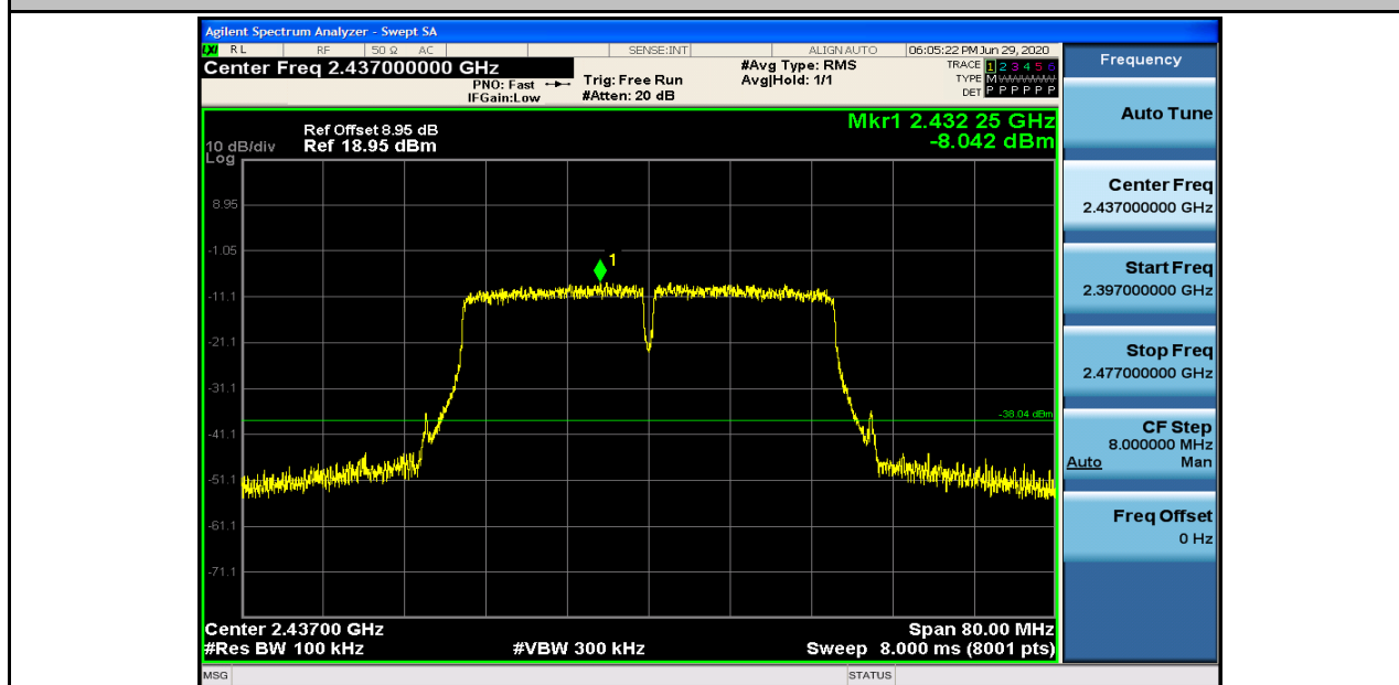
RF Conducted Spurious Emissions_11N40SISO_2437_Ant2
