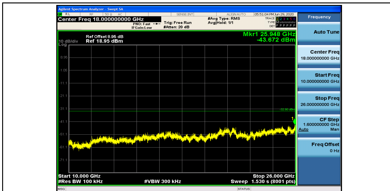
RF Conducted Spurious Emissions_11N20SISO_2462_Ant2
