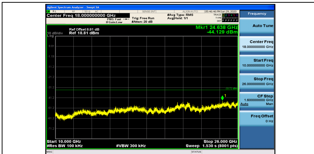
RF Conducted Spurious Emissions_11N20SISO_2437_Ant2
