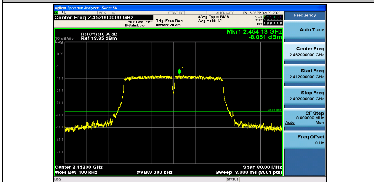
RF Conducted Spurious Emissions_11N40SISO_2452_Ant2
