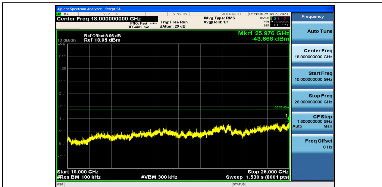
RF Conducted Spurious Emissions_11N40SISO_2422_Ant2
