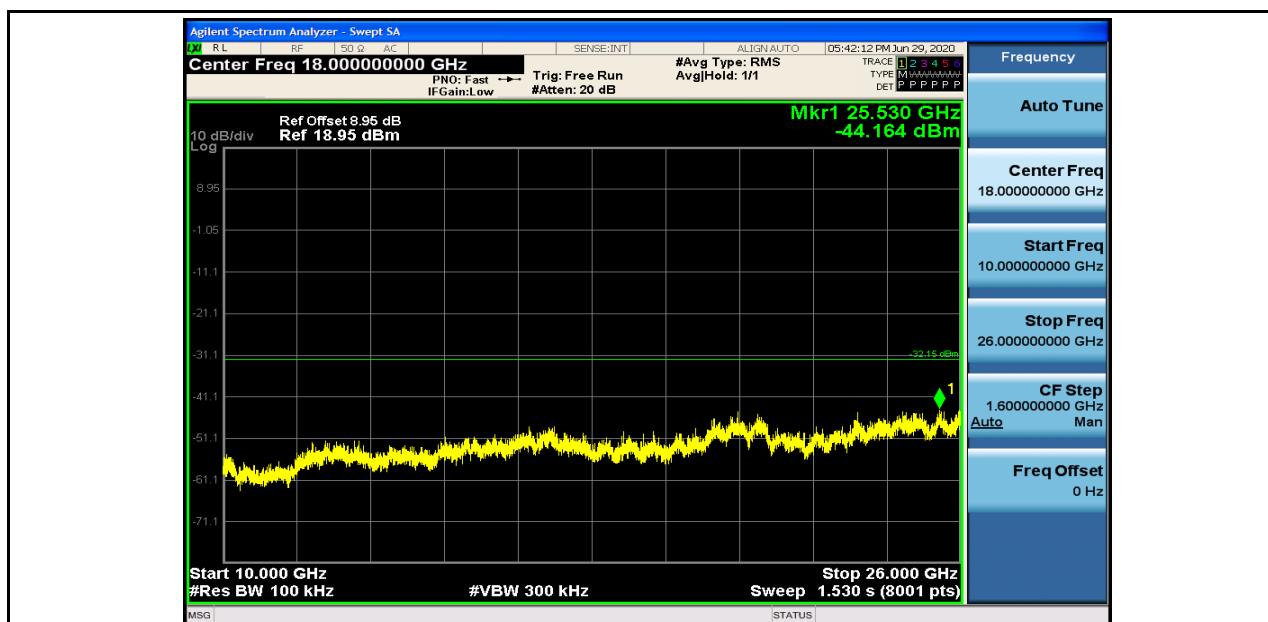
RF Conducted Spurious Emissions_11N20SISO_2412_Ant2
