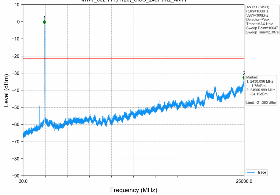
Unwanted Emissions in Non-restricted Frequency Bands NTNV_802.11n(HT20)_SISO_2437MHz_ANT1
