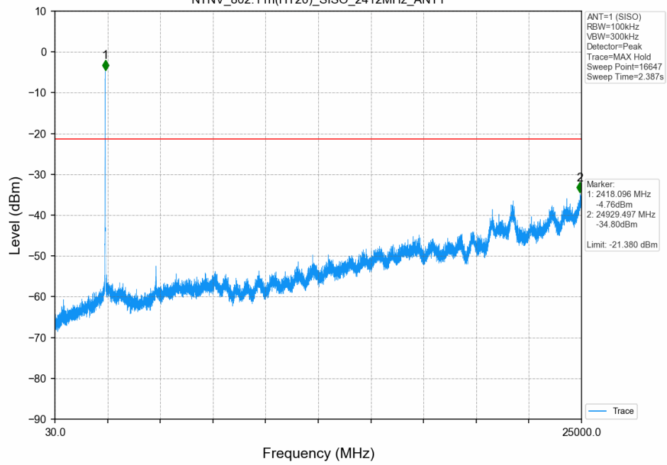
Unwanted Emissions in Non-restricted Frequency Bands NTNV_802.11n(HT20)_SISO_2412MHz_ANT1
