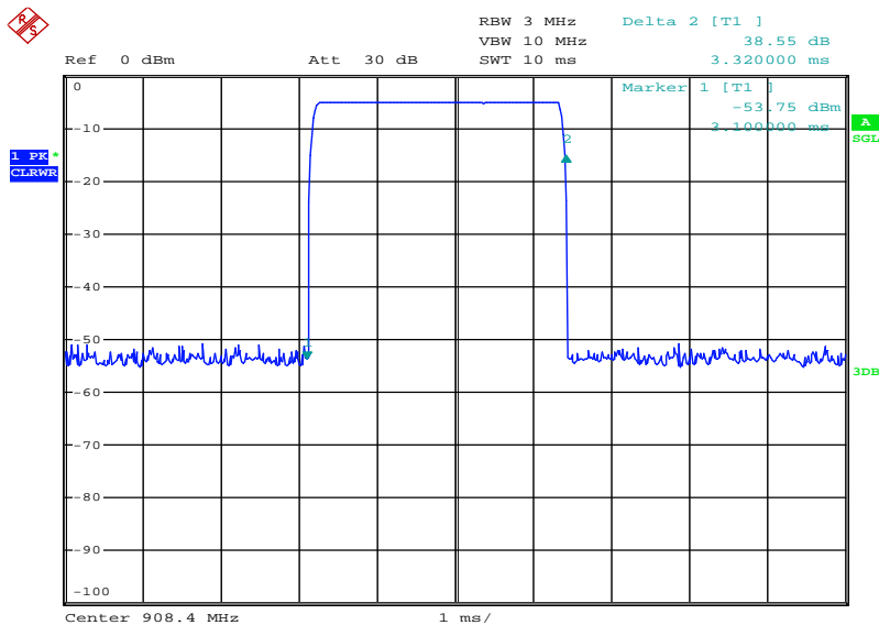
Plot 1: Time slot length = 3.32 ms
