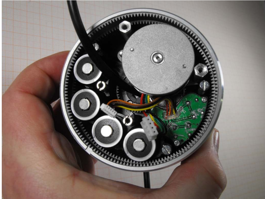
Photo 1: Gear unit
