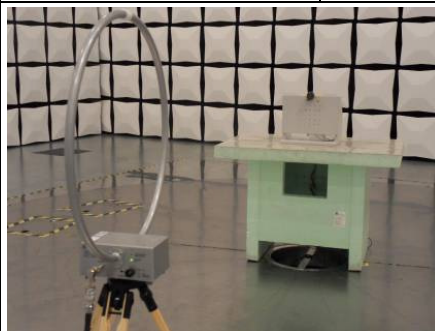
Figure 7: Measurement of field strength [Messung der Feldstärke]
